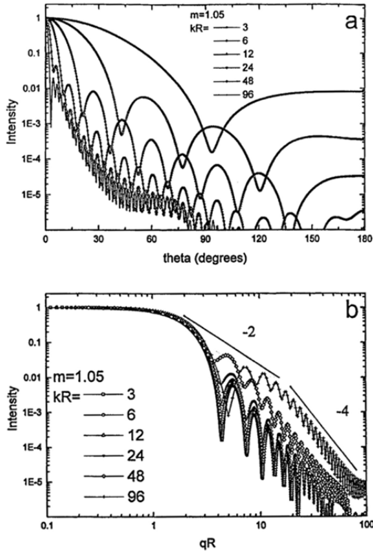
Figure 3. (a) Normalized Mie scattering curves as a function of scattering angle for spheres of refractive index m = 1.05 and a variety of size parameters; and (b) same as (a) but plotted logarithmically vs. qR . Lines with slope -2 and -4 are shown [1].
