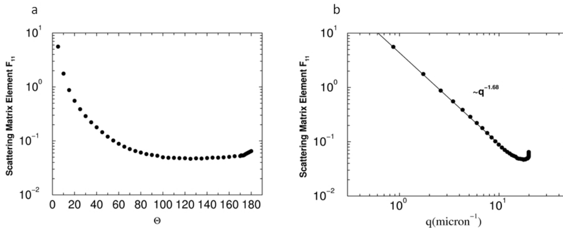
Figure 11. The scattered intensity (scattering matrix element F_{11} ) for Saharan (JGR 112 [34]) dusts versus (a) scattering angle \theta , and (b) The scattering wave vector q .
