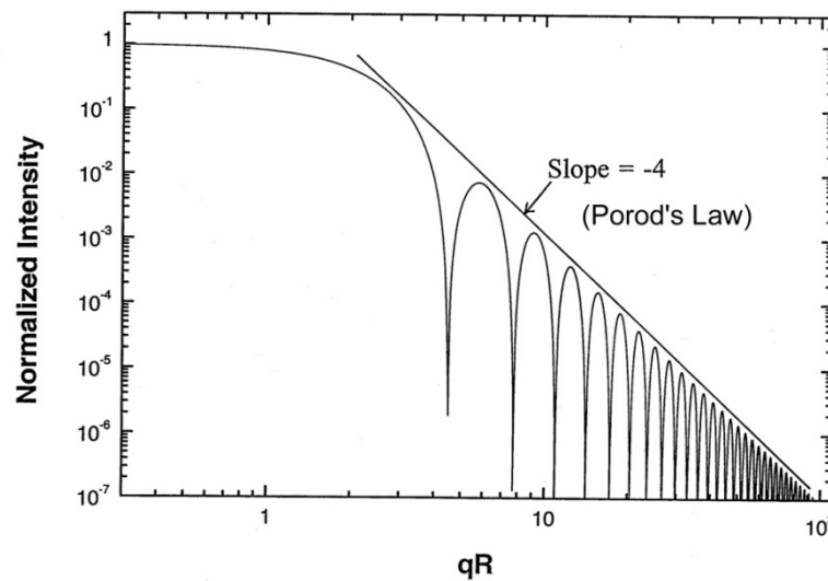
Figure 2. Plot of the structure factor for scattering from a sphere in the Rayleigh-Debye-Gans limit.
