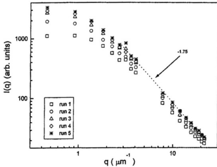
Figure 10. Scattered intensity as a function of the wave vector q for a \text{TiO}_2 aerosol. The slope in the large q regime for this log-log plot is the fractal dimension D_f=1.75 . Five sets of data represent five consecutive runs as aggregation ensued.
