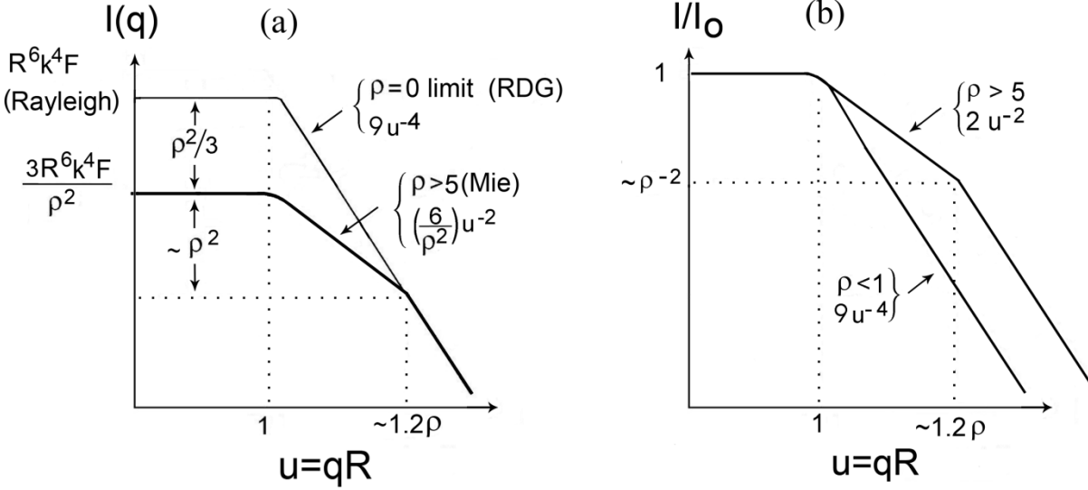
Figure 8. Diagrams of the general description of Mie scattering, the Mie scattering patterns, for uniform spheres of arbitrary size and real refractive index.
