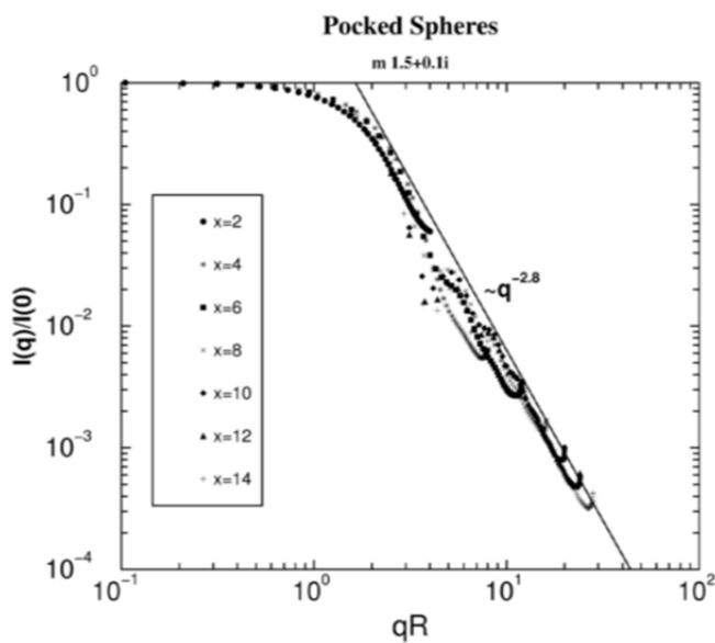
Figure 12. Normalized scattering intensity calculated for pocked spheres of various size parameters, x = kR .
