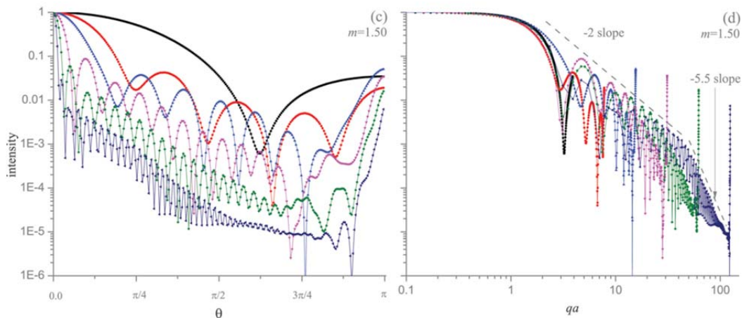
Figure 9. Scattered intensity for strongly refractive prolate spheroids with an aspect ratio of 0.8 and size parameters ka , where a is the major axis of the spheroid, ranging from 1.94 to 62.2. The incident illumination is parallel to the major axis. On the left the normalized intensity is plotted versus the scattering angle, on the right plotted versus the log of qa .
