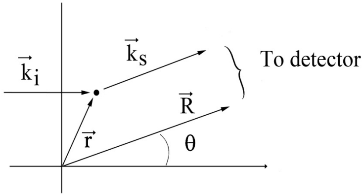
Figure 1. Diagram of light with an incident wave vector \vec{k}_i scattering from a point scatterer at \vec{r} into the scattering wave vector \vec{k}_s at an angle \theta directed to a distant detector.
