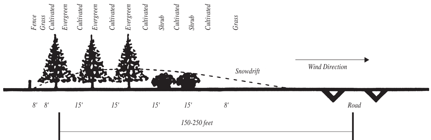
Figure 1. Living snowfence.
