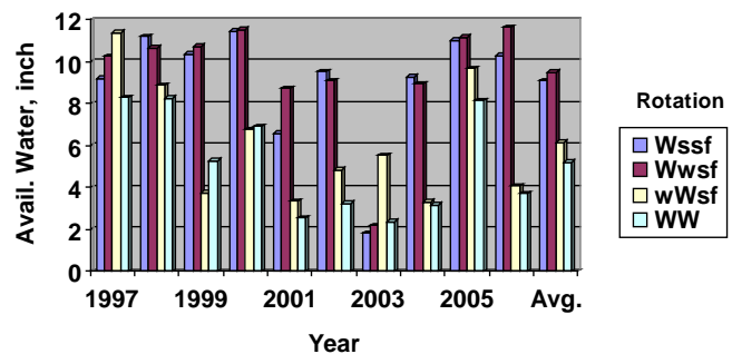
Figure 1. Available soil water at planting of wheat in several rotations, 1997-2006, Tribune, KS. Letter capitalized denotes current crop in rotation.
