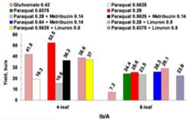
Fig 3. Control of glyphosate-resistant corn in Garden City.
