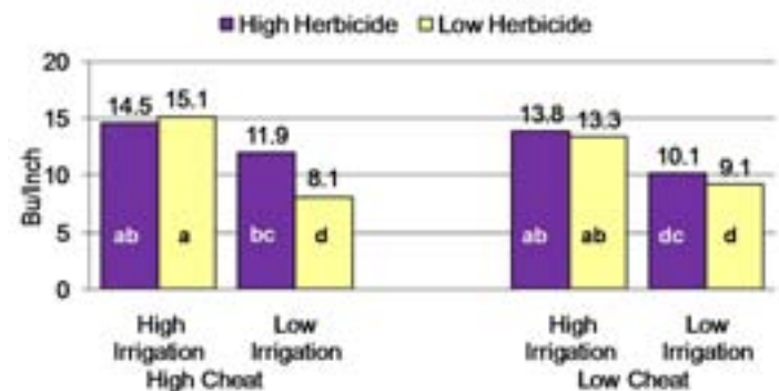
Fig. 6. WUE of irrigation water only at location 2 in 2006.
