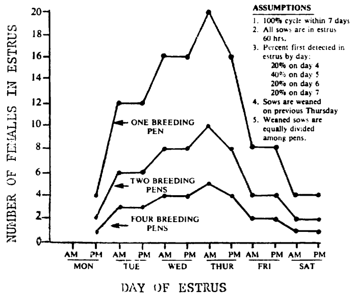
Figure 4. Number of sows in estrus on each day when pen-mated in one, two, or four breeding pens (20 weaned sows).
