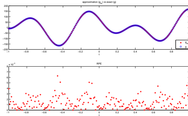
Figure 4: A reconstruction of the continuous part g(x) (above) of Example 3 with \epsilon = 10^{-6} , and the corresponding Relative Pointwise Errors (RPE) (below)
