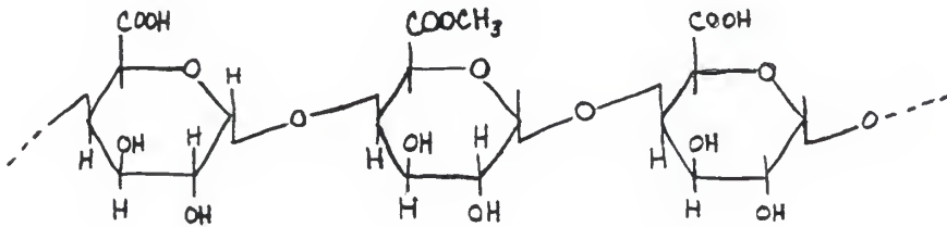
FIGURE 6: PECTIC SUBSTANCE CHAIN FRAGMENT (PECTIN)
