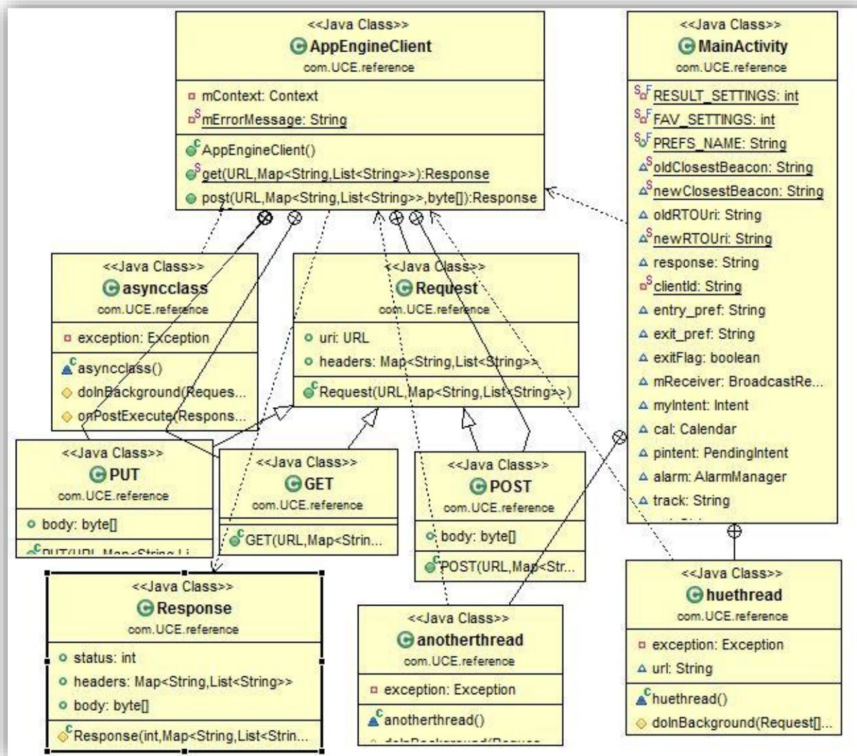
Figure 4-5 Class Diagram 2
