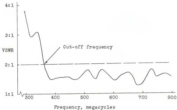
Fig. 5(b). VSWR for Archimedes scimitar, r = k\theta .
