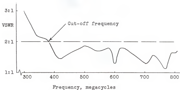
Fig. 5(a). VSWR for equiangular scimitar, r = ae^{k\theta} .
