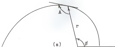
(a) Equiangular or logarithmic spiral. r = ae^{k\phi} .
