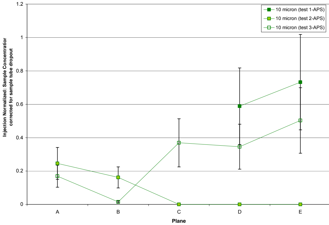
Figure 5-7: Injection normalized sample concentrations at location 3.
