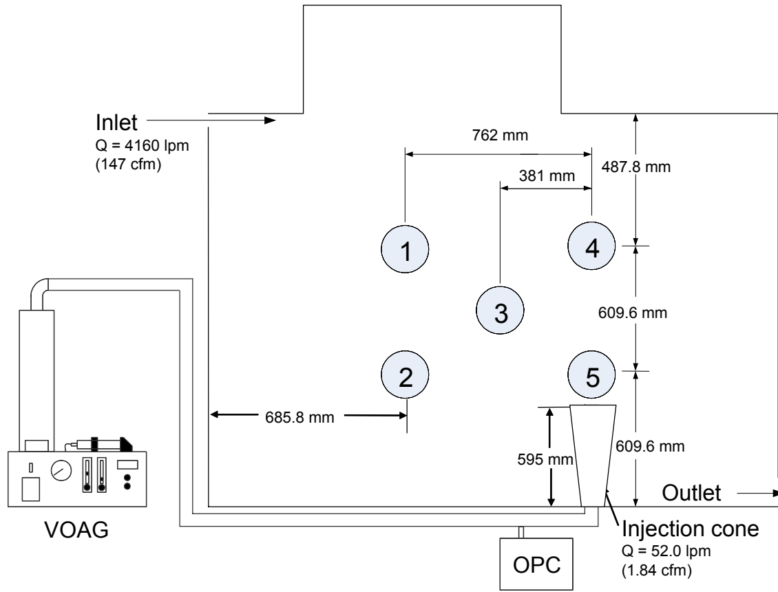
Figure 4-2: Test cabin measurement locations ( z=0 ) with injection cone (front view).
