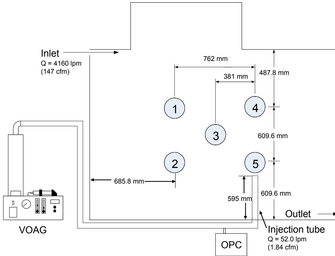
Figure 3-5: Schematic of injection setup relative to the test cabin and sampling locations.
