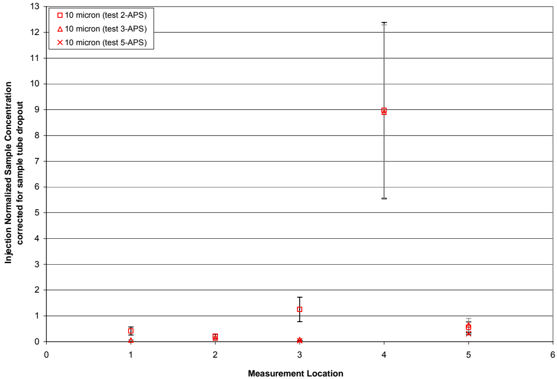
Figure 5-2: Injection normalized concentration for ten micron particles.
