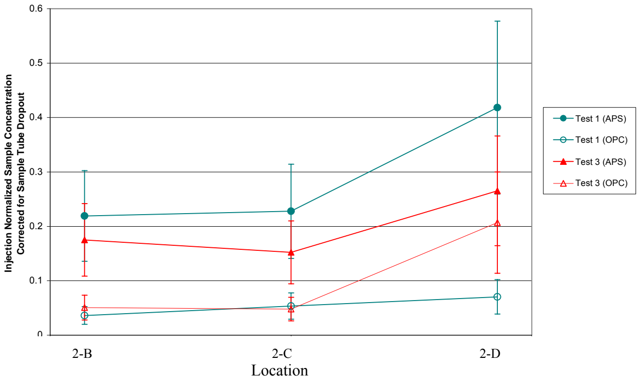
Figure 7-8: Injection normalized sample concentration for side-by-side APS to OPC comparison tests for ten micron particles (test 1 and test 3).
