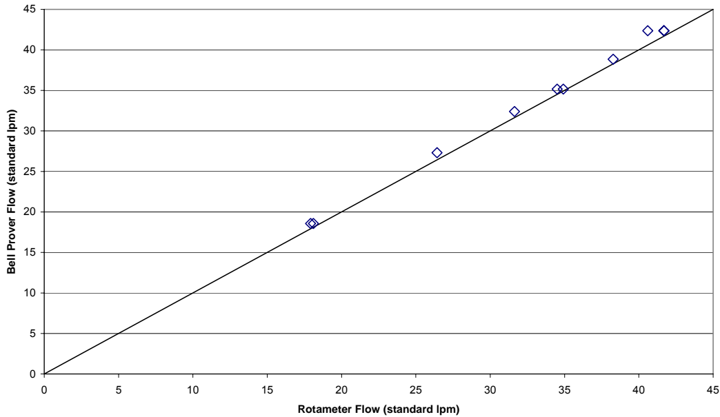
Figure 7-12: Rotameter calibration.
