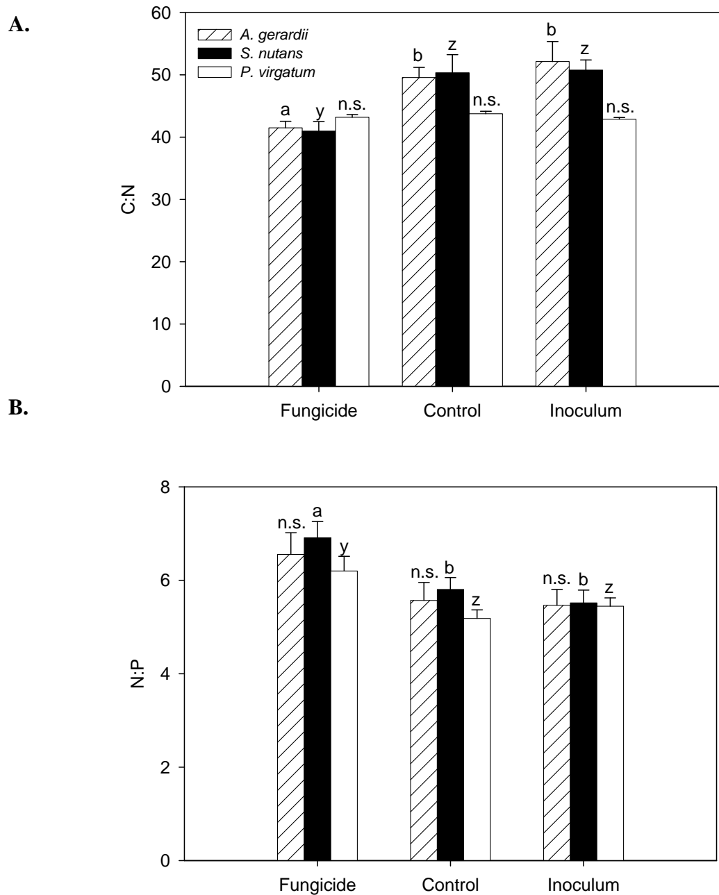
Figure 4-5. Mean ( \pm SE) values for indices of leaf tissue chemistry, including A) C:N ratio and B) N:P ratio for samples collected in 2007 of Andropogon gerardii , Sorghastrum nutans , and Panicum virgatum . Treatments included fungicide, control, and inoculum addition (n=6 for each treatment). Means accompanied by the same letter or designated with “n.s.” were not significantly different ( \alpha = 0.05 ).
