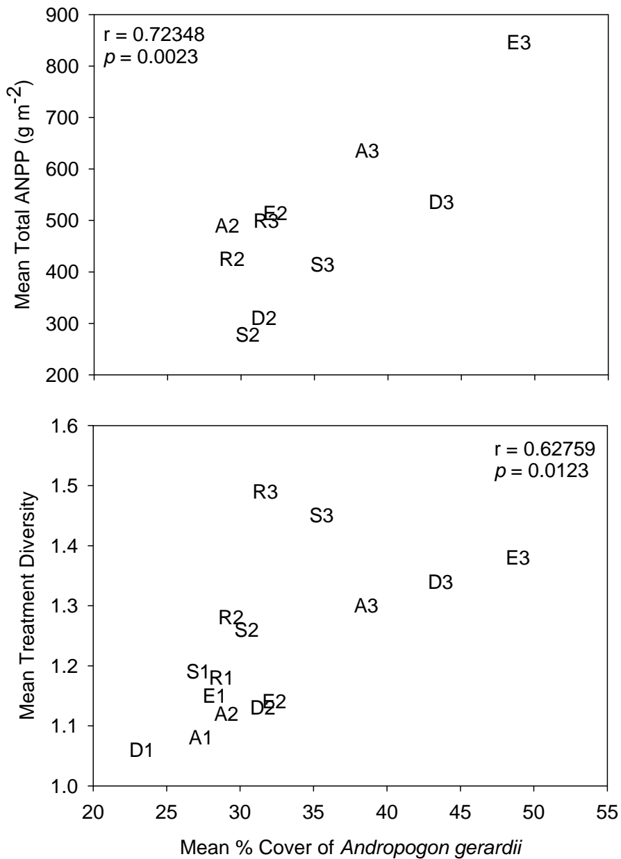
Figure 3-7. Correlations between mean % cover of Andropogon gerardii and mean total ANPP excluding litter (g m -2 ) (top panel) and mean treatment diversity (Shannon diversity) (bottom panel) by year. All plots and years were included in the analyses, except for ANPP in 2005 due to lack of pre-mowing biomass sampling. Labels represent treatment (S = shallow soil, D = deep soil, R = reduced-N, A = ambient-N, and E = enriched-N) and year (1 = 2005, 2 = 2006, and 3 = 2007). Significant relationships were determined from the Pearson correlation coefficient ( r ) derived from SAS (SAS 2002-2003).
