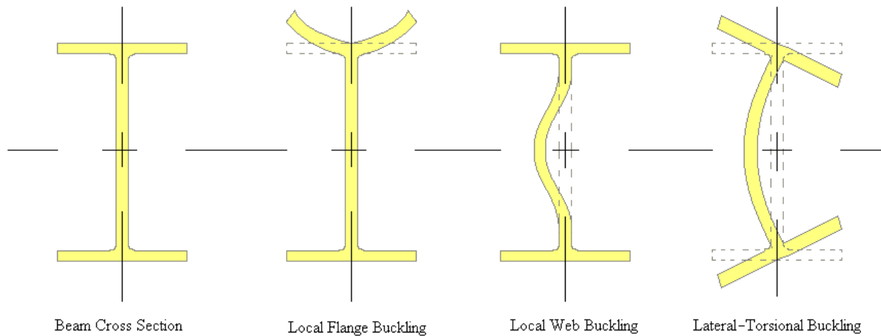
Figure 5-4 Buckling Examples
