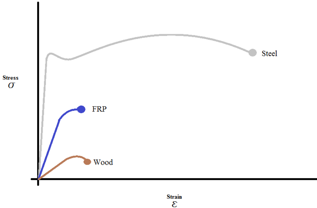
Figure 4-4 Stress-Strain Curve Comparisons
