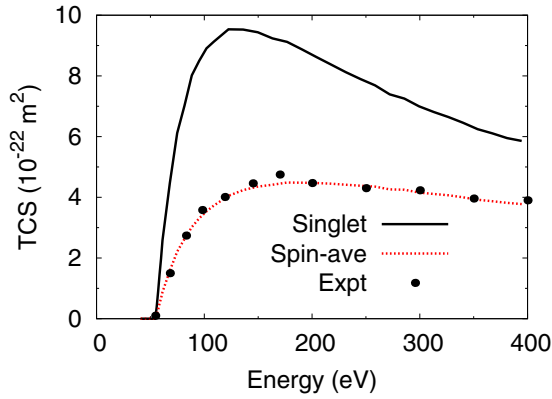
FIG. 2. (Color online) Total cross sections for electron impact ionization of \text{He}^+ in the ground state. Results are shown for the singlet spin channel alone and for the spin-averaged cross section. The latter predictions are compared with the experimental data of Peart et al. [56].
