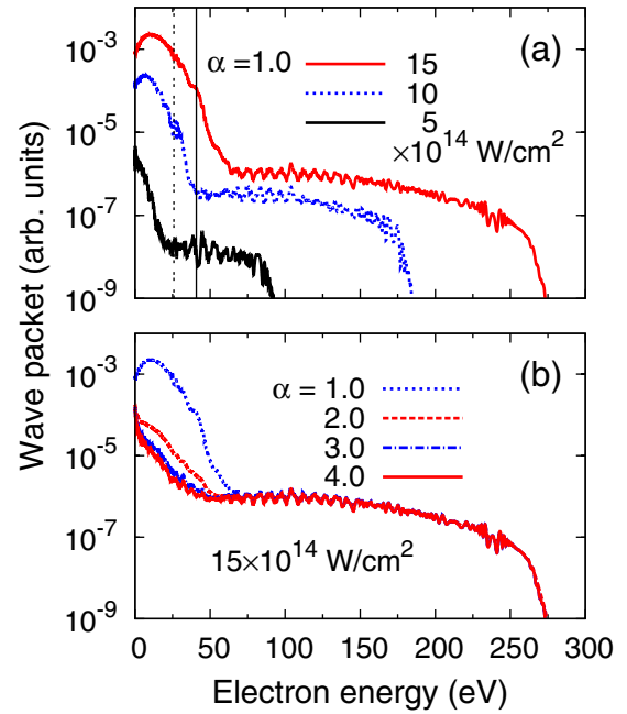
FIG. 5. (Color online) Returning electron wave packets for He in linearly polarized laser pulses at 780 nm. (a) The screening factor is chosen as \alpha = 1.0 , and the peak intensities are 5 , 10 , and 15 \times 10^{14} \text{ W/cm}^2 , respectively; (b) The peak intensity is 15 \times 10^{14} \text{ W/cm}^2 and the screening factors are \alpha = 1.0, 2.0, 3.0 , and 4.0 , respectively. The calculations include integration over the laser focus volume. In (a), the vertical solid line marks the excitation threshold of \text{He}^+ in the field-free case, while the vertical dotted line marks the corresponding threshold for excitation in the field at a peak intensity of 15 \times 10^{14} \text{ W/cm}^2 .
