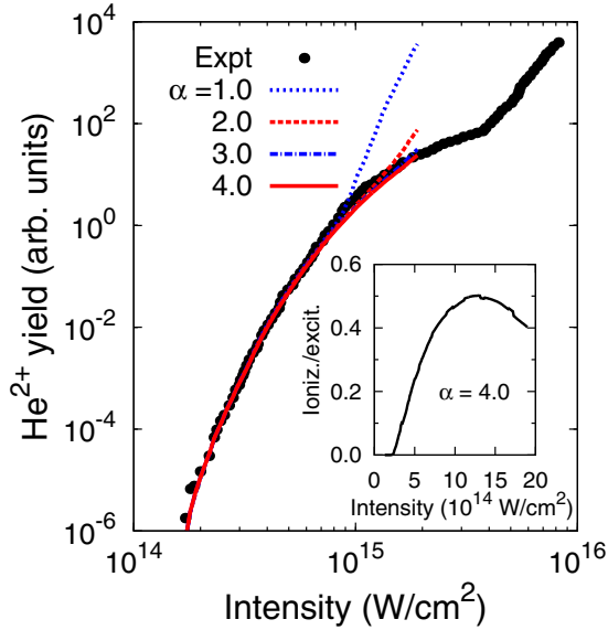
FIG. 6. (Color online) Comparison of the simulated results, with the shift of the continuum threshold energy taken into account, for the yields of doubly charged ions with the experimental data for He in linearly polarized laser pulses at 780 nm. The solid circles represent the measurements of Walker et al. [4], while the lines are simulated results for \alpha = 1.0, 2.0, 3.0, and 4.0 , respectively. The theoretical predictions are relative and were normalized to the experimental data at the peak intensity of 4.5 \times 10^{14} W/cm 2 with a fixed factor for each screening factor. The inset shows the ratio of the contributions to double ionization from ionization and excitation.
