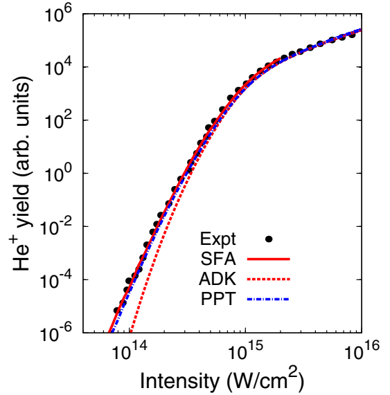
FIG. 7. (Color online) Comparison of theoretical simulations based on SFA, ADK, and PPT with the experimental data for single ionization of He in linearly polarized laser pulses at 780 nm. The solid circles represent the measurements of Walker et al. [4]. The theoretical results are normalized individually for the best visual agreement with experiment.
