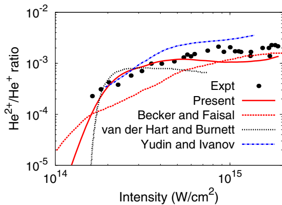
FIG. 9. (Color online) Ratio between double and single ionization of He as a function of intensity for a 160-fs pulse with a wavelength of 780 nm. The present simulations are compared with the experimental data of Walker et al. [4], as well as other theoretical results of Becker and Faisal [21], van der Hart and Burnett [39], and Yudin and Ivanov [40].
