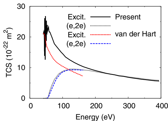
FIG. 3. (Color online) Comparison of the present BRS singlet TCSs for electron impact ionization and excitation of \text{He}^+ in the ground state with the corresponding results of van der Hart [38].
