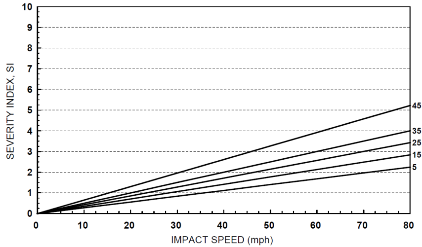
Figure 1.10: Relationship between Severity Index and Impact Speed (Wolford & Sicking, 1997)
