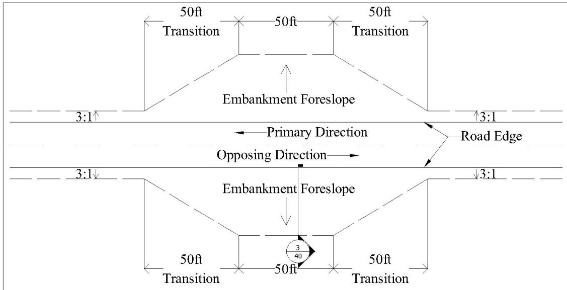
Figure 45.32: Plan View of Embankment on Three- or Four-Wheel-Track Gravel or Paved Road
