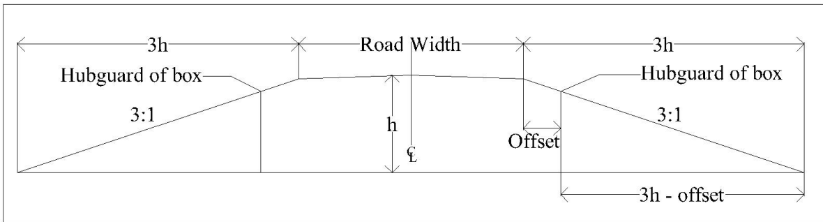
Figure 40.27: Cross Section of Culvert
