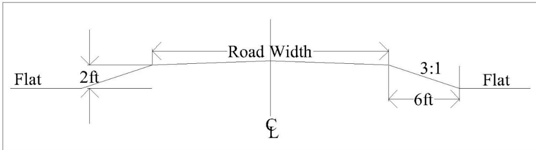
Figure 37.24: Cross Section Before and After Transition
