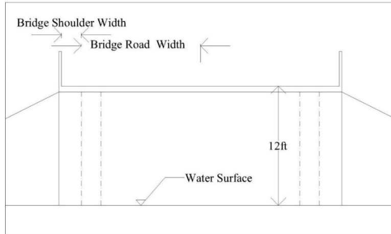
Figure 49.36: Bridge Cross Section for Three- or Four-Wheel-Track Gravel or Paved Road
