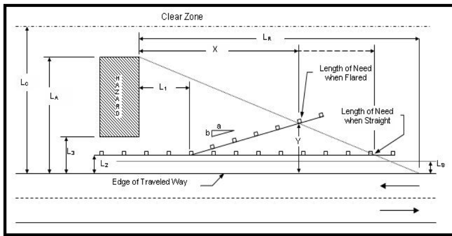
Figure 1.8: Guardrail Length for Approaching Traffic (AASHTO, 2011)
