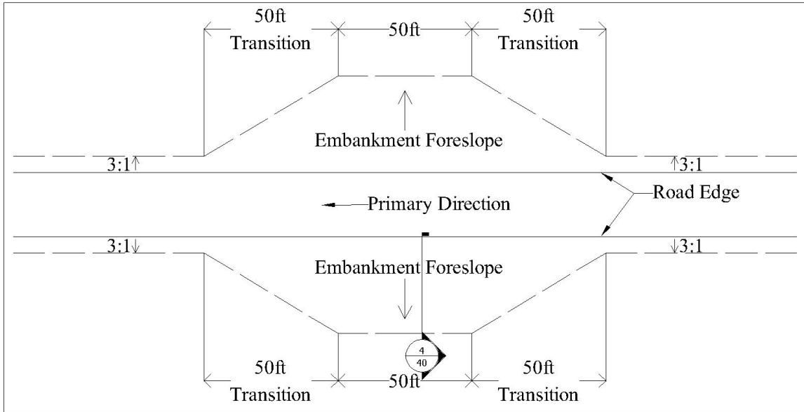
Figure 44.31: Plan View of Embankment on Two-Wheel-Track Gravel Road
