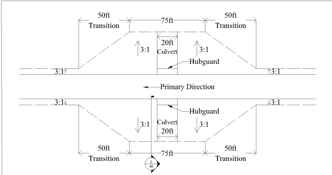
Figure 38.25: Plan View for Culvert on Two-Wheel-Track Gravel Road
