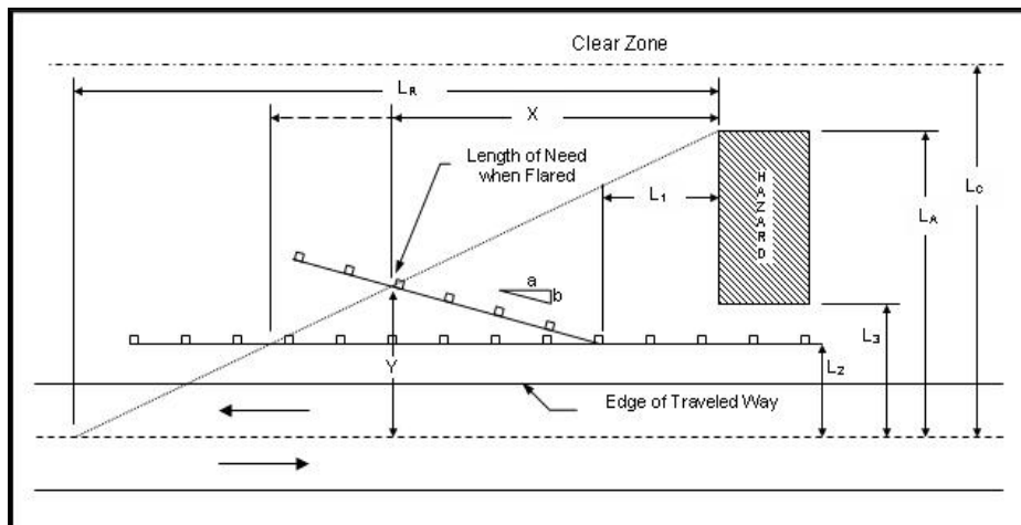
Figure 1.9: Guardrail Length for Opposite Traffic (AASHTO, 2011)
