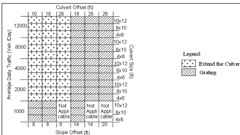
Figure 1.13: Decision Matrix of Safety Treatment for Culverts (Albuquerque et al., 2011)
