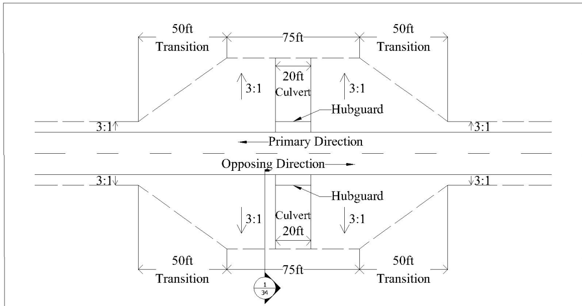
Figure 39.26 Plan View of Culvert on Three- or Four-Wheel-Track Gravel or Paved Road
