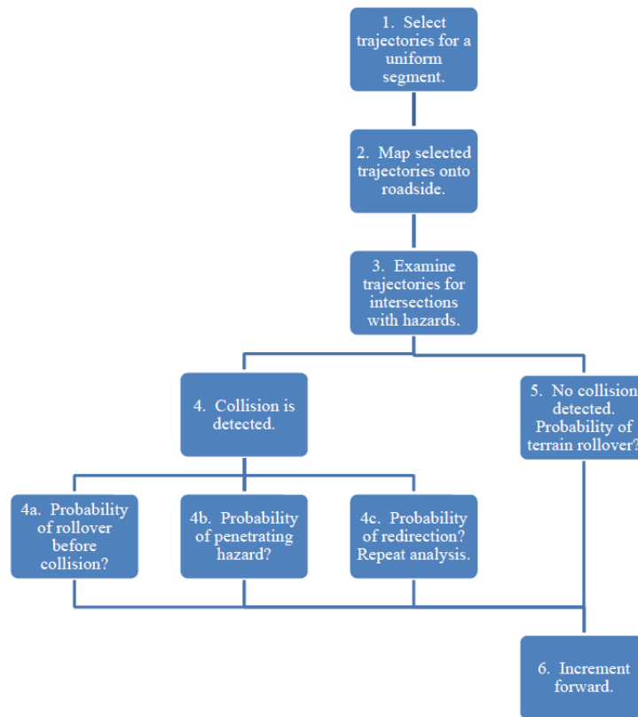
Figure 33.20: RSAPv3 Crash Prediction Module Flowchart (RSAPv3 Engineer’s Manual)
