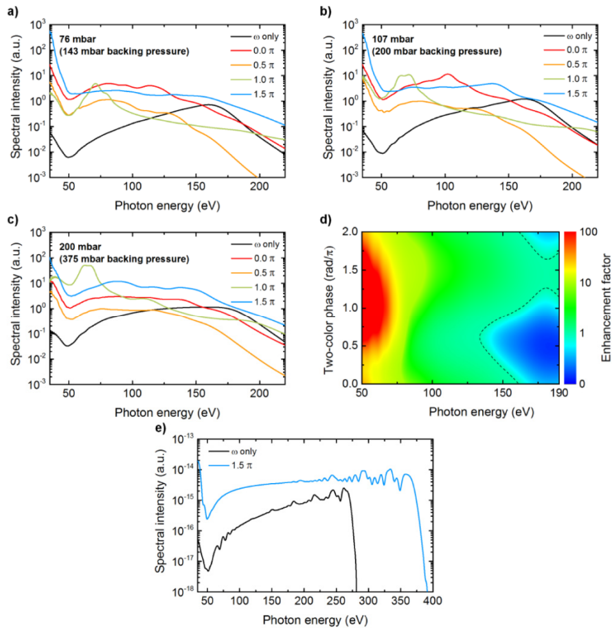
Fig. 6. Simulated HHG spectra depending on pressure and two-color phase. Experimental backing pressures (given in brackets) are specified along with the corresponding pressure at the interaction region. (a) – (c) show the two-color driven HHG spectra and the single-color driven spectrum (black). The simulated HHG enhancement factors for 200 mbar (backing pressure of 375 mbar), taking the spectrometer resolution and experimental jitter ( \approx 400 as) in the two-color phase (via smoothing along the energy and phase-axis using Gaussians of the corresponding widths) into account, are shown in (d). The color bar saturates at a factor of 100, as the region around the Cooper minimum ( \approx 50 eV) is hard to quantitatively model. The dashed line indicates where the enhancement factor drops below a value of 1, meaning the two-color-driven HHG yield is lower than the single-color-driven case. (e) Smoothed simulated single-atom HHG spectra for both the single-color-driven ( \omega only) and the optimal two-color-driven case using the laser intensities at the focus for vacuum.
