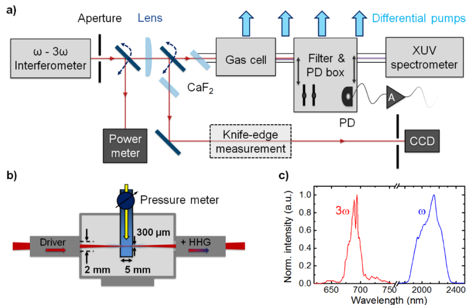
Fig. 1. (a) Experimental layout of the HHG chamber and detection systems. A CaF 2 lens focuses the output of the Michelson-type, two-color interferometer into the gas cell [shown in detail in (b)] and HHG beamline. Different combinations of filters and EUV/SXR PDs, connected to an electronic amplifier (A), or an XUV spectrometer can be used to characterize the generated high harmonics. Flippable mirrors can send the beam to a power meter or other characterization units such as a CCD camera or traveling-knife-edge stage as well as FWM in air (not shown) to optimize the temporal overlap of the two pulses. (b) Layout of the custom gas cell in the HHG beamline. The driving field enters the cell from the left and interacts with the target gas (gas flow indicated by the yellow arrow) at adjustable pressure in the gas capillary (blue). (c) Normalized spectra of both \omega (blue) and 3\omega (red) pulse.
