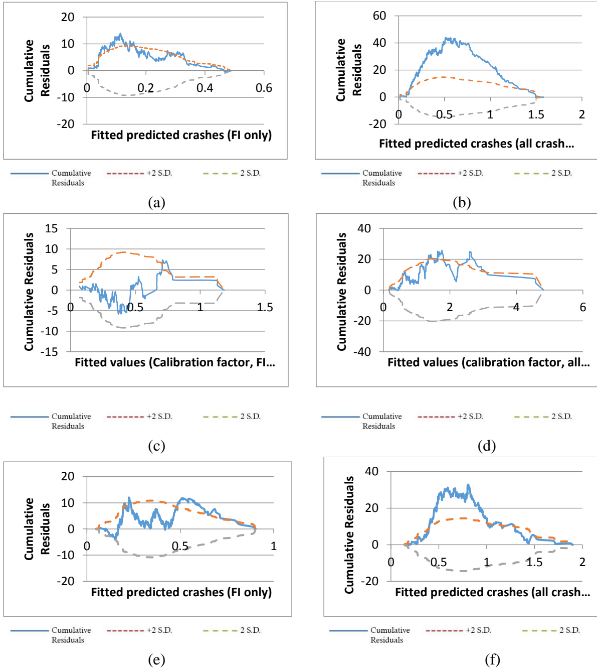
Figure D-1: CURE plots for fitted values estimated using calibration factors for: (a) 3SG, FI, (b) 3SG, all crashes, (c) 3ST, FI, (d) 3ST, all crashes, (e) 4ST, FI, and (f) 4ST, all crashes.
