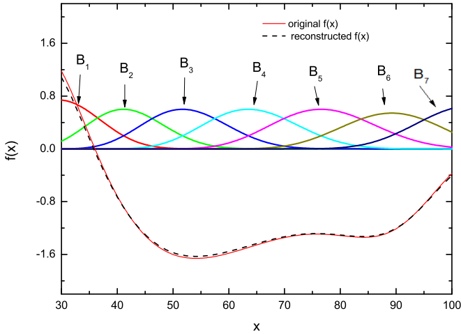
FIG. 1. Illustration of expanding a smooth function in terms of B -spline basis functions. The input function (red solid line) is compared with the reconstructed one (black dashed line). Seven B -spline functions with the order of five are used in the reconstruction.
