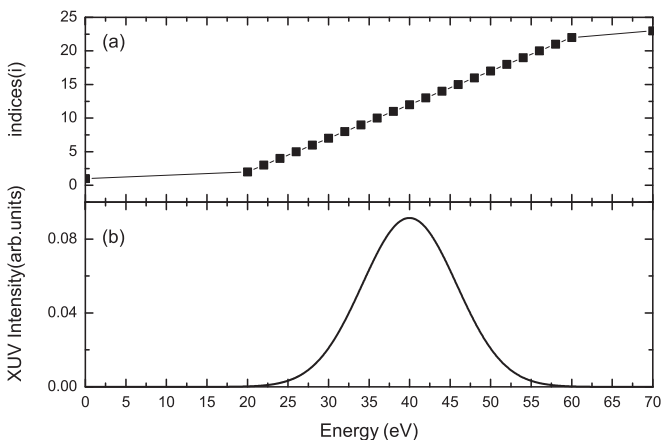
FIG. 2. The scheme that shows how we optimize the distribution of the knot points (a) for XUV phase based on the spectral amplitude of the (b) XUV pulse.
