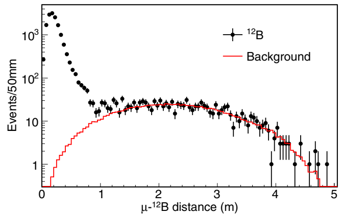
FIG. 2. Distance between selected ^{12}\text{B} events and preceding stopped muon (black), as compared to a background sample (red). The efficiency for a distance cut is the fraction of background-subtracted ^{12}\text{B} within the cut.
