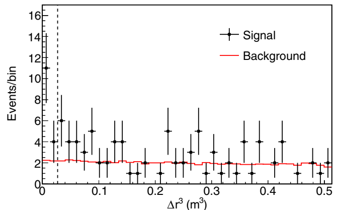
FIG. 3. The distance-cubed distribution of \beta n events less than 0.4 s after a stopping muon with all other cuts applied. The dashed line is the \Delta r cut.
