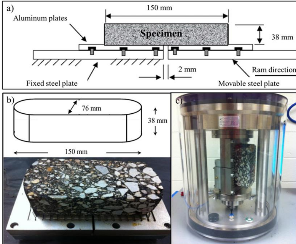
Figure 4-6 OT test setup: a) load configuration, b) sample dimensions, c) AMPT setup
