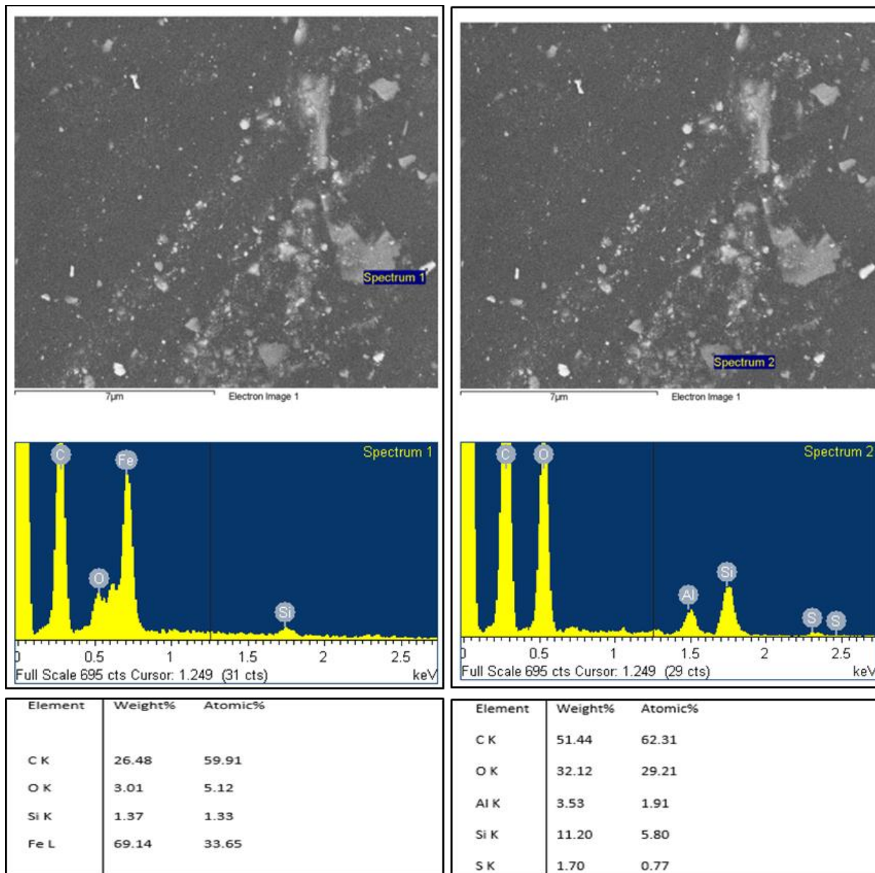
Figure 4-12 EDXS analysis of two spots on the binder extracted from US-59 mixture
