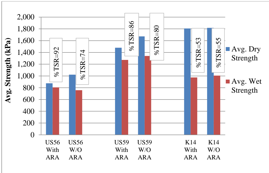
Figure 5-2 Average TSR results for wet and dry samples
