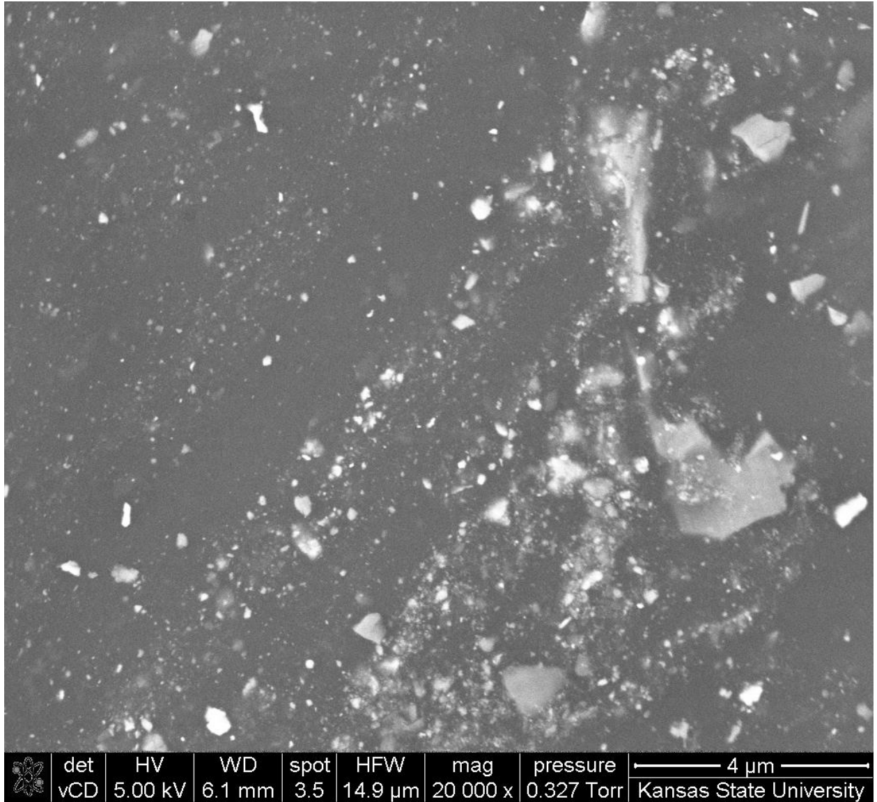
Figure 4-11 SEM image of US-59 extracted binder
