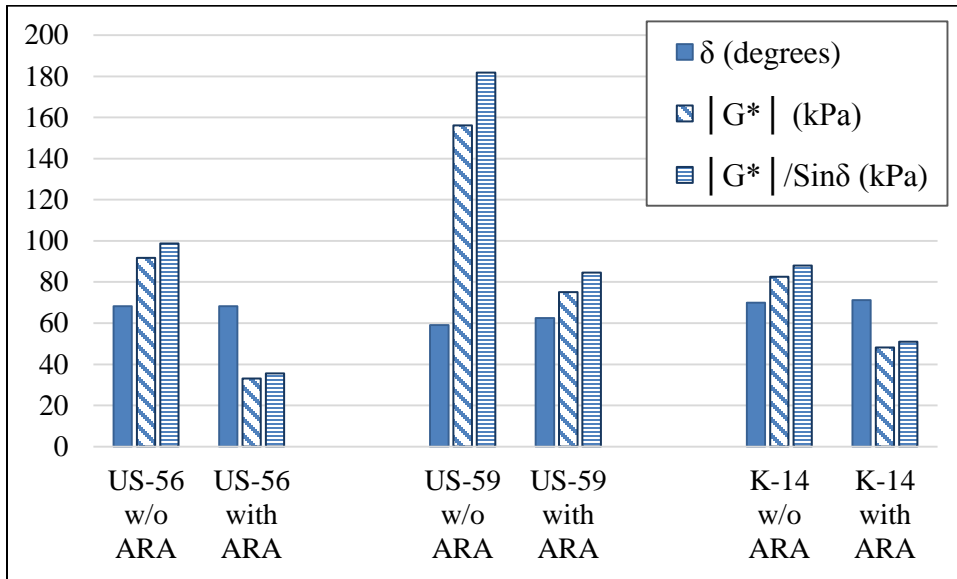
Figure 3-4 DSR test results at 58 °C for non-aged extracted binder of HIR mixtures
