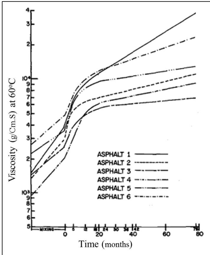
Figure 2-1 Typical changes of asphalt binder viscosity over time (Kandhal et al. 1973)
