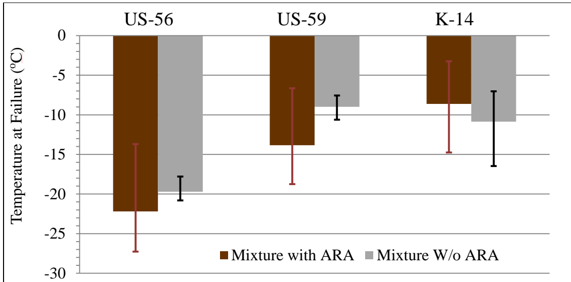
Figure 5-3 TSRST results for mixtures with and without ARA
