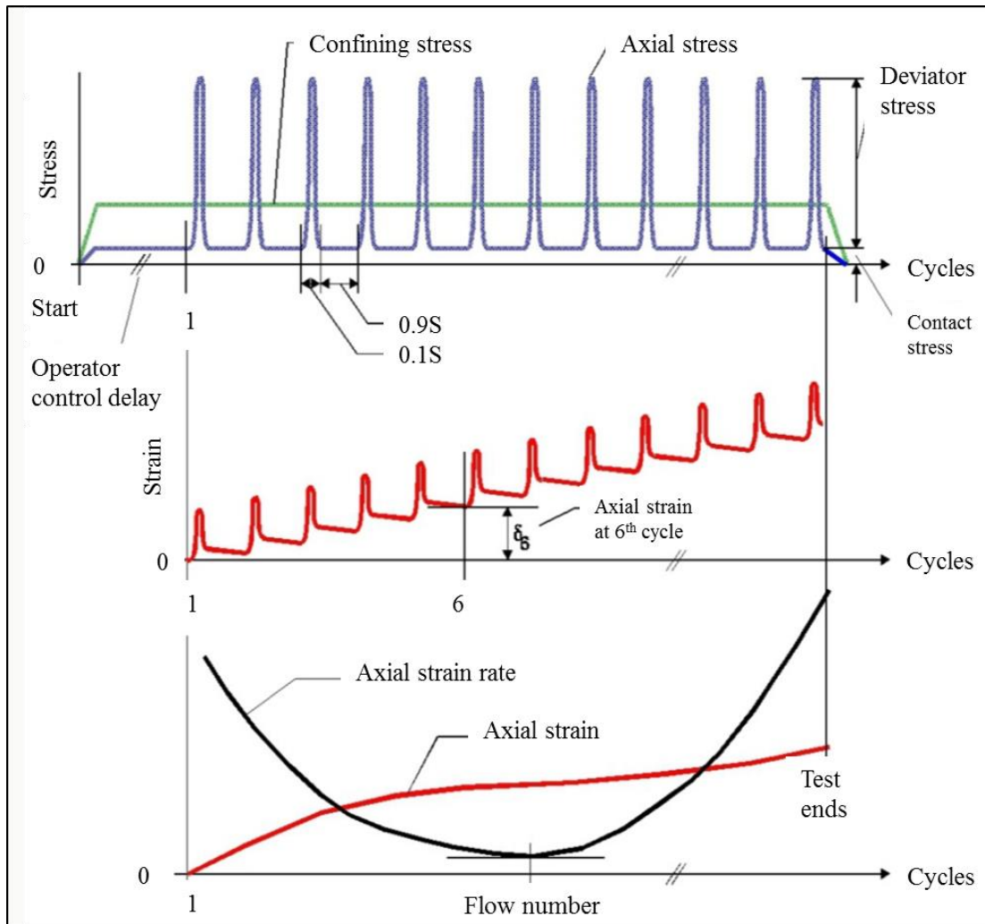
Figure 4-5 Stress application and timing in the flow number test
