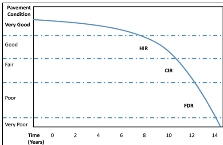
Figure 1-1 Pavement condition and applicable in-place recycling method (NCHRP 2011)
