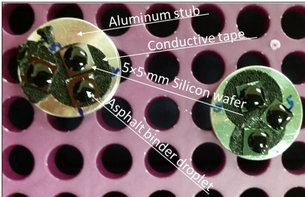
Figure 4-10 Extracted asphalt binder samples prepared for SEM
