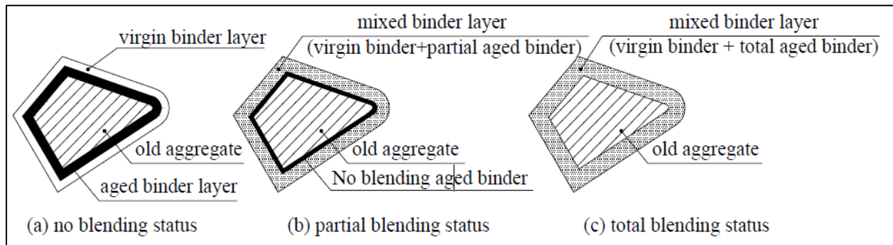
Figure 2-3 Three scenarios for blending of virgin and aged binder (Xu et al. 2014)
