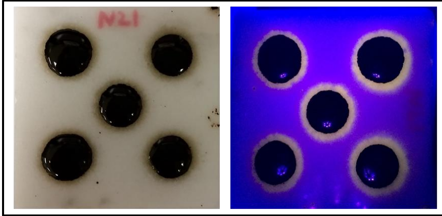
Figure 4-9 EDT samples under normal (left) and UV (right) light with clear rings around asphalt droplets
