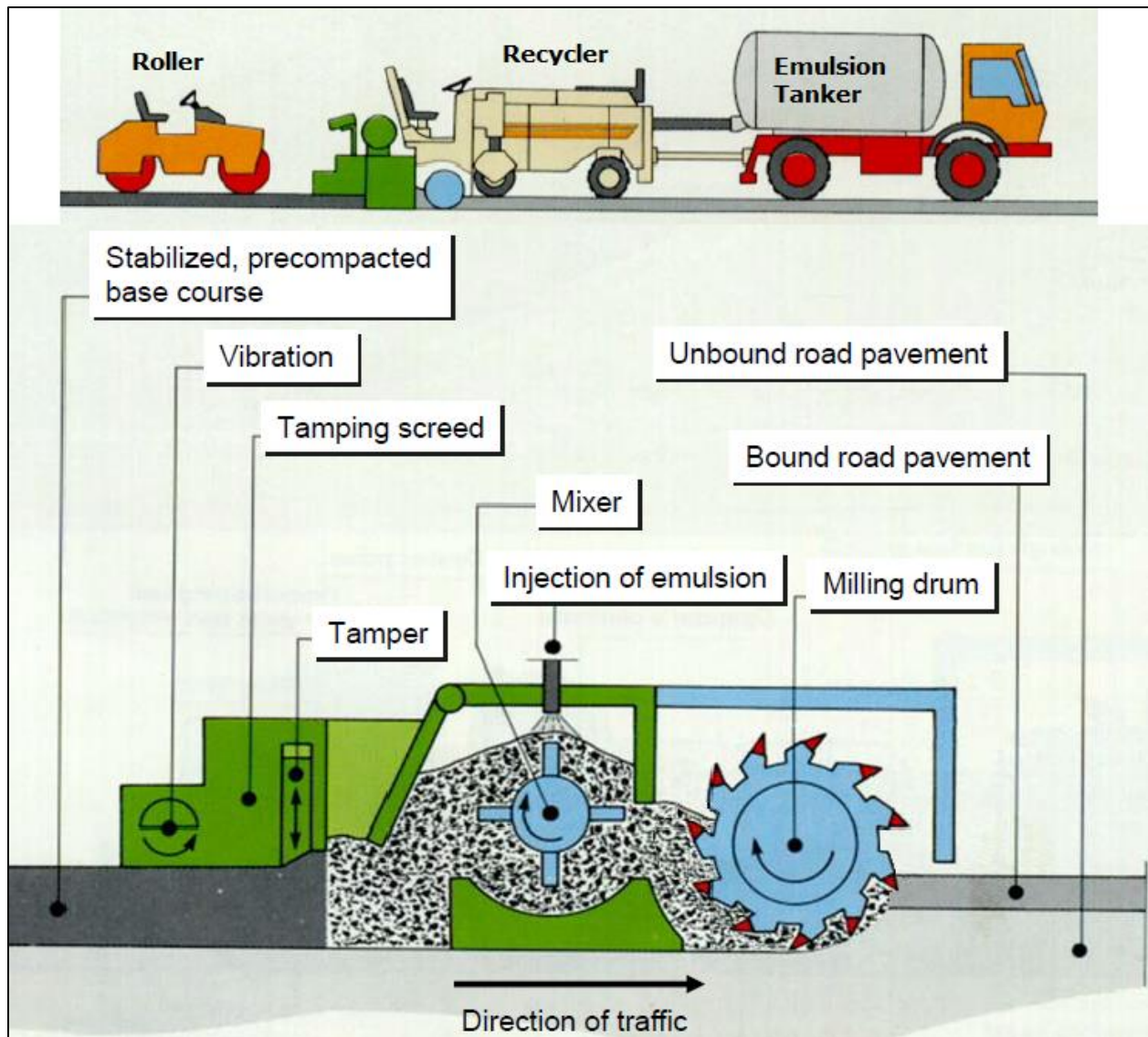
Figure 1-2 Schematic of single-unit CIR train (Kandhal and Mallick 1997)
