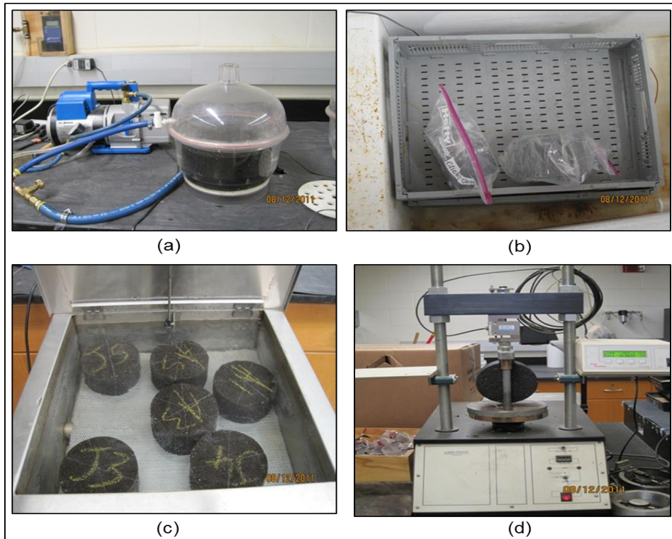
Figure 4-7 KT-56 test procedure: (a) vacuum saturation, (b) freezing (minimum of 16 hrs, (c) thawing (24 hrs in water bath at 60 °C), (d) testing tensile strength
