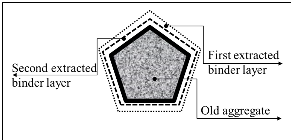
Figure 2-5 Staged extraction analogy for a single RAP aggregate (Xu et al. 2014)
