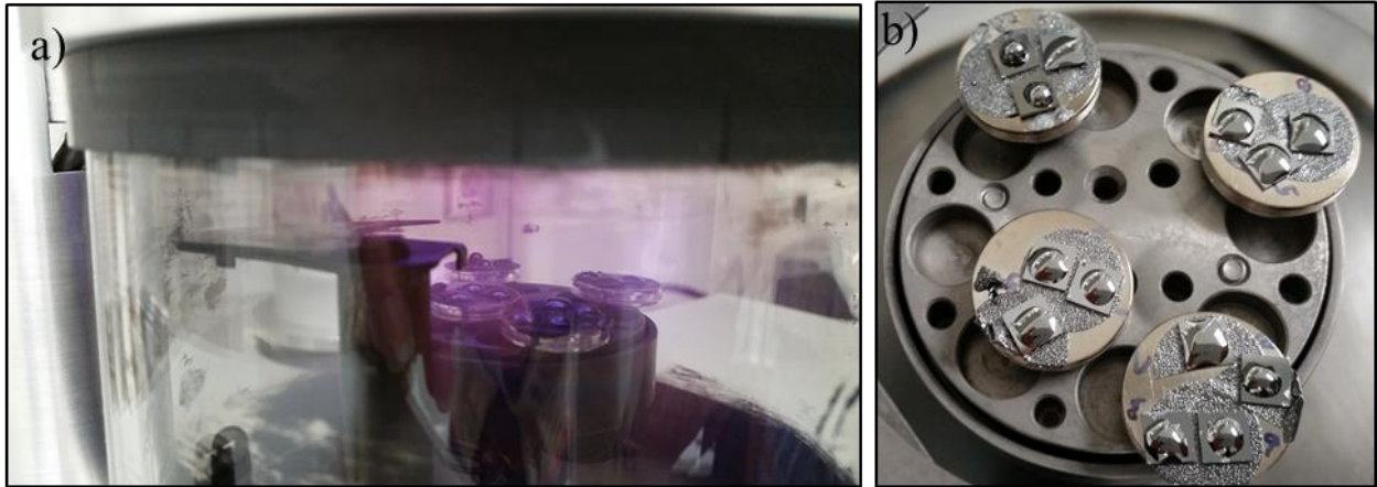
Figure 4-13 US-56 extracted binder samples: a) under Pd spray, b) coated with Pd
