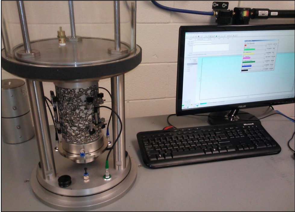
Figure 4-4 Dynamic modulus sample setup in AMPT machine with attached LVDTs
