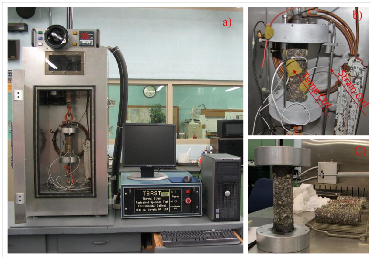
Figure 4-8 TSRST setup: a) testing equipment, b) load cell (inside the chamber), c) test sample glued to the top and bottom plates
