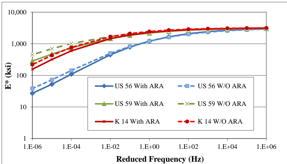
Figure 5-1 Dynamic modulus master curves for HIR mixtures with and without ARA
