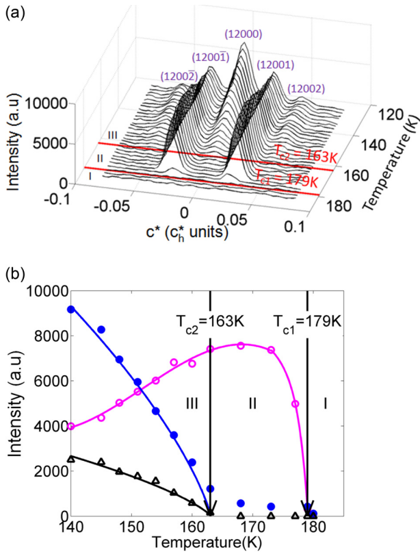
FIG. 6. (Color online) (a) Temperature evolution of the superstructure line ( h = 1, k = 2 ) measured on the mar345dtb system using Cu- K_{\alpha} radiation revealing two phase transitions at T_{c1} = 179 K and T_{c2} = 163 K. (b) Extracted temperature evolution of the averaged intensities of superstructure Bragg peaks ( hklmn ), which demonstrate that h + k + n = \text{odd} Bragg peaks characterize phase III ( n = 0 in blue filled circles, n = 2 in black triangles) and that h + k + n = \text{even} Bragg peaks characterize phase II ( n = 1 in pink circles).
