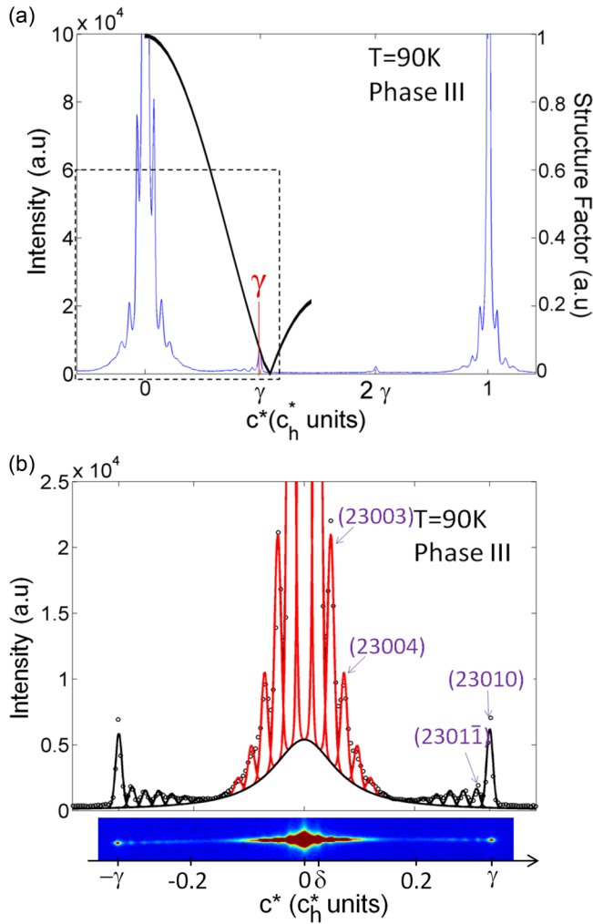
FIG. 4. (Color online) (a) n -Tetracosane/urea (230mn)_o superstructure line (in blue) measured at 90 K on the CRISTAL beamline at SOLEIL along the incommensurate direction in the q range of -0.2c_h^* to 1.2c_h^* in reciprocal urea units. Inset in black: Molecular form factor of the n -tetracosane molecule aligned along the c direction with sixfold orientational disorder, as calculated in [39]. (b) Diffraction image and extracted profile of the (230mn)_o superstructure line between -0.4c_h^* and +0.4c_h^* . Superstructure satellite Bragg peaks are associated with a modulation vector \mathbf{c}_m^* = \pm(0.025 \pm 0.001)c_h^* . Satellite peaks were fit using Gaussians and are indexed as (2300m)_o in red and (2301m)_o in black.
