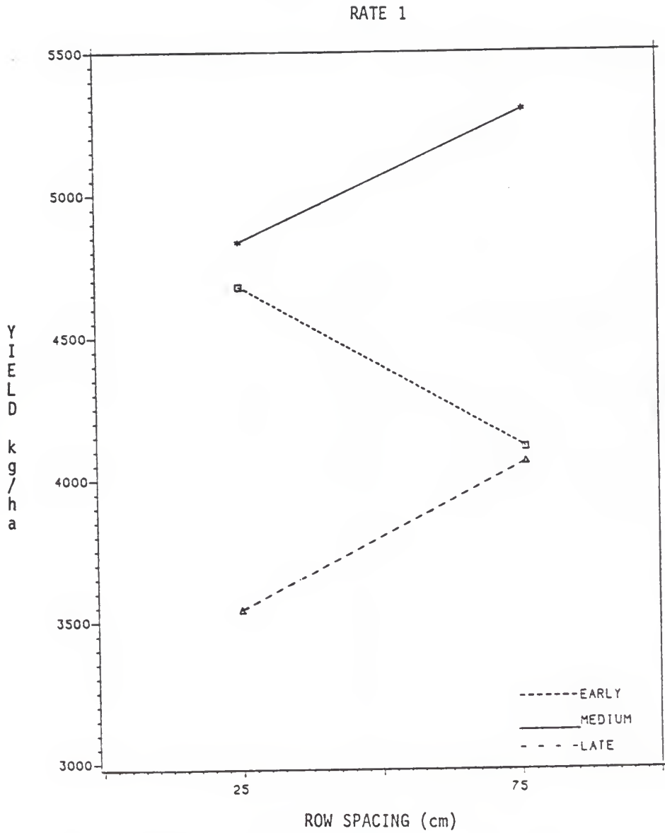
Figure 4a. Interaction of Rate X Hybrid X Spacing on Yield, Manhattan 1983. Rate 1 = 123,500 seeds/hectare
