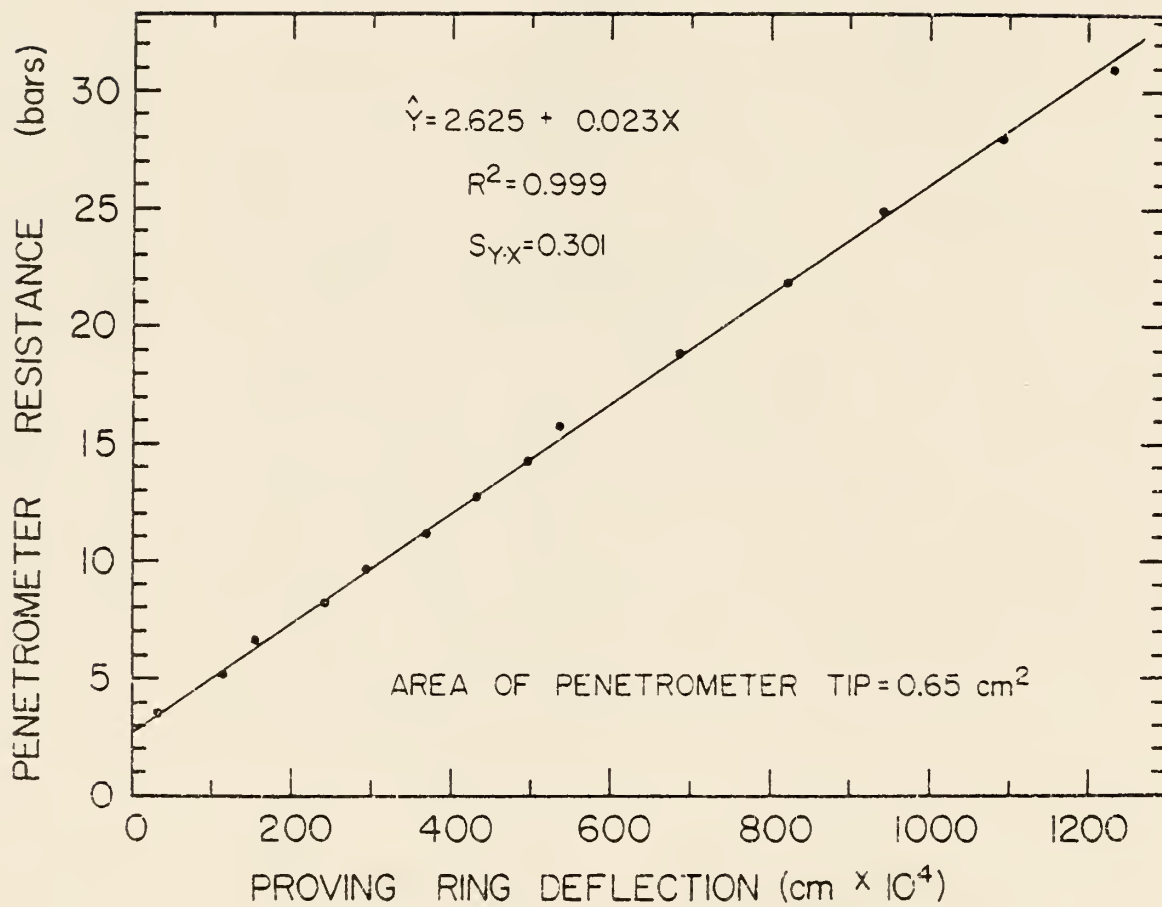
Fig. 1A: Penetrometer resistance (bars) versus proving ring deflection (cm × 10 4 ).
