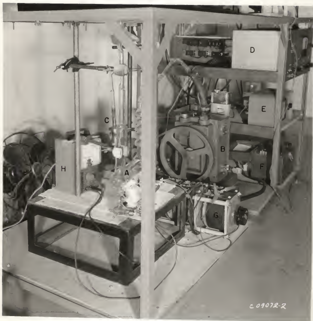
Fig. 1. Photograph of vacuum pumps and associated control panels for the ionization and Pirani gauges. A, diffusion pump; B, mechanical pump; C, Pirani gauge; D, control panel RG-21; E, control panel for GP-110 (Pirani gauge); F, potentiometer; G, variac; H, VTVM Heathkit; I, exhaust vent.
