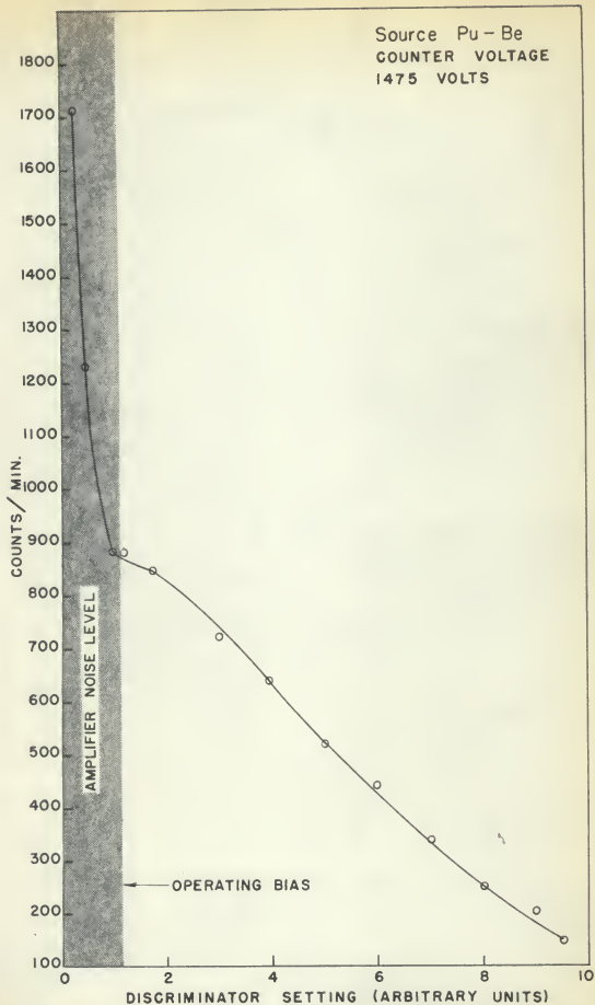
Fig. 21. Integral bias curve for \text{BF}_3 counter.
