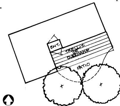
An airlock entry is protected from the wind and summer sun.
