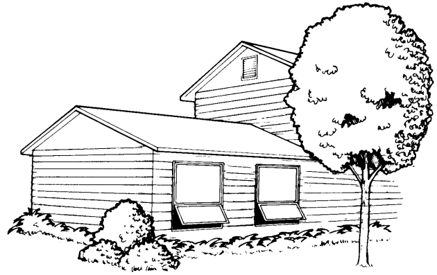
Low-placed louvered windows allow air flow at floor level.
