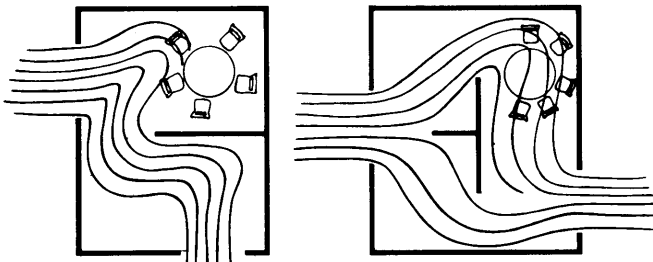
A plan view: Interior walls should be designed so air moves through the house easily.
