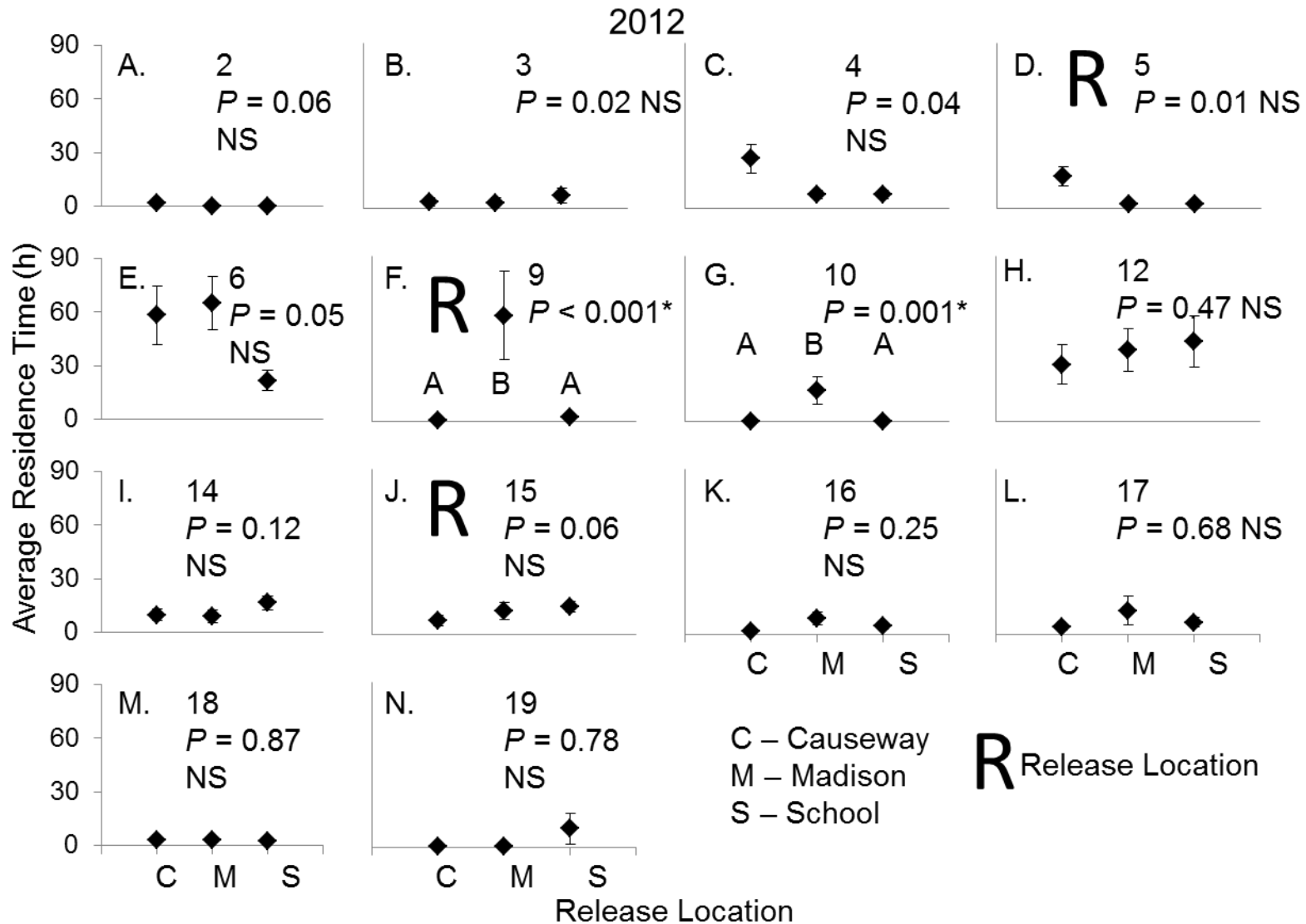
Figure D.2. Average and SE plots depicting release location differences using average residence time (h) in Milford Reservoir, KS in 2012. The X-axis is the release locations Causeway (C), Madison (M), and School (S). The Y-axis is the average residence time (h). Y-axes are standardized to compare across months. Capital R's indicate receivers closest to release location. Also shown are the results of a Kruskal-Wallis nonparametric ANOVA and post-hoc Mann Whitney U multiple comparisons with Bonferroni corrections that test release locations. Bonferroni corrected critical alpha P < 0.004 was considered significant.
