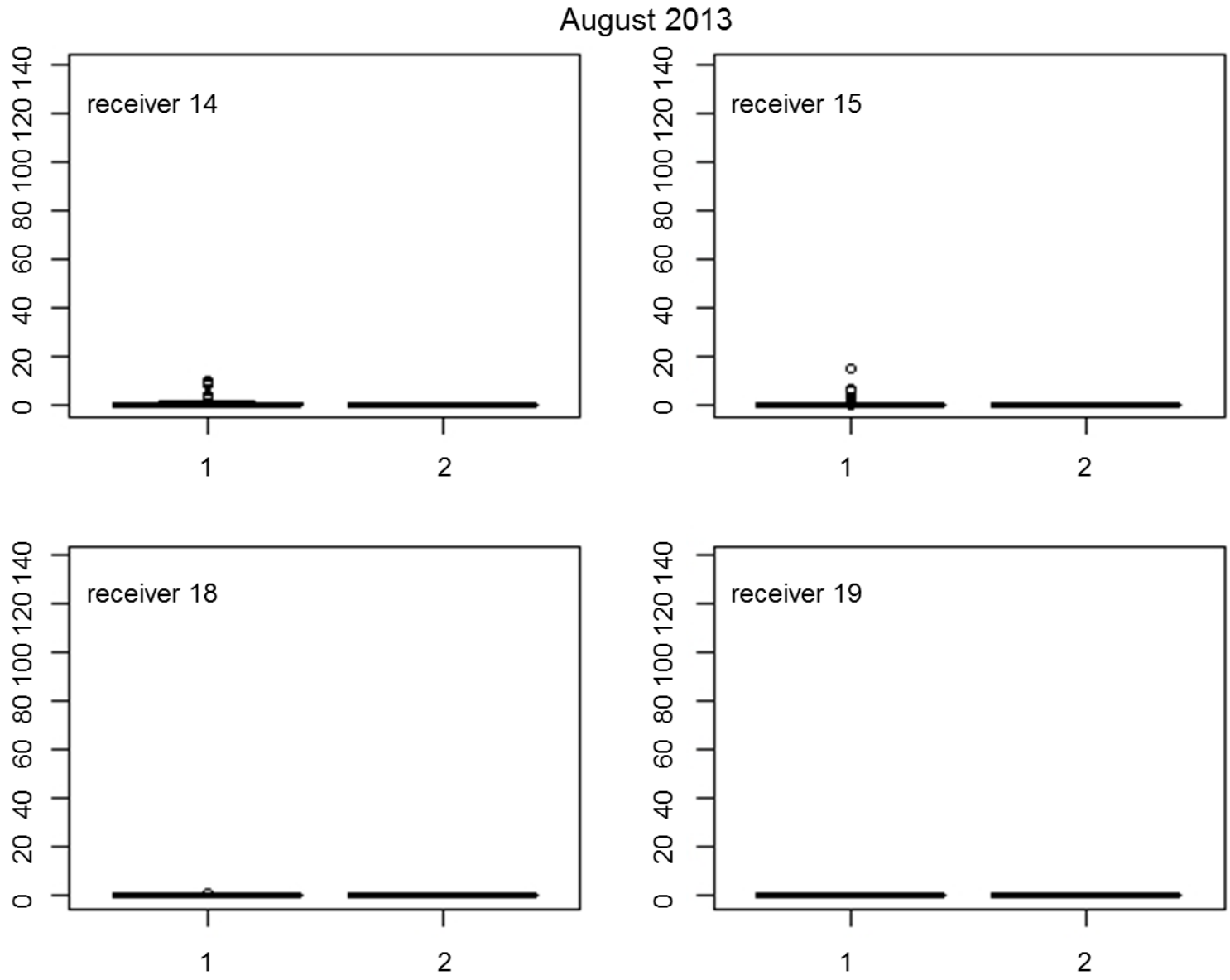
Figure K.9. Boxplots of residence times for receivers 14-19 in Milford Reservoir, KS in August, 2013. The Y axis is residence time (h); the X axis is cluster number. These data are means for individual fish in each cluster.
