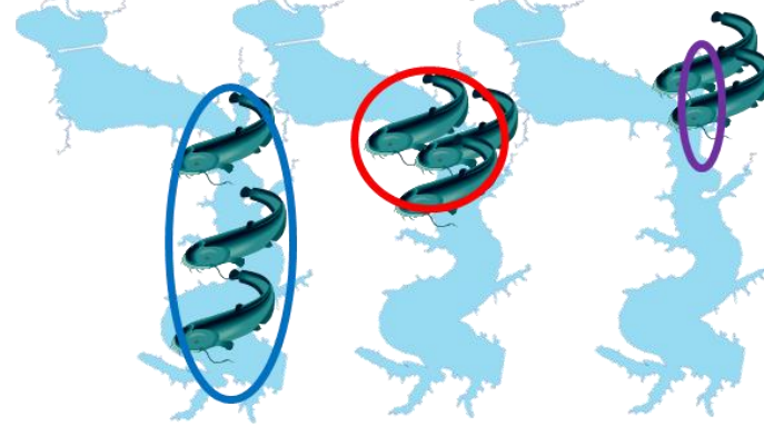
Figure 2.1. Conceptual diagram of the complexity of distribution. A total of six responses are shown three for individuals (1. presence/absence, 2. residence time, 3. number of movements) and three for populations (1. population proportion, 2. mean residence time, 3. mean movements). Also shown are my three research questions.
