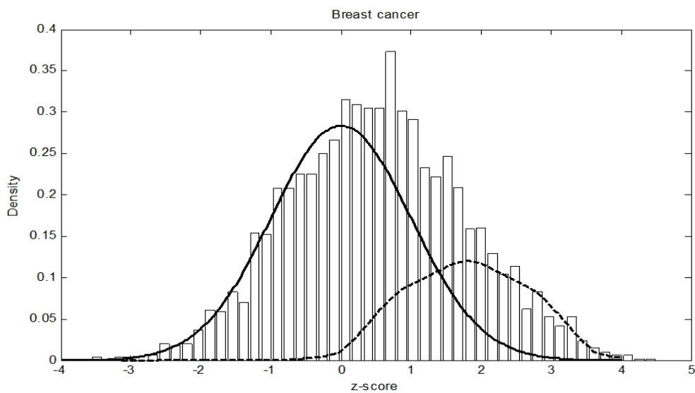
Figure 6: Breast cancer data: plot of fitted two-component mixture model with theoretical N(0, 1) null and non-null component (weighted respectively by \hat{\pi} and (1 - \hat{\pi}) ) imposed on histogram of z -score.
