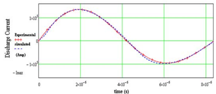
Fig. 2. The simulated current and the experimental current for deuterium at 40 mbar.
