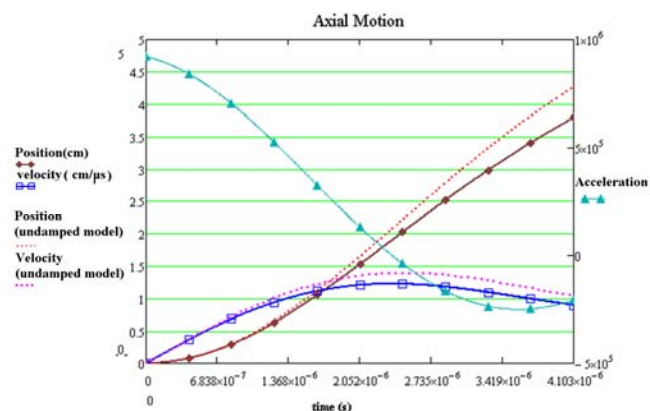
Fig. 5. Snowplow model using MathCAD dynamic sheet. Solid lines indicate the damped current model; the dotted lines indicate the sinusoidal current model. (data for neon at 40 mbar, 17 kV).
