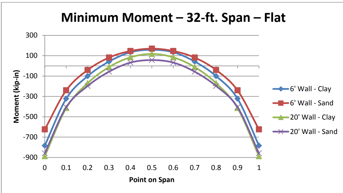
Figure 3.17: Substructural Influence on Minimum Moment for 32-ft. Flat Slab
