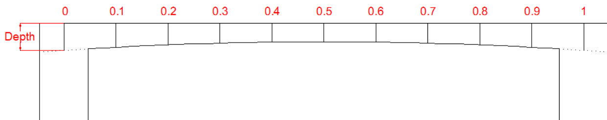
Figure 3.2: Parabolic Haunched-Slab Profile
