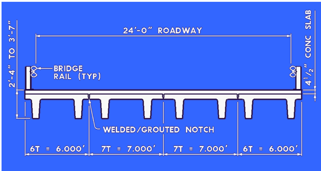
Figure 2.23: Texas Prestressed Double-Tee Beam Bridge*
