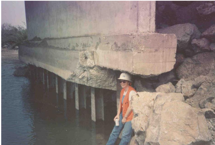
Figure 1.2: Scour Under Bridge Pile Bent
