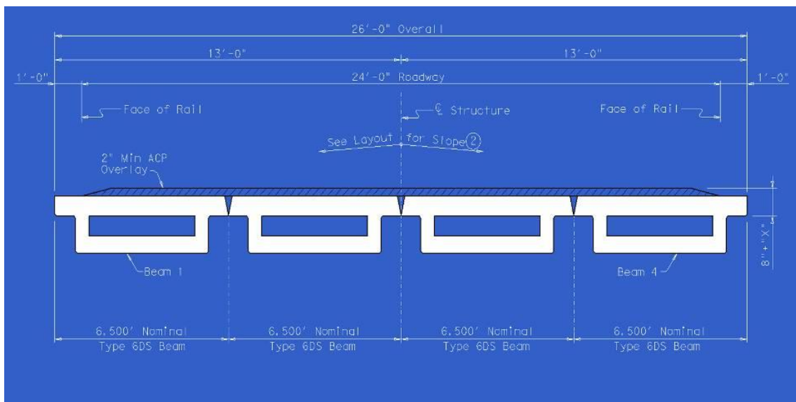
Figure 2.20: Texas Prestressed Decked-Slab Beam Bridge*
