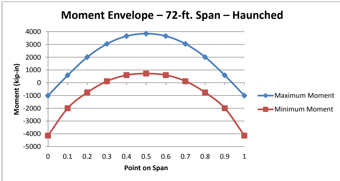
Figure 3.30: Moment Envelope for 72-ft. Span with Haunched Profile
