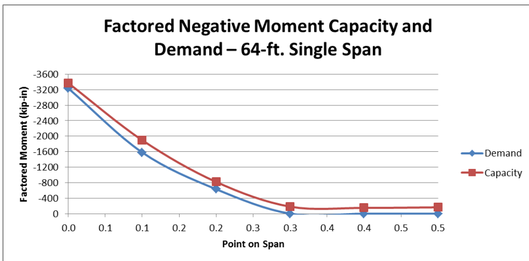
Figure 3.49: Factored Negative Moment Design of 64-ft. Section
