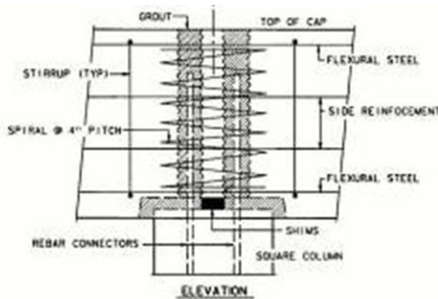
Figure 2.27: Grouted Duct Substructural Connection*
