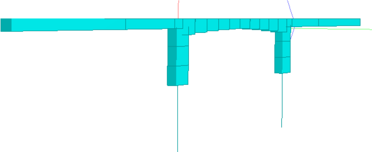
Figure 3.6: Modeled View of Strip with 6-ft. Abutment and Clay Soil
