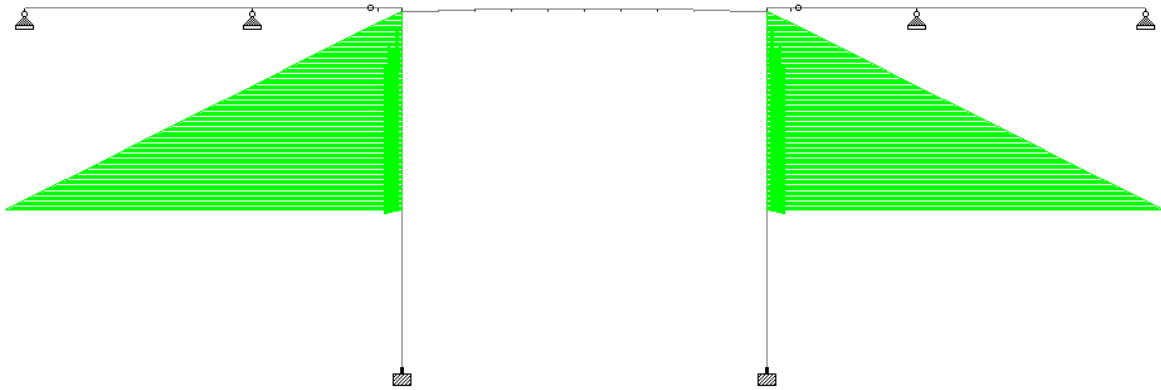
Figure 3.13: Lateral Earth Load on 20-ft. Abutment Wall
