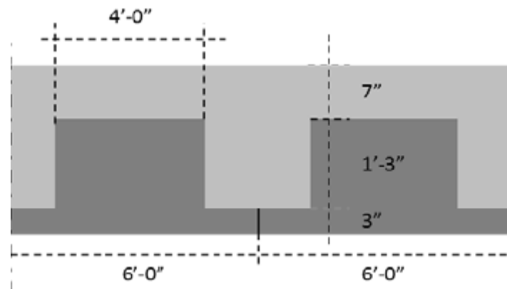
Figure 2.6: Dimensions of Minnesota Inverted-Tee System
