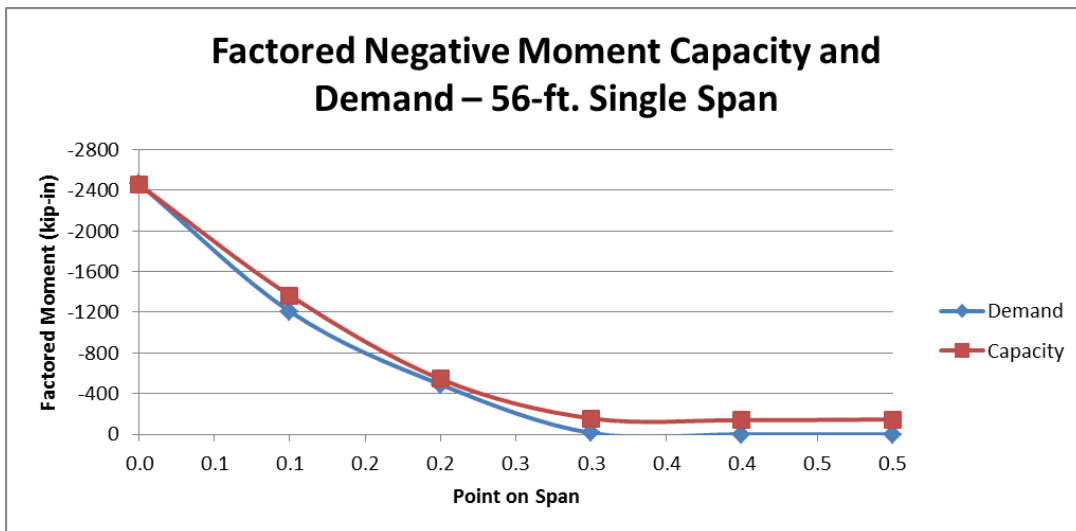
Figure 3.47: Factored Negative Moment Design of 56-ft. Section
