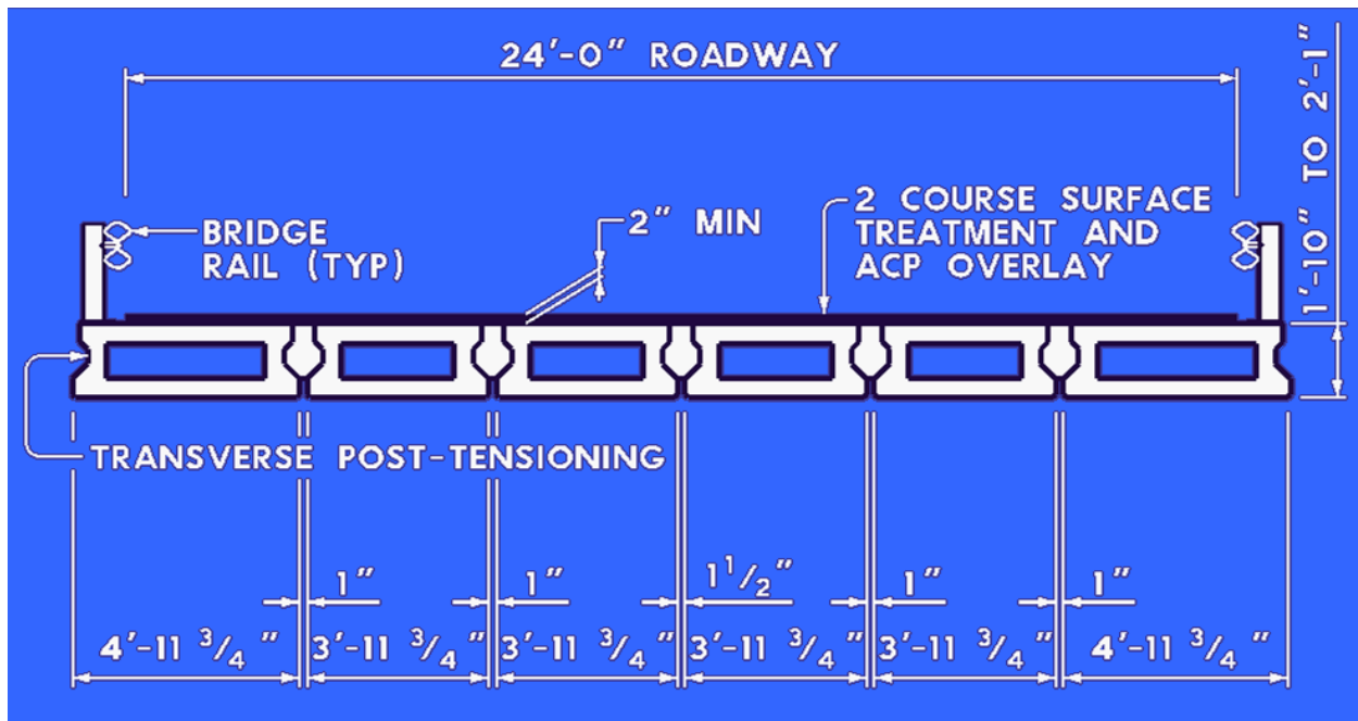
Figure 2.22: Texas Prestressed Box-Beam Bridge*
