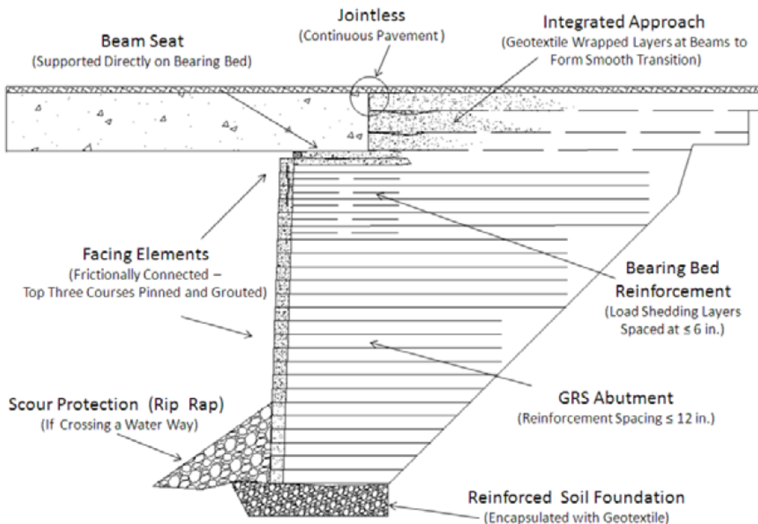
Figure 2.30: Profile of a GRS-IBS System
