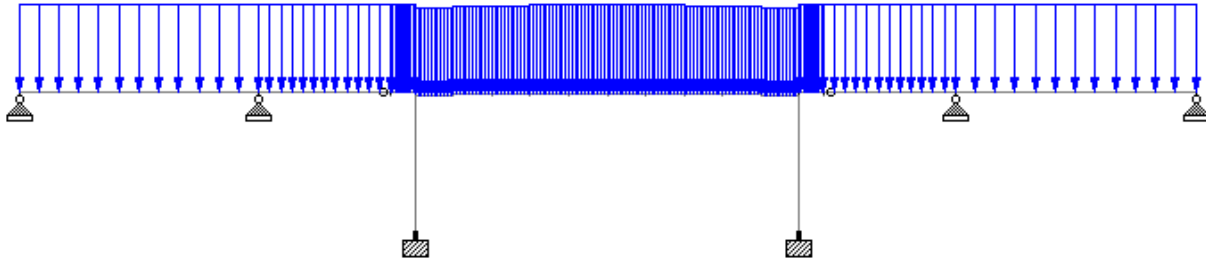
Figure 3.11: AASHTO HL-93 Lane Load on Structure
