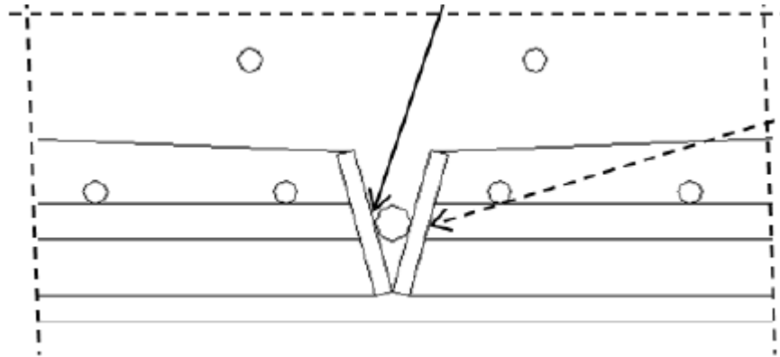
Figure 2.10: Minnesota Inverted-Tee Embedded-Plate Connection
