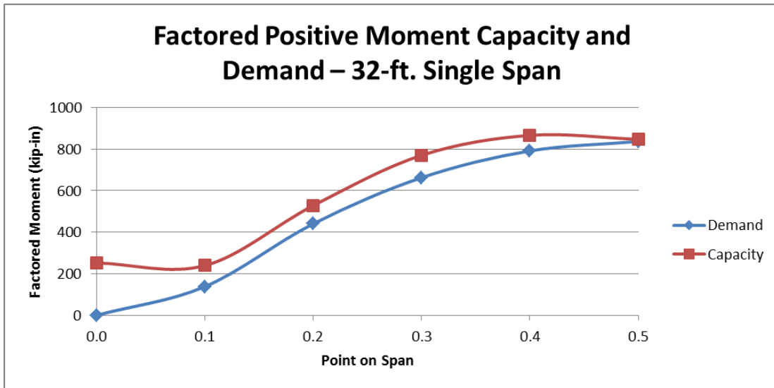
Figure 3.40: Factored Positive Moment Design of 32-ft. Section
