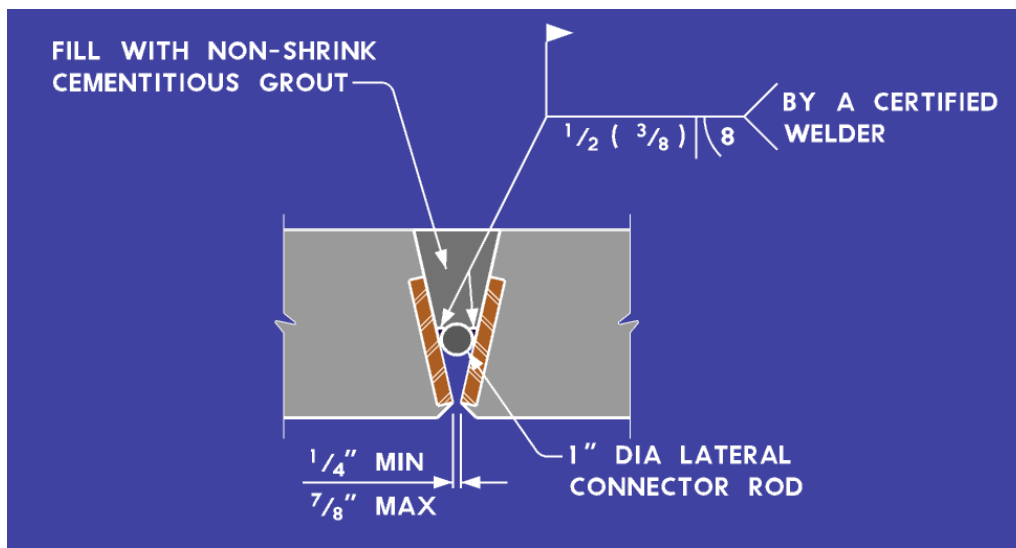
Figure 2.21: Welded Embedded-Plate Connection*
