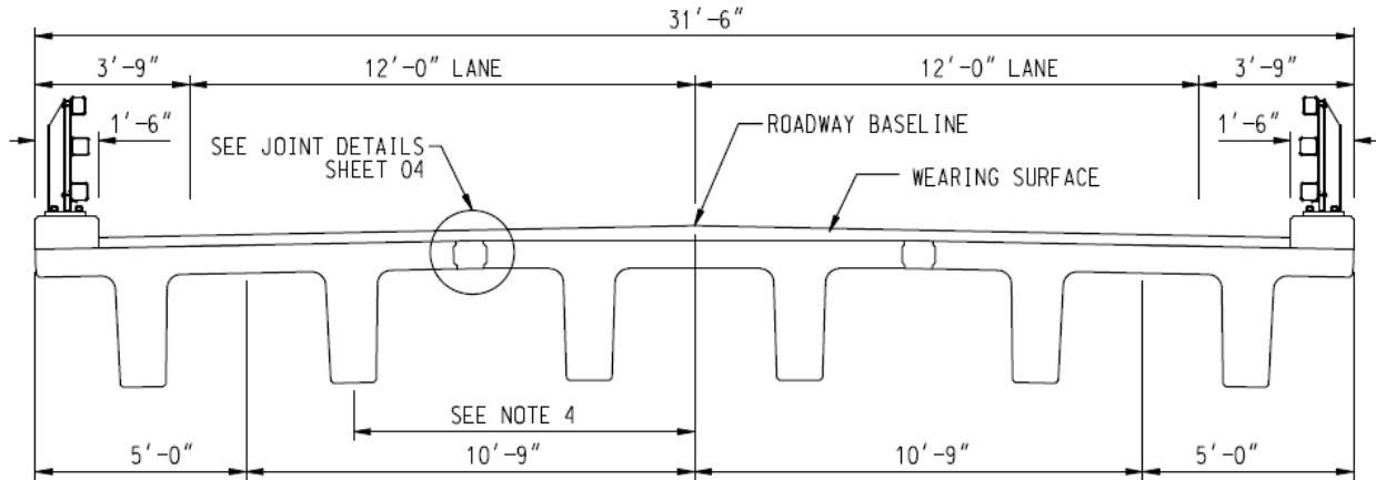
Figure 2.13: Detail of NEXT Full-Depth Section
