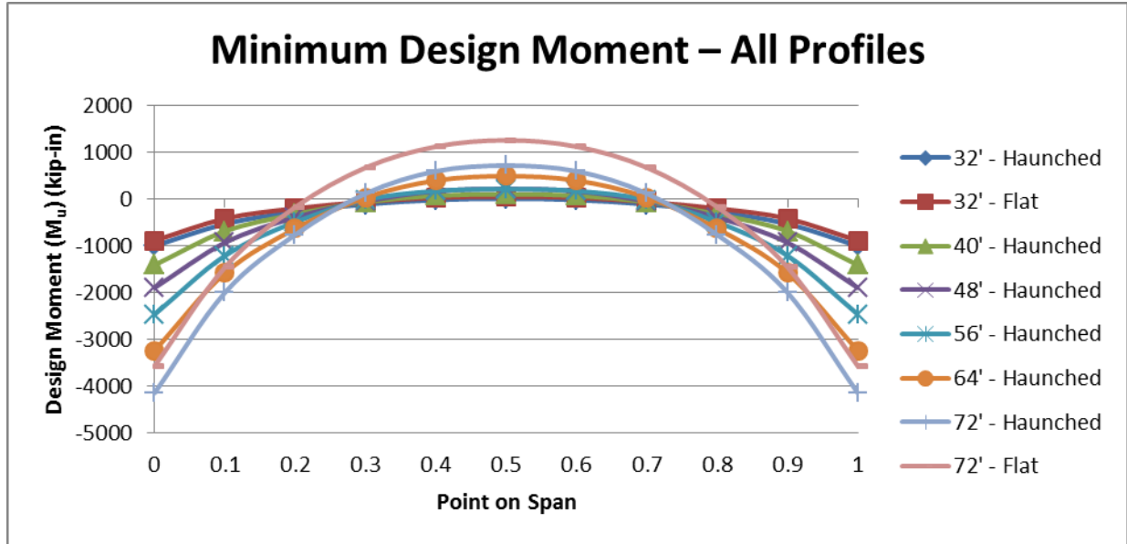
Figure 3.33: Minimum Design Moment for All Spans and Profiles
