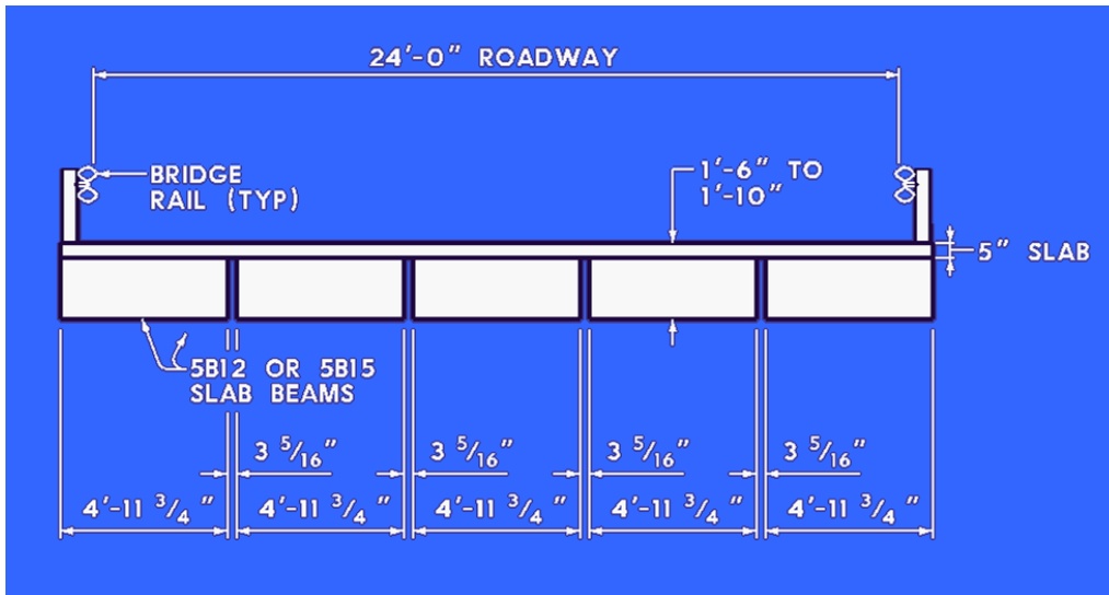
Figure 2.19: Texas Prestressed Slab-Beam Bridge*
