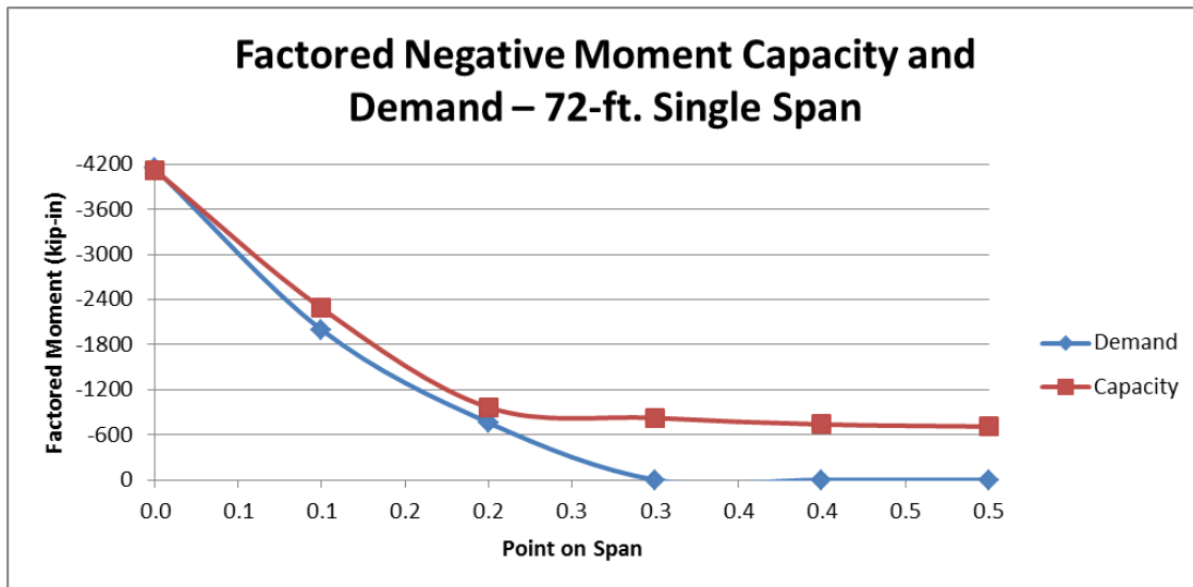
Figure 3.51: Factored Negative Moment Design of 72-ft. Section
