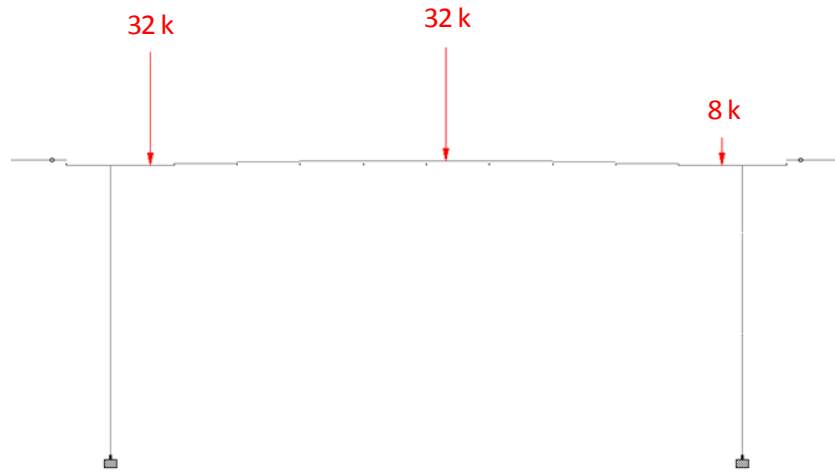
Figure 3.9: AASHTO HL-93 Truck Load on Structure
