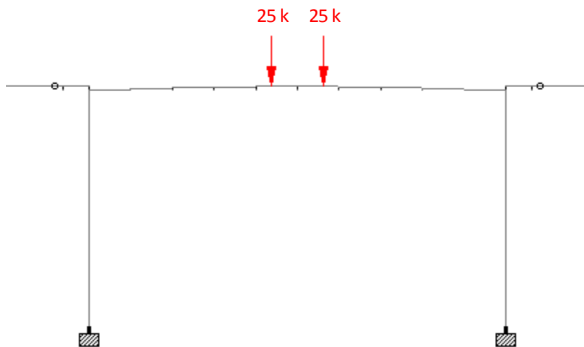
Figure 3.10: AASHTO HL-93 Tandem Load on Structure
