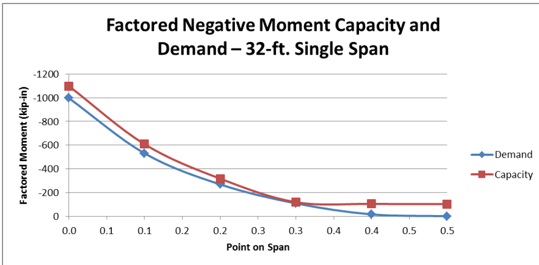
Figure 3.41: Factored Negative Moment Design of 32-ft. Section
