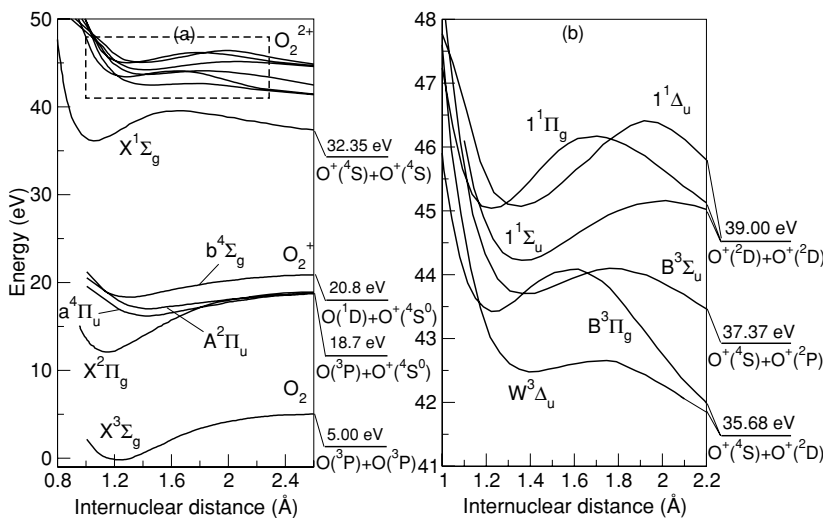
FIG. 2. (a) Potential energy curves for O_2 and O_2^+ [11] and O_2^{2+} [9]. (b) Expanded view of the region denoted in (a) by the dashed box.
