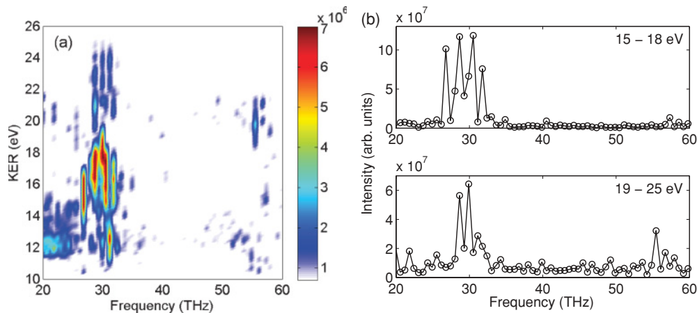
FIG. 4. (Color online) (a) The Fourier transform of the spectrum of Fig. 3(a): KER vs quantum-beat frequency. (b) Slices through energy bands in (a).
