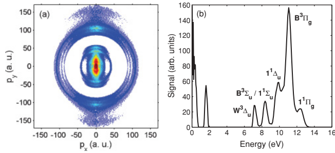
FIG. 1. (Color online) (a) Two-dimensional cut (along p_z = 0 ) through the 3D momentum distribution in Cartesian coordinates p_x , p_y , and p_z of O^+ ions from O_2 at a delay of 500 fs. The polarization is parallel to the p_y direction. (b) KER spectrum obtained from (a) via angular integration within a 30^\circ range in the direction perpendicular to the laser polarization.
