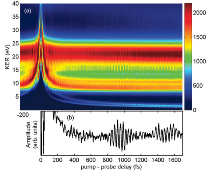
FIG. 3. (Color online) (a) KER (eV) vs pump-probe delay (fs) for O^{2+} ions. (b) Oscillations in the yield of O^{2+} for KERs between 15 and 17 eV showing vibrational revival times near 955 and 1490 fs.
