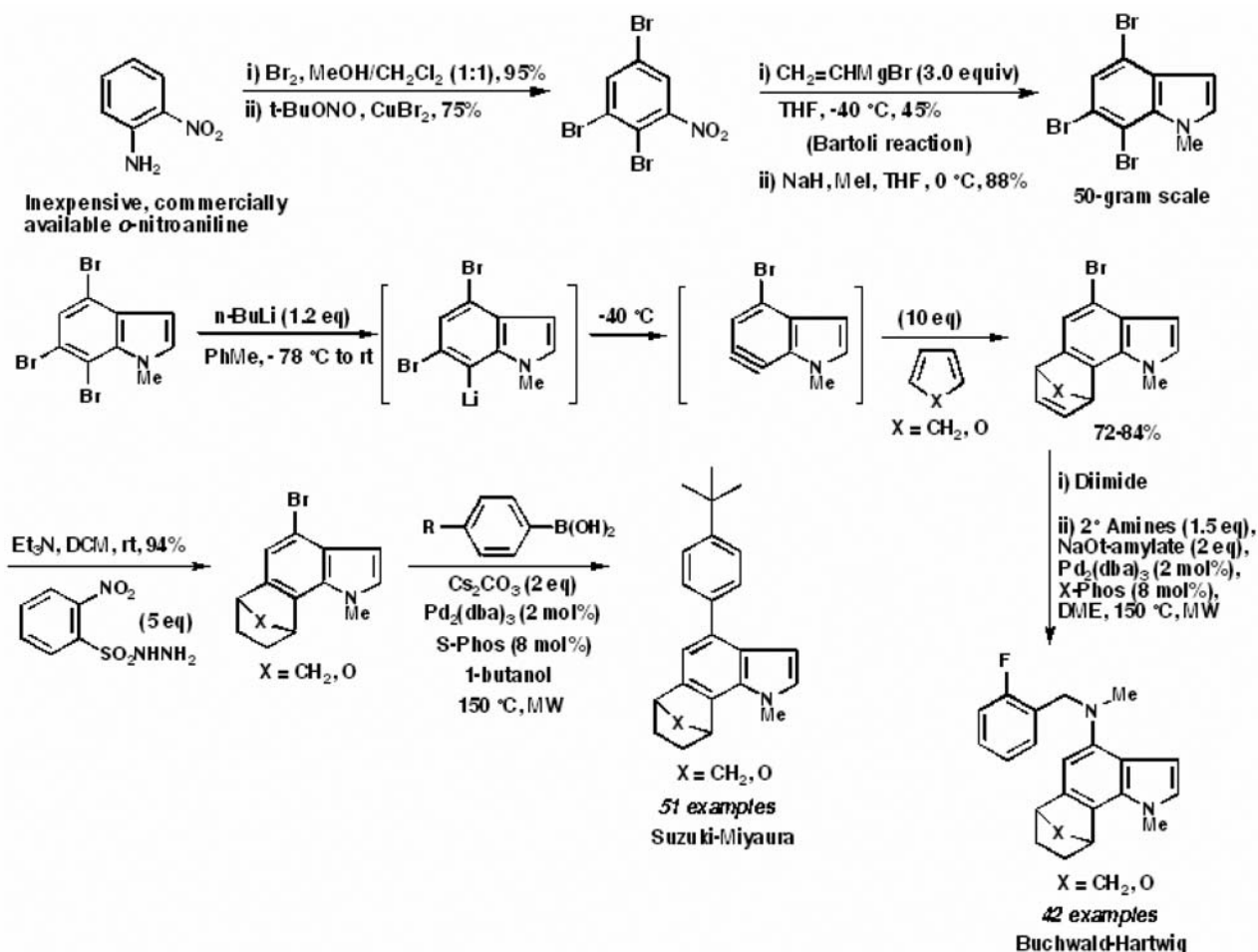
Figure 1. First example of library development that employs the indole aryne methodology to construct 6,7-annulated-4-substituted indole compounds. Top: Bartoli route to prepare the N-methyl-4,6,7-tribromoindole scaffold. Bottom: Selective generation of 4-bromo-6,7-indole aryne, and strategic combination of 6,7-indolyne cycloaddition and cross-coupling reactions under both Suzuki-Miyaura and Buchwald-Hartwig conditions to construct polycyclic indole libraries.
