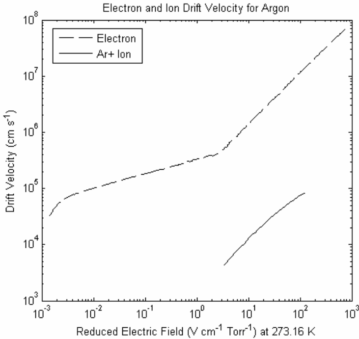
Figure 3.7: Drift velocity of electrons and Ar + ions in argon at 273.16 K [23,24].
