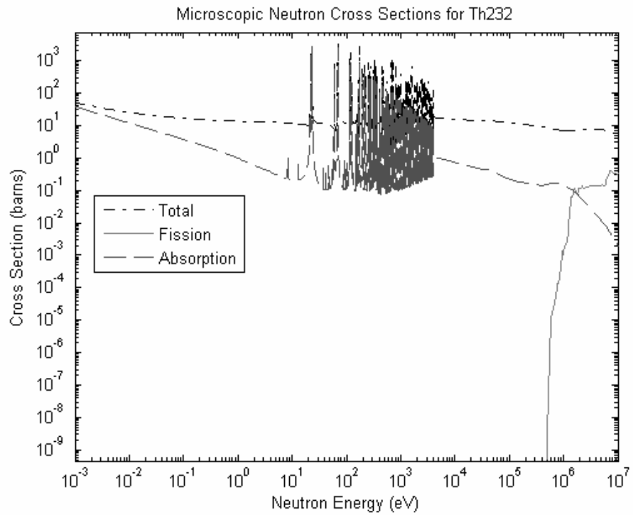
Figure B.9: Microscopic neutron cross sections for Th-232 [17].
