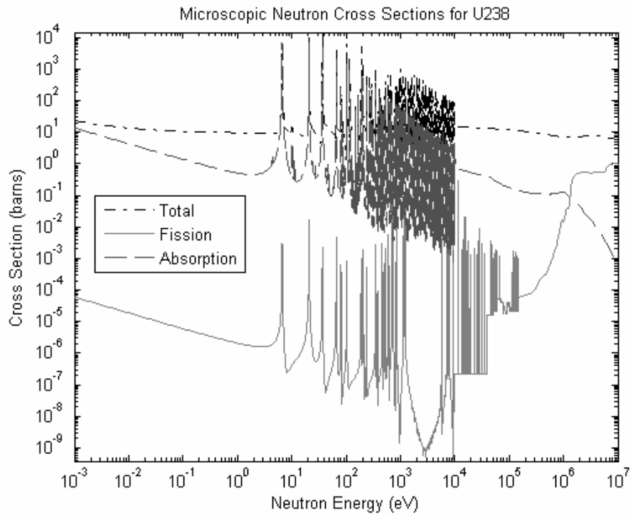
Figure B.17: Microscopic neutron cross sections for U-238 [17].
