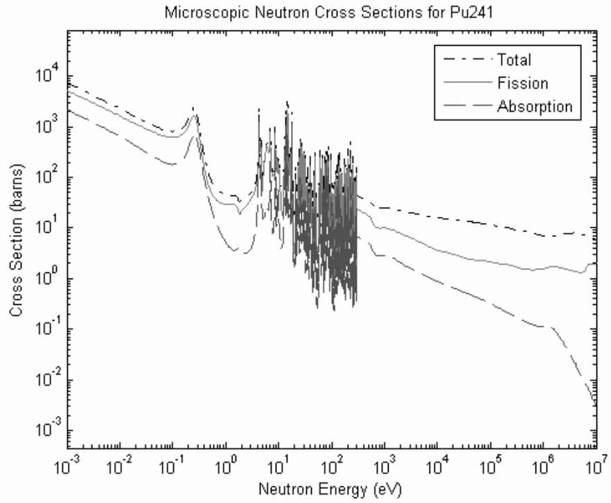
Figure B.8: Microscopic neutron cross sections for Pu-241 [17].
