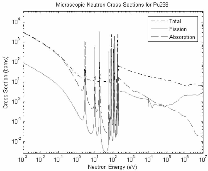
Figure B.5: Microscopic neutron cross sections for Pu-238 [17].
