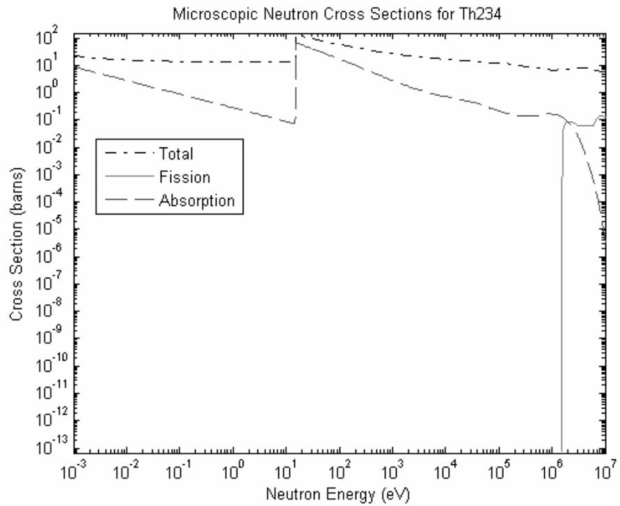
Figure B.11: Microscopic neutron cross sections for Th-234 (from JENDL-3.3 300 K) [17].
