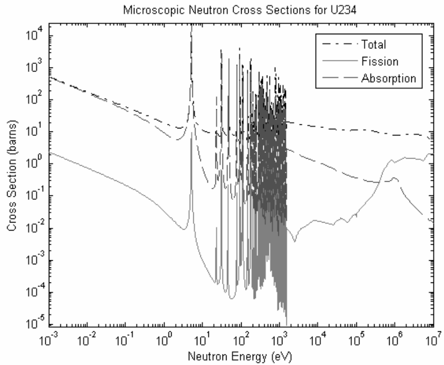
Figure B.13: Microscopic neutron cross sections for U-234 [17].
