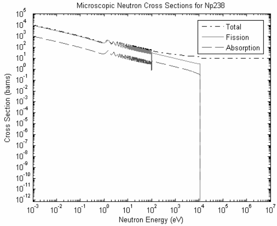
Figure B.2: Microscopic neutron cross sections for Np-238 [17].
