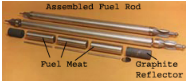
Figure 5.3: Parts of a fuel rod used in the Kansas State University TRIGA Mark-II Nuclear Reactor [37].
