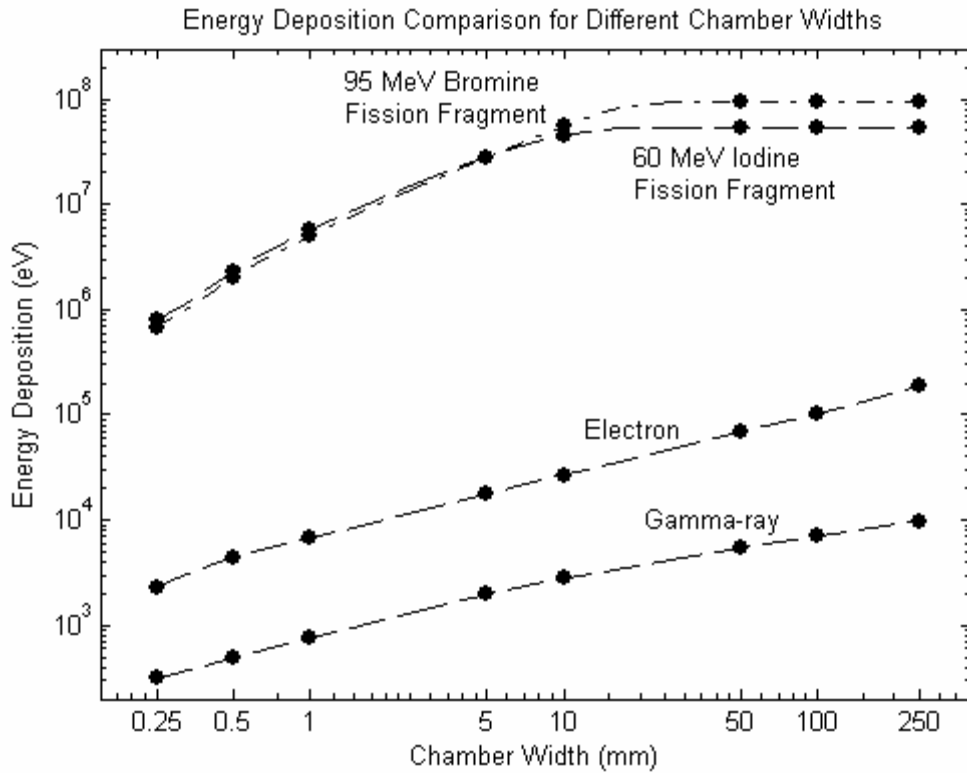
Figure 3.6: Energy deposition comparison for different chamber widths.
