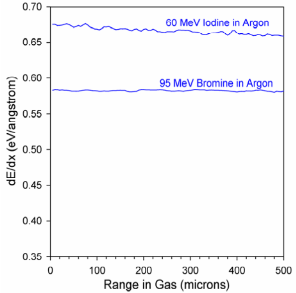
Figure 3.2: Expanded view of Figure 3.1 showing that nearly 3 MeV is deposited by fission products in only half a millimeter of argon fill gas at 1 atm.
