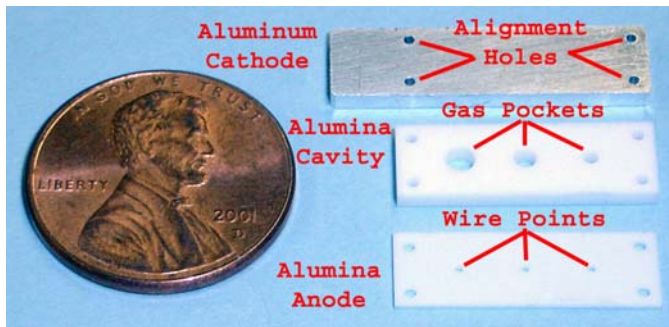
Figure 4.2: Manufactured 3-chamber alumina substrates and aluminum backing plate.
