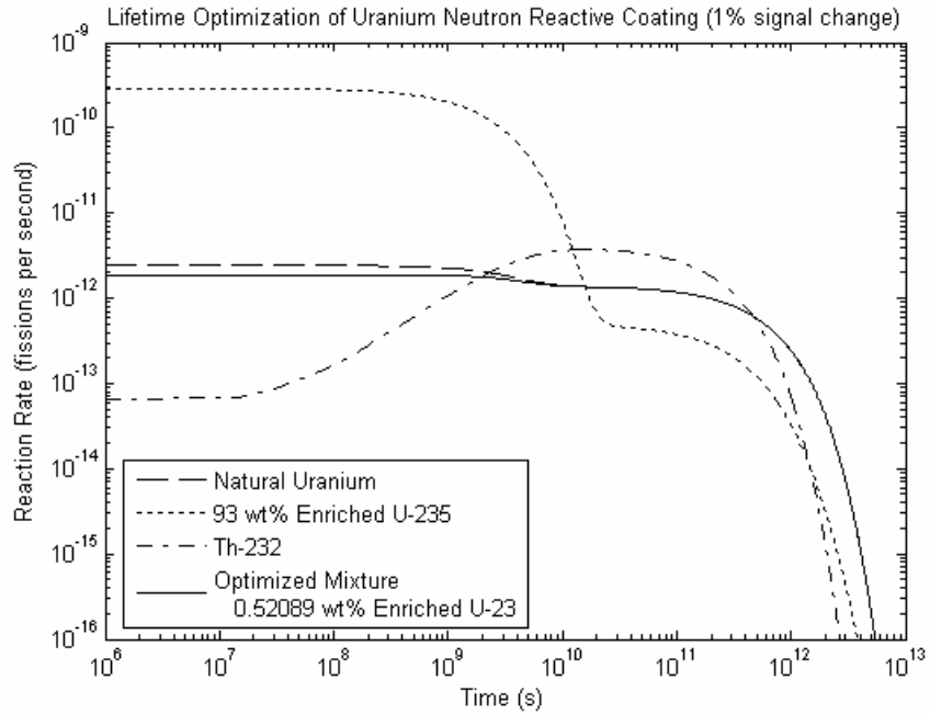
Figure 3.20: Lifetime optimization using enriched uranium for 15.273 kW continuous operations.
