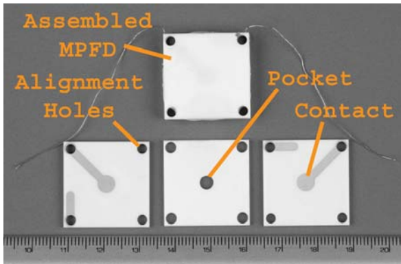
Figure 4.3: Using spare alumina substrates to form an MPFD. Shown is actually the very first prototype MPFD ever built.
