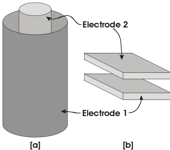
Figure 2.1: Basic design of [a] cylindrical and [b] parallel plate fission chambers.
