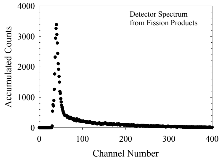
Figure 8.2: Beamport differential pulse height spectrum for a natural uranium coated MPFD with 3 mm diameter by 1 mm wide chamber [1,14].
