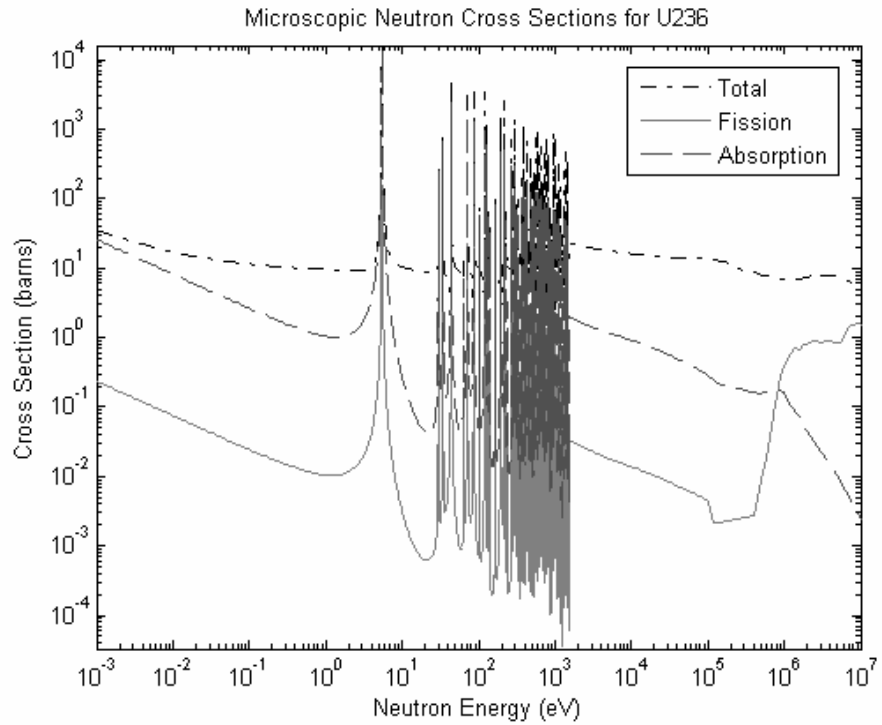
Figure B.15: Microscopic neutron cross sections for U-236 [17].
