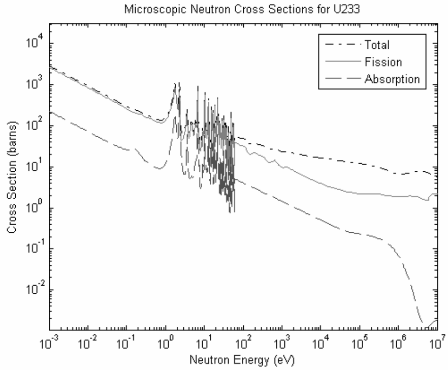
Figure B.12: Microscopic neutron cross sections for U-233 [17].
