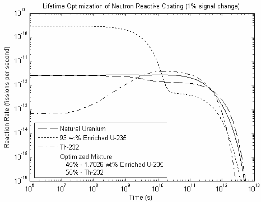
Figure 3.21: Lifetime optimization using a mixture of enriched uranium and thorium for 15.273 kW continuous operations.
