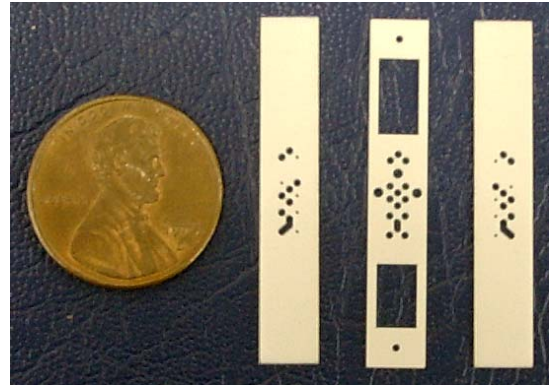
Figure 6.1: MPFD 3 -T alumina substrates.
