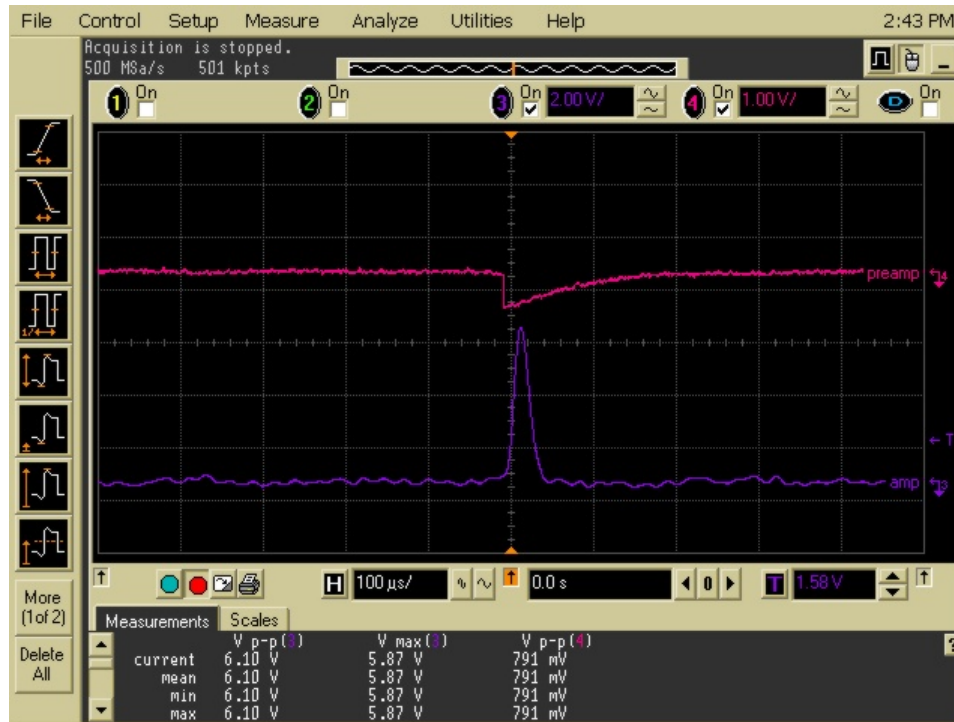
Figure 8.5: Oscilloscope screen capture showing preamplifier (top) and amplifier (bottom) outputs during in-core tests.
