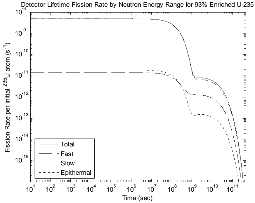
Figure 3.15: Detector lifetime fission rate by neutron energy range for 93% enriched ^{235}\text{U} .
