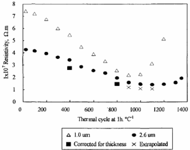
Figure 7.2: Resistivity variation of two evaporated platinum strips after heat treatments. Extrapolated and corrected for thickness data takes into account the decrease in thickness after heat treatments [40].
