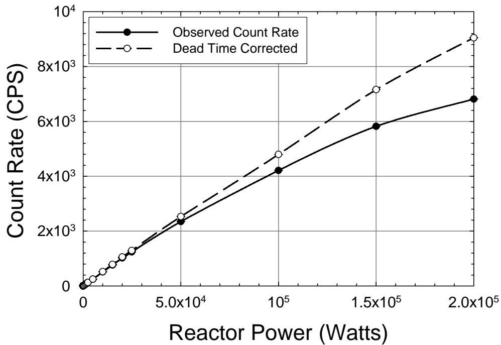
Figure 8.4: Linear plot of Figure 8.3 showing a deadtime of only 24% at 200 kW or 9.6 \times 10^{12} slow n \text{cm}^{-2} \text{s}^{-1} flux [15].
