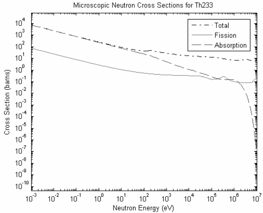
Figure B.10: Microscopic neutron cross sections for Th-233 (from JENDL-3.3 300 K) [17].
