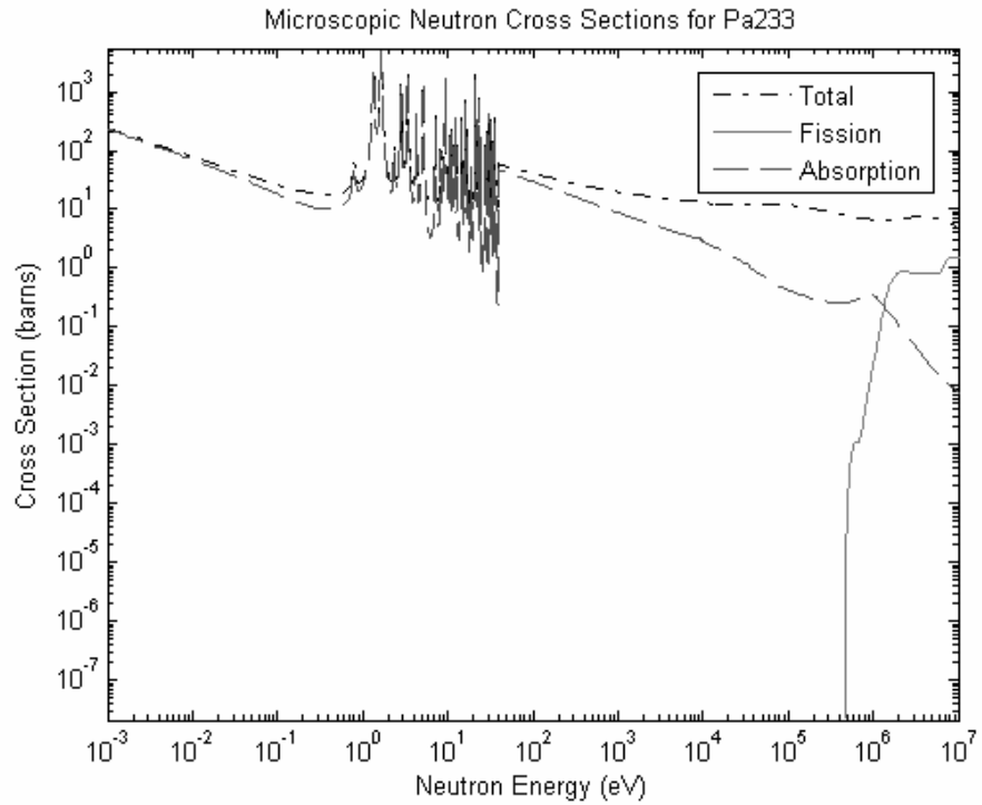
Figure B.4: Microscopic neutron cross sections for Pa-233 [17].
