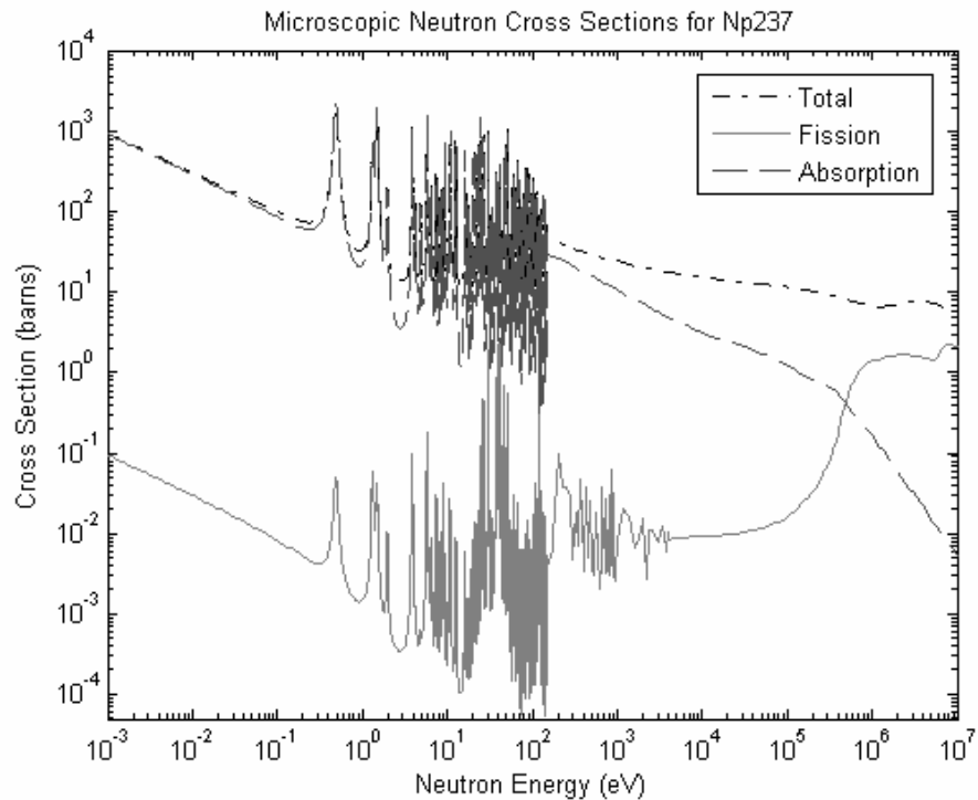
Figure B.1: Microscopic neutron cross sections for Np-237 [17].
