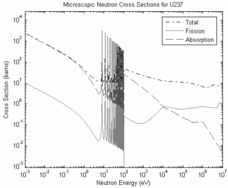
Figure B.16: Microscopic neutron cross sections for U-237 [17].
