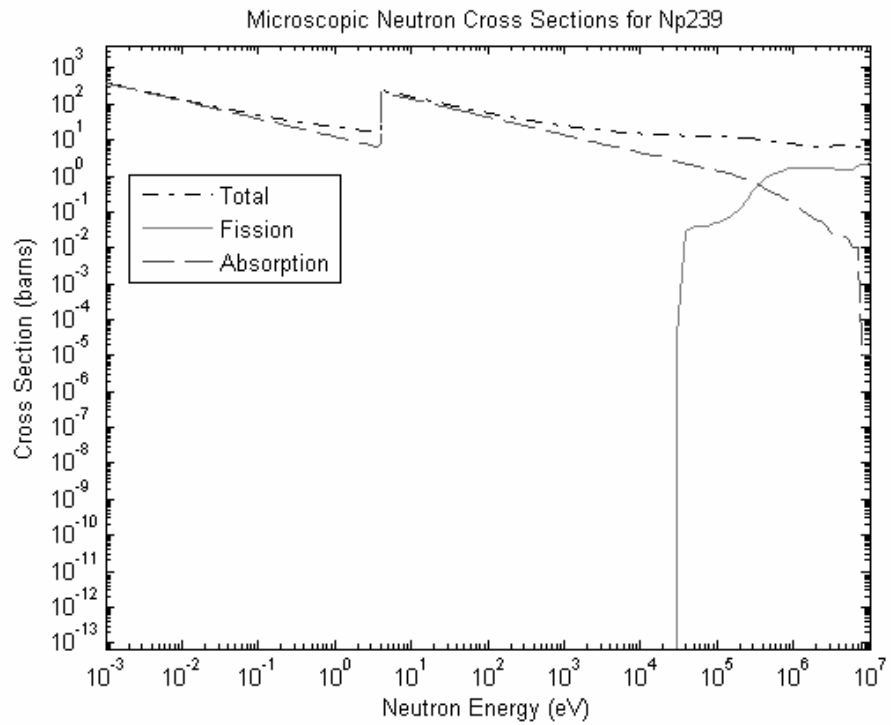
Figure B.3: Microscopic neutron cross sections for Np-239 [17].
