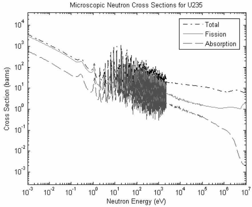
Figure B.14: Microscopic neutron cross sections for U-235 [17].
