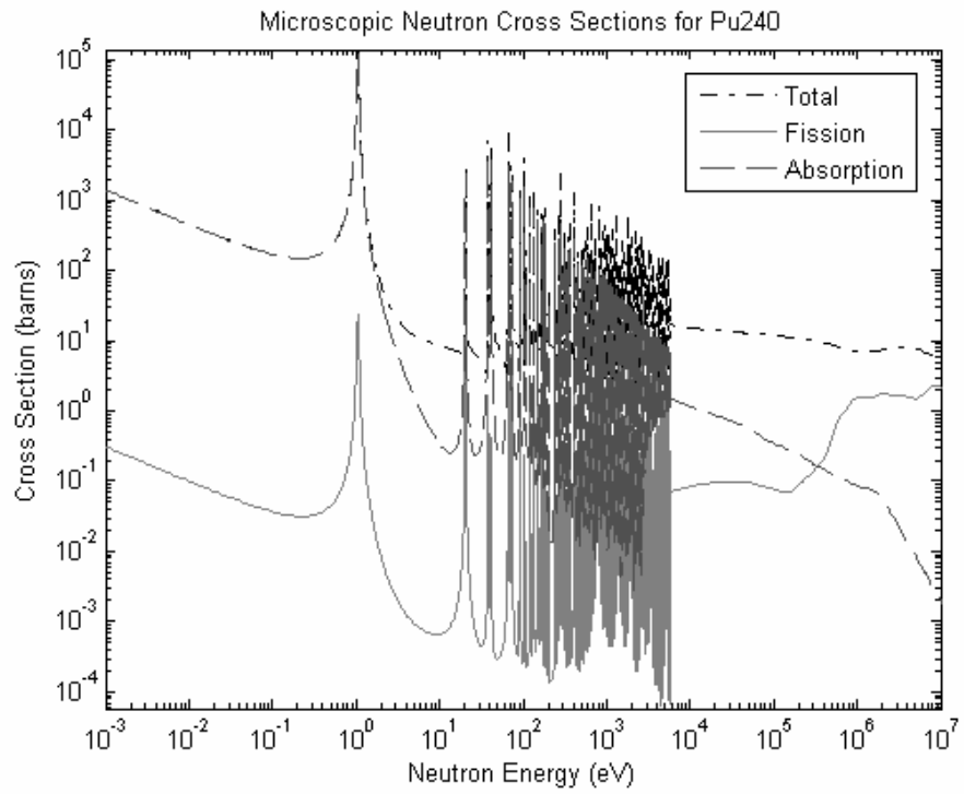
Figure B.7: Microscopic neutron cross sections for Pu-240 [17].
