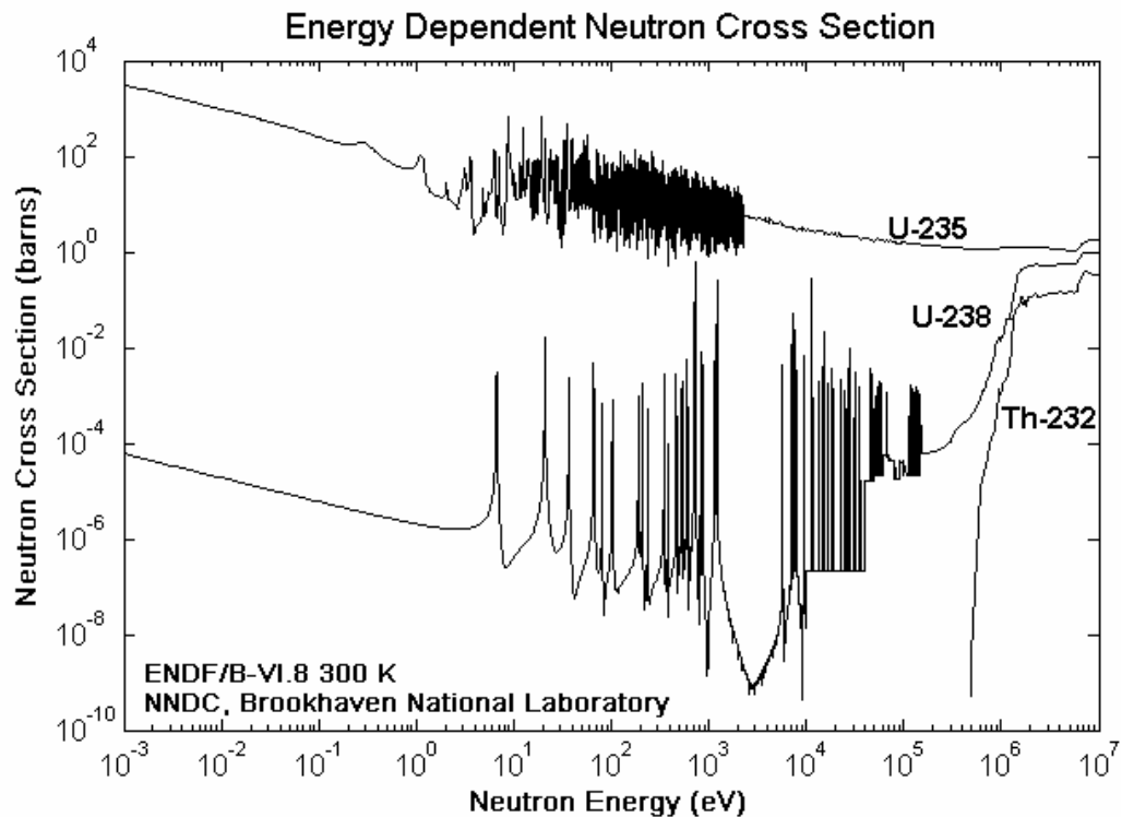
Figure 2.2: Energy dependent neutron cross sections for ^{235}\text{U} , ^{238}\text{U} , and ^{232}\text{Th} from the ENDF/B-VI.8 300 K cross section library [17].
