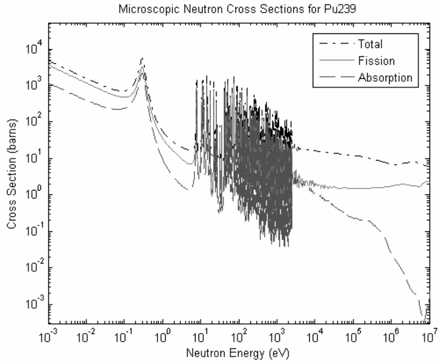
Figure B.6: Microscopic neutron cross sections for Pu-239 [17].
