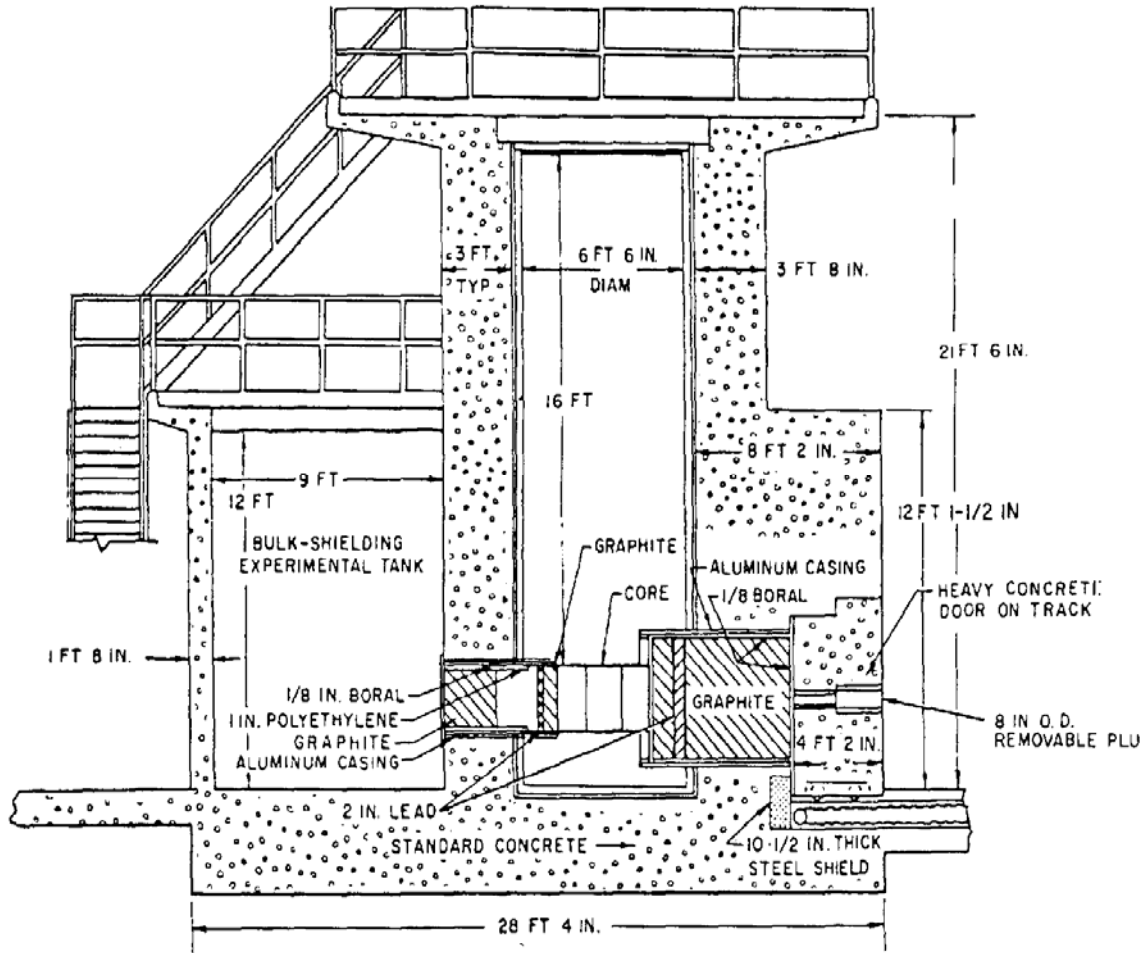
Figure 5.4: Vertical cross section of the Kansas State University TRIGA Mark-II Reactor [29].
