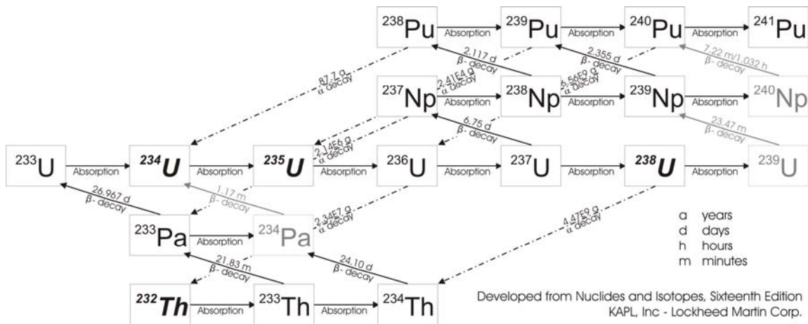
Figure 3.11: Isotope buildup and decay of fissile coatings (developed from [30]).
