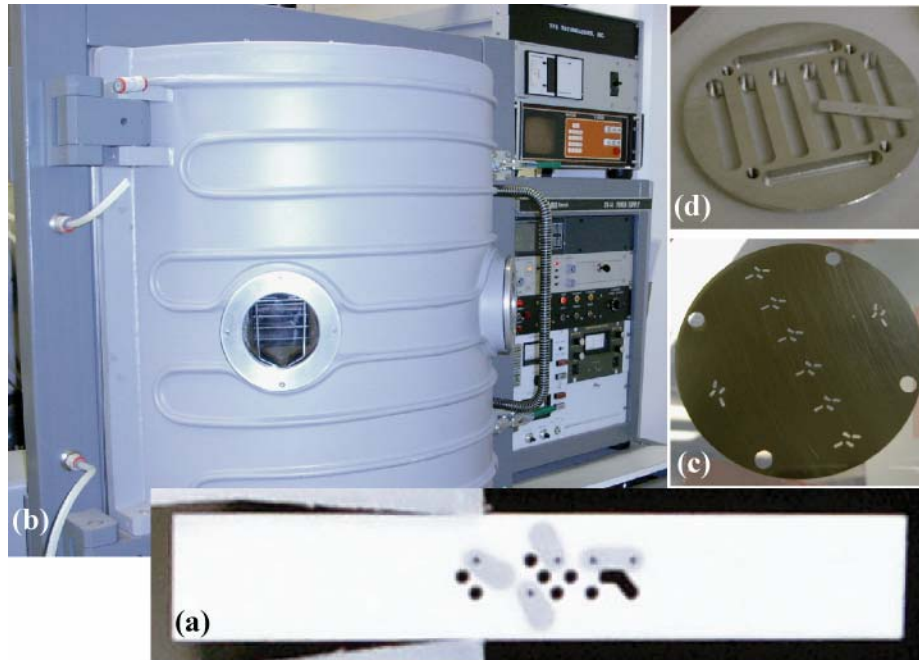
Figure 7.1: (a) Electrodes were deposited on the substrates using the (b) S.M.A.R.T. Lab's electron beam evaporator. The pattern was defined by a (c) shadow mask which was attached to the bottom of a (d) substrate holder.
