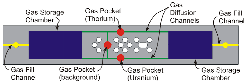
Figure 6.2: The cavity substrate of the MPFD 3 -T shown with gas fill/flow features highlighted.
