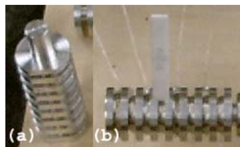
Figure 7.18: The wire winding spool contains cylindrical slots for each wire, (b) a slot for hold an assembled MPFD vertical, and (a) a bottom flat to keep the spool from rolling inside the annealing oven.
