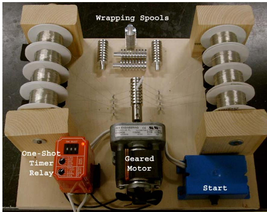
Figure 7.19: Custom built wire winding system with an MPFD loaded in the wrapping spool slot.
