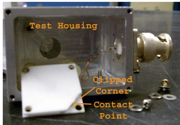
Figure 4.5: A successful and reproducible contact design ready for beam port testing.
