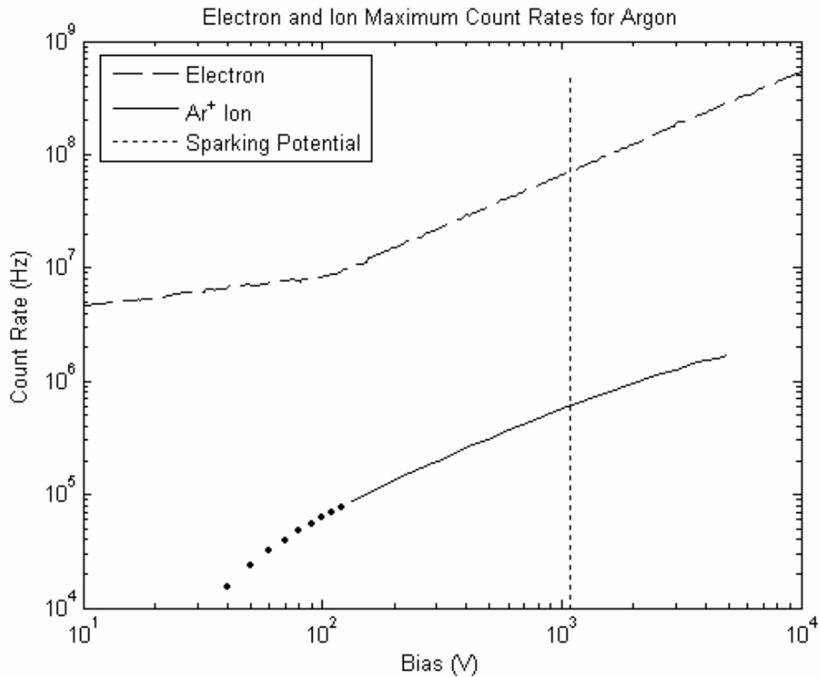
Figure 3.9: Maximum count rate achievable versus detector bias for pure argon fill gas.
