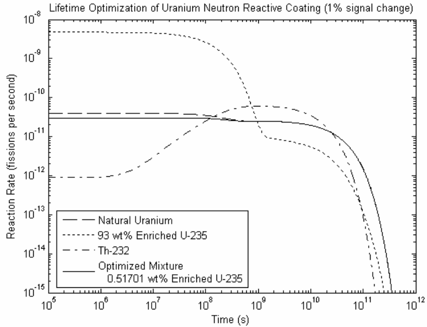
Figure 3.18: Lifetime optimization using enriched uranium for full power continuous operations.
