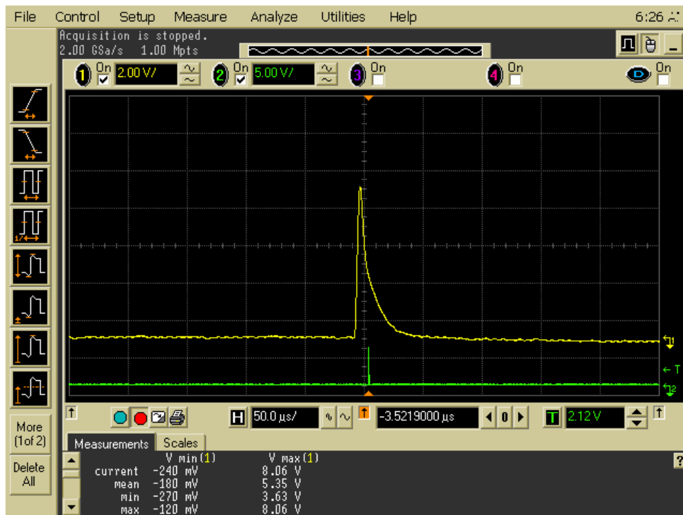
Figure 8.6: Oscilloscope screen capture showing preamplifier (top) and discriminator (bottom) outputs using an Amptek A250 preamplifier closely coupled to an MPFD tested at the southeast beamport.
