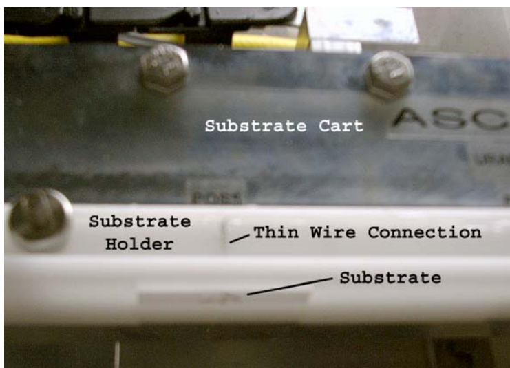
Figure 7.8: Substrate cart of ASCEFI with the attached substrate holder loaded with a substrate. The substrate is held in place and is connected to the electroplating circuit through a thin wire that goes through the base of the holder.
