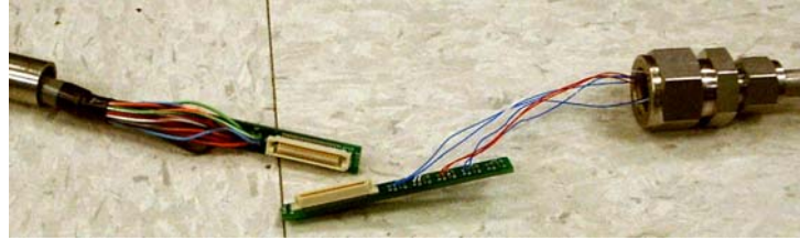
Figure 7.22: Connector circuit boards for switching wiring from the bare 30 AWG wiring (prototype insulated wiring shown) in the flux probe tube to the shielded 24 AWG wiring in the 5/8" stainless steel tubing.
