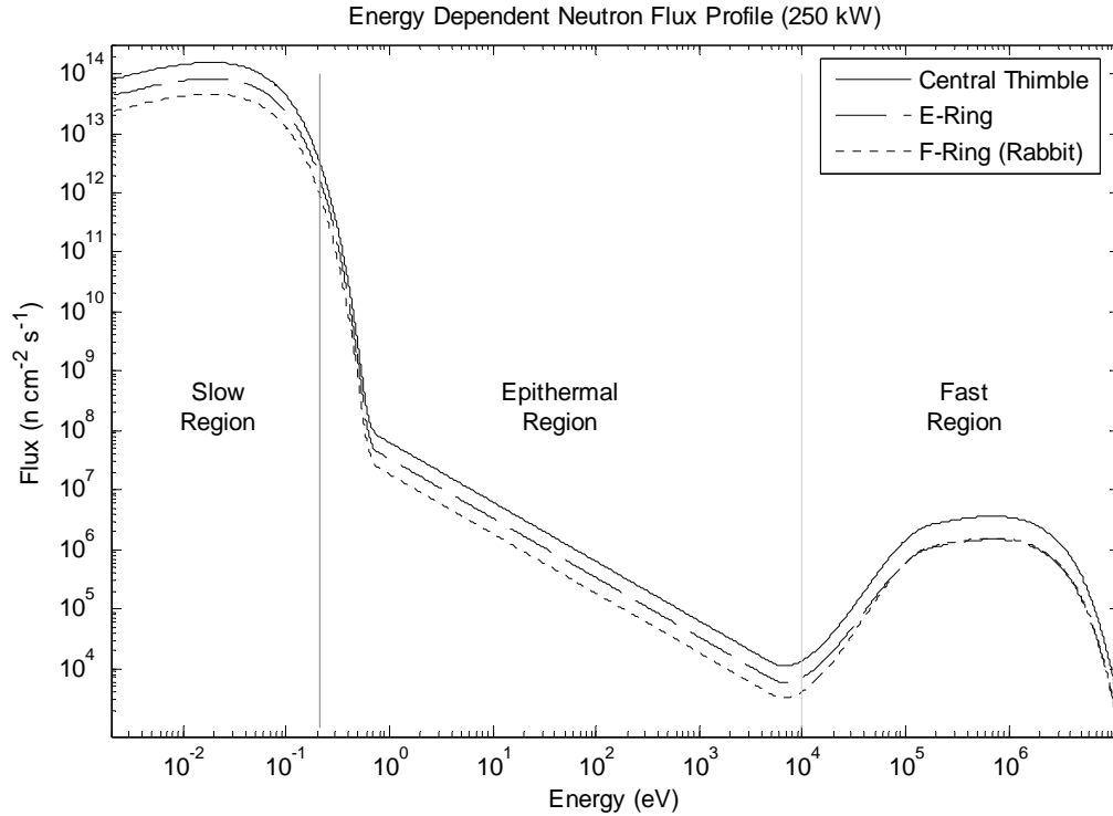
Figure 3.10: Energy dependent neutron flux profiles for the Kansas State University TRIGA Reactor in the Central Thimble, E-Ring, and F-Ring (see A.2.2 for generation program).
