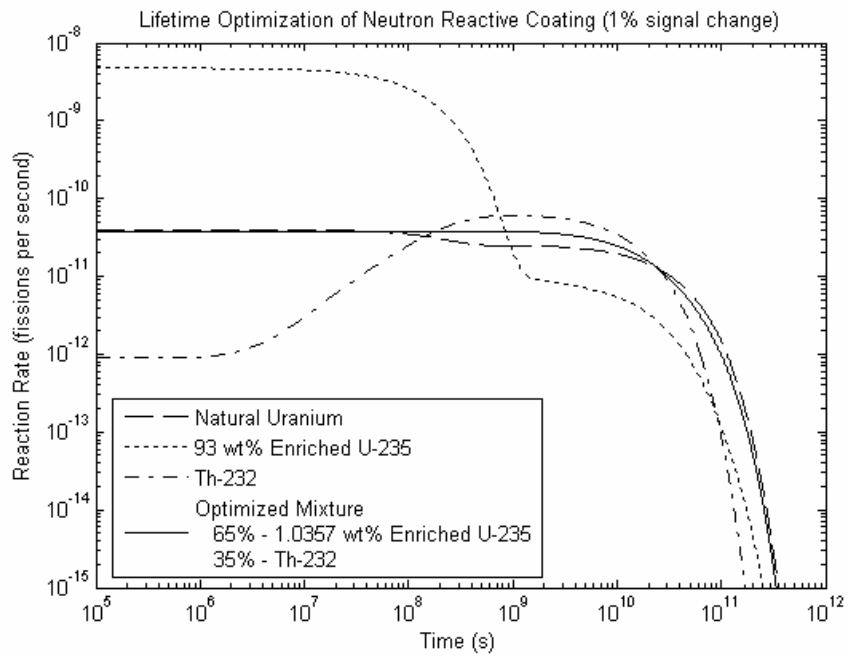
Figure 3.19: Lifetime optimization using a mixture of enriched uranium and thorium for full power continuous operations.
