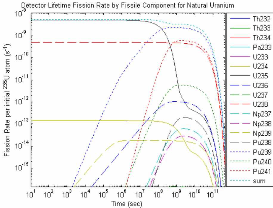
Figure 3.12: Detector lifetime fission rate by fissile component for natural uranium.
