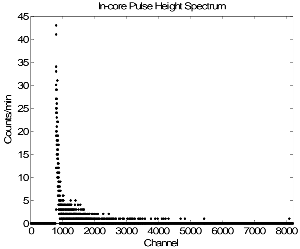
Figure 8.7: Differential pulse height spectrum of the MPFD with a bias of 1000 V.
