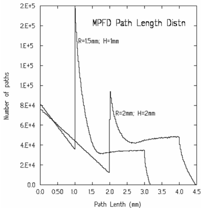
Figure 8.1: Theoretical pulse height spectrum based on fission product path length through two different detector sizes [1].
