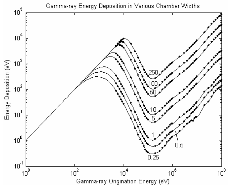
Figure 3.3: Data (dots) and spline fit (lines) of gamma-ray energy deposition in various chamber widths of argon gas.
