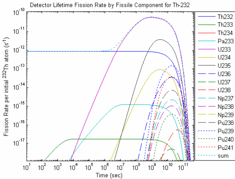
Figure 3.16: Detector lifetime fission rate by fissile component for ^{232}\text{Th} .
