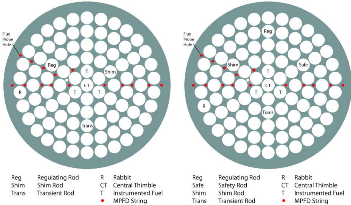
Figure 5.1: Existing Kansas State University TRIGA Reactor core configuration II-21.
