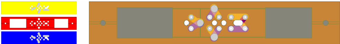
Figure 6.4: Semi-transparent overlay of the two base substrates with platinum electrodes and the cavity substrate showing how the different components work together.
