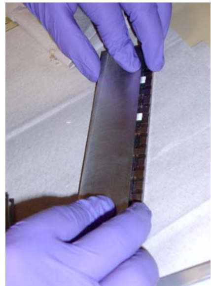
Figure 7.15: Interdigitated plates for aligning the substrate pieces and pressing them together.
