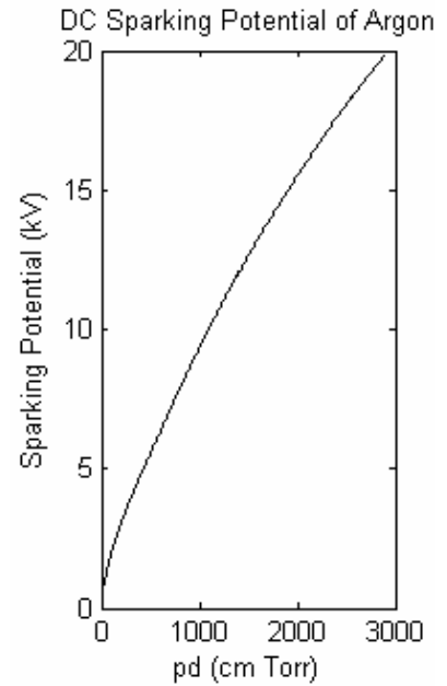
Figure 3.8: DC sparking potential of argon as a function of pressure and chamber width [25].
