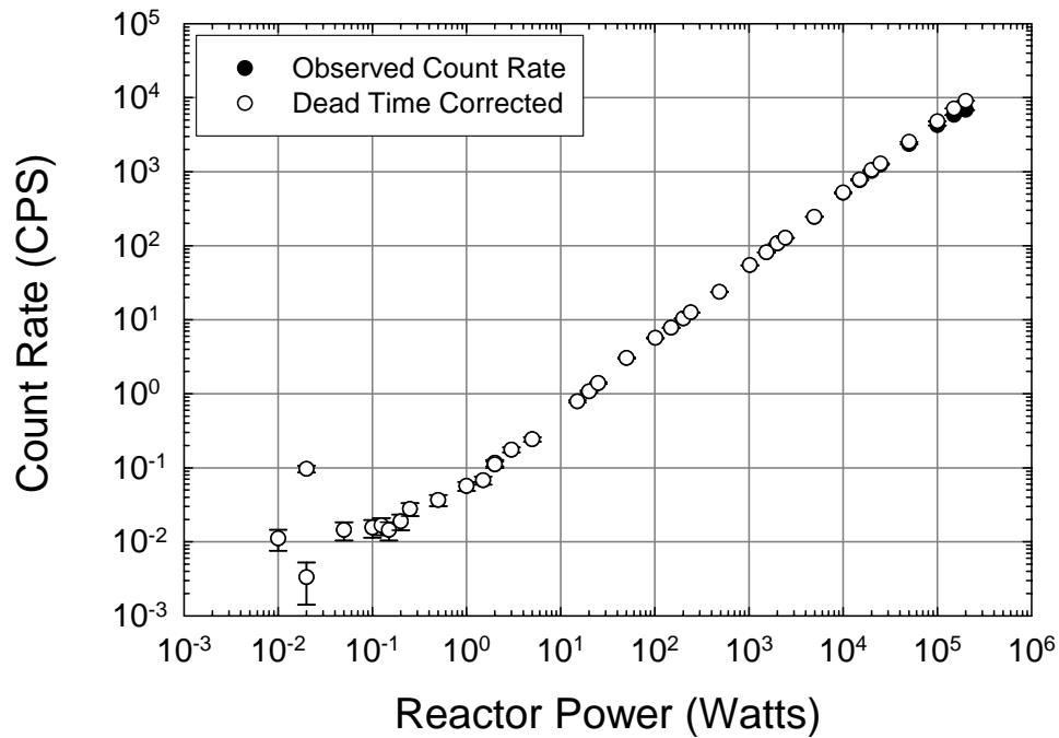
Figure 8.3: In-core central thimble test results from 10 mW to 200 kW with detector operated in pulse-mode [15].
