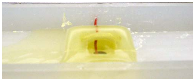
Figure 7.12: Uranium plating bath with flowing solution. The red wire connects to the platinum mesh through which the electrolytic solution flows.
