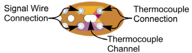
Figure 6.5: Expanded view from Figure 6.4 showing the embedded thermocouple location.
