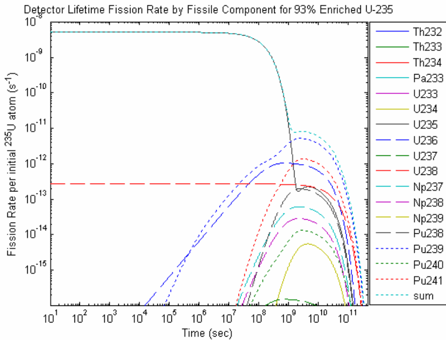
Figure 3.14: Detector lifetime fission rate by fissile component for 93% enriched ^{235}\text{U} .
