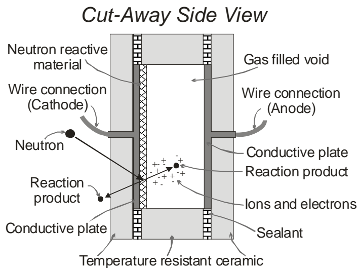
Figure 2.4: Cut-away side view of the MPFD showing fill gas ionization from a neutron induced reaction with the neutron reactive material [13].
