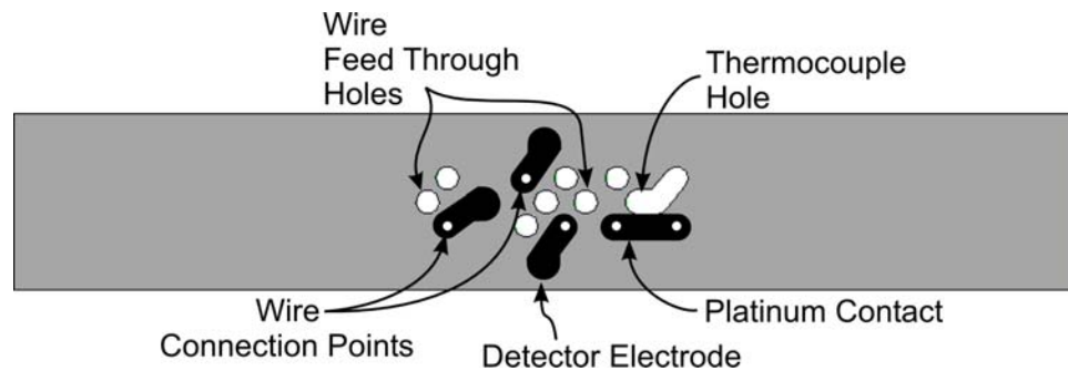
Figure 6.3: The base substrate of the MPFD 3 -T shown with electrical coatings.
