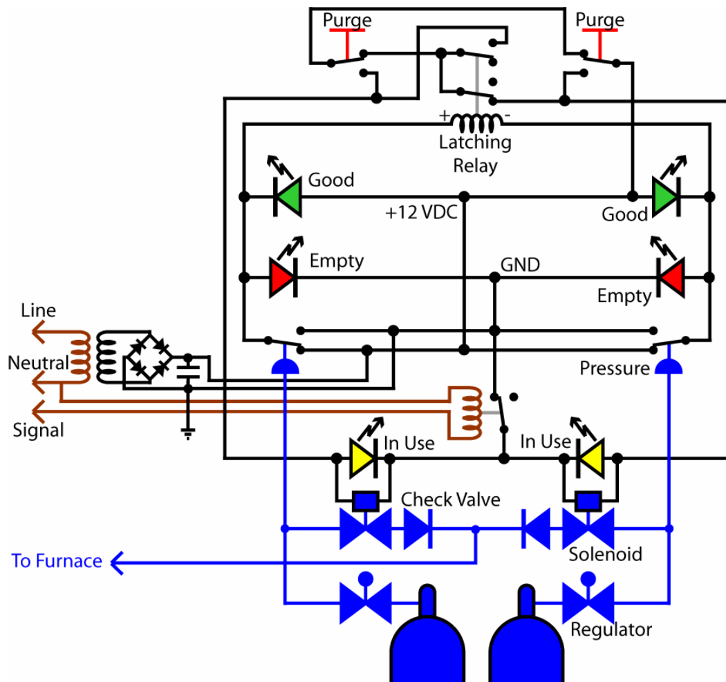
Figure 7.6: Flow schematic and circuitry diagram for Mr. Cylinder.
