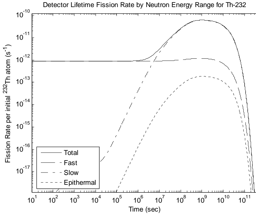
Figure 3.17: Detector lifetime fission rate by neutron energy range for ^{232}\text{Th} .
