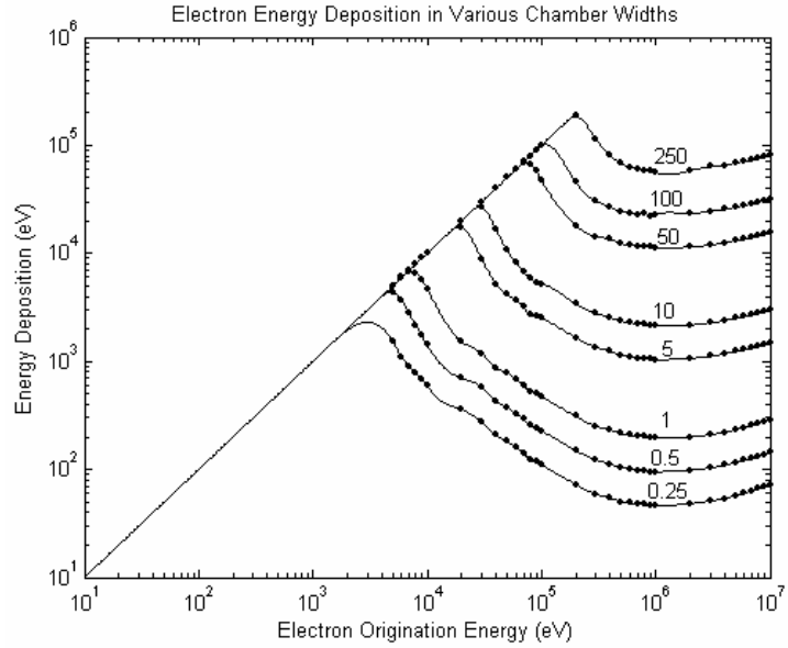
Figure 3.5: Data (dots) and spline fit (lines) of gamma-ray energy deposition in various chamber widths of argon gas.
