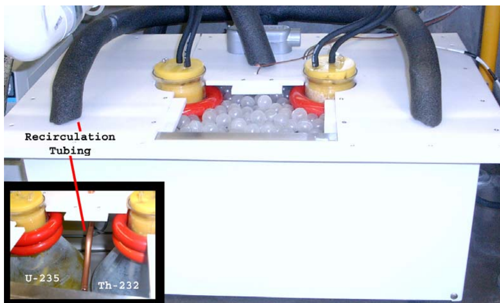
Figure 7.9: Hot water bath with uranium and thorium electrolytic solutions loaded.
