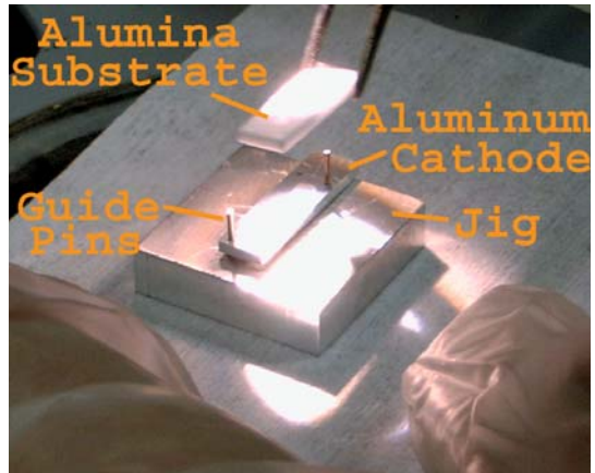
Figure 4.8: Manufactured 3-chamber alumina substrates and aluminum backing plate being assembled using a guide pin jig.
