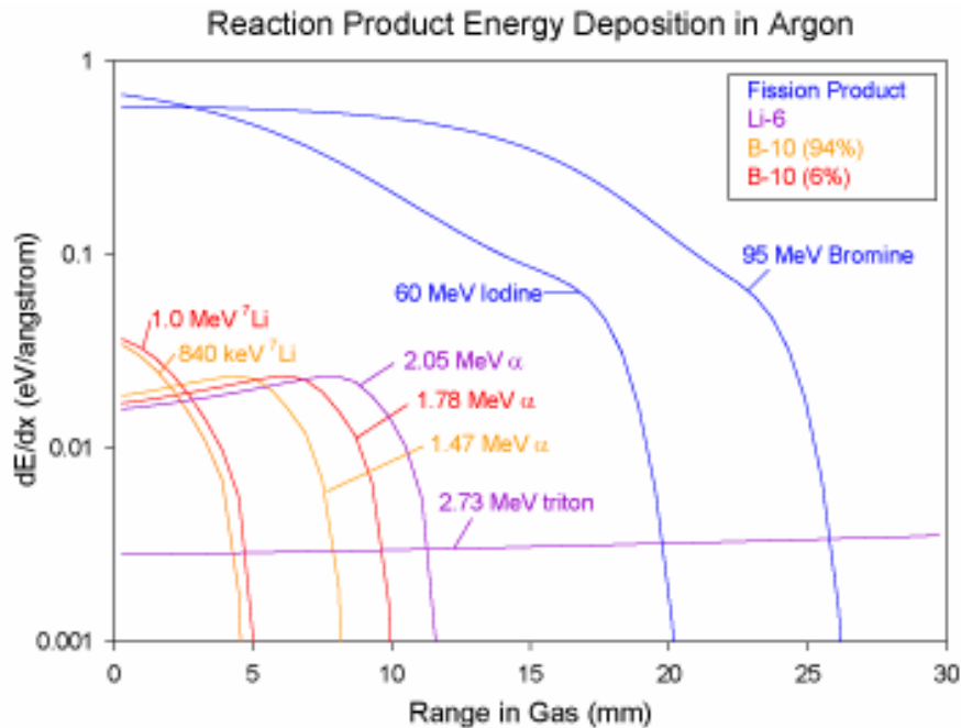
Figure 3.1: Energy deposition and range of neutron reaction products in argon fill gas at 1 atm.
