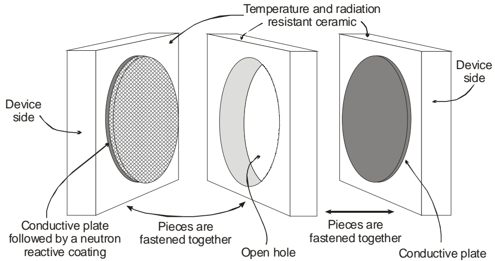
Figure 2.3: Basic construction method for fabricating MPFDs [13].
