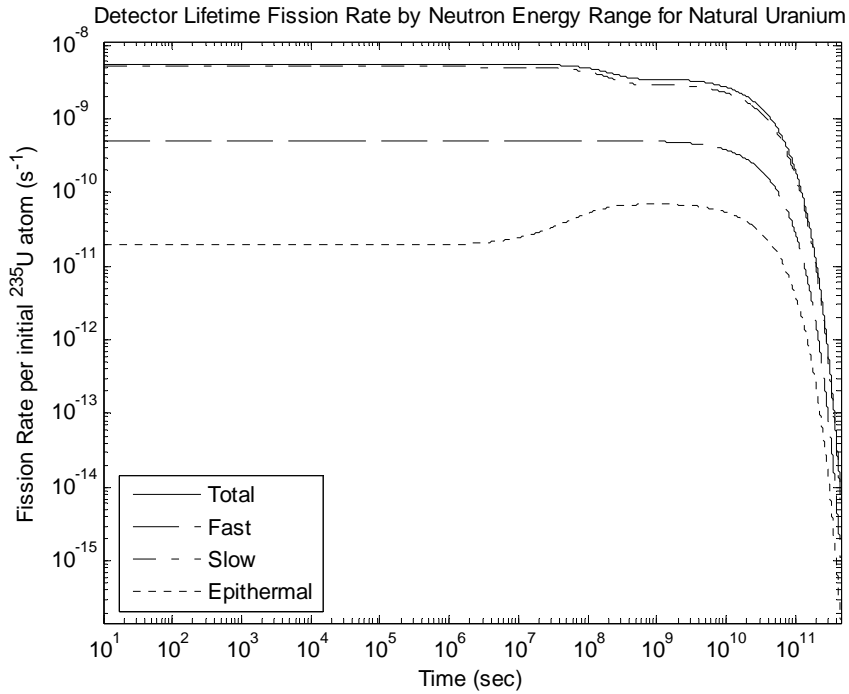
Figure 3.13: Detector lifetime fission rate by neutron energy range for natural uranium.
