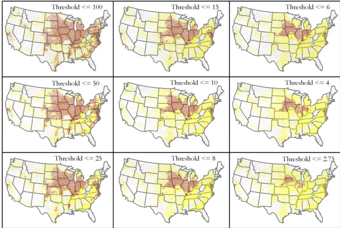
Supplemental Figure 1. Dropped edge analysis of the corn network. A threshold indicates the highest landscape resistance to transmission (LRT; defined in terms of host availability) that still allows dispersal by a particular pest or pathogen. Brown edges between counties meet the threshold criterion and yellow edges between counties have been “dropped” because the LRT is above the threshold being evaluated.
