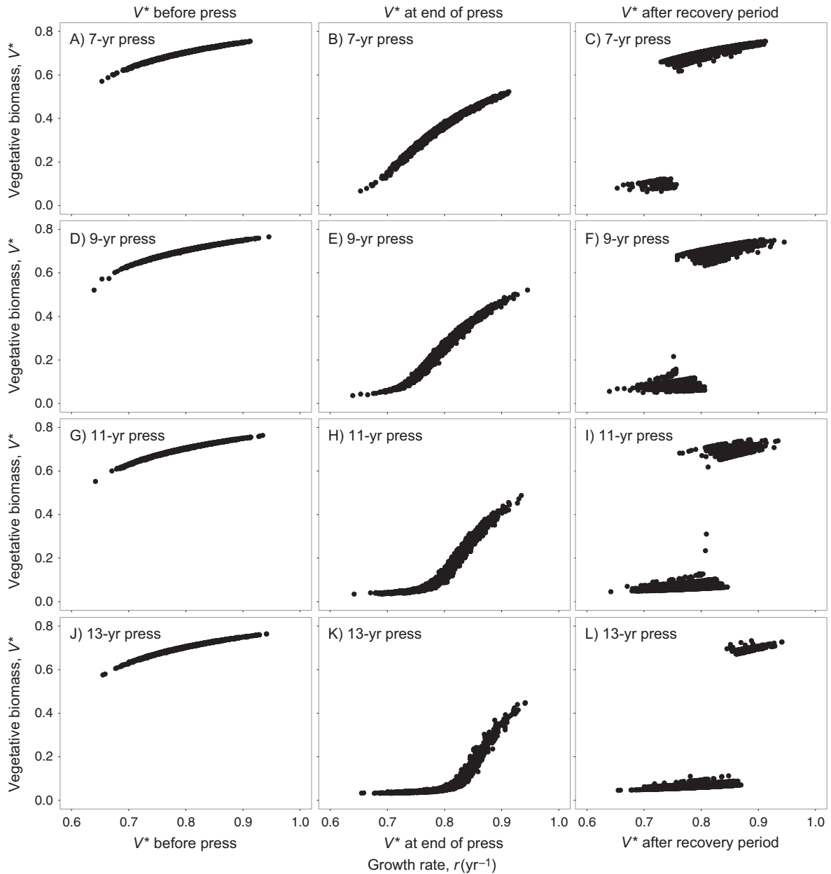
FIG. 8. Relationships between patch-scale vegetation growth rate, r ( \text{yr}^{-1} ), and vegetation biomass, V^* , in the spatially extended model. Each row is a single iteration of the spatially extended model, subjected to a press of the same moderate intensity as in Fig. 6 and varying durations of (A–C) 7, (D–F) 9, (G–I) 11, or (J–L) 13 years. The first column depicts V^* before the press is applied, the second column is V^* at the end of the press, and the third column is 100 years after the press ends. Each point is one of the 2500 patches.
