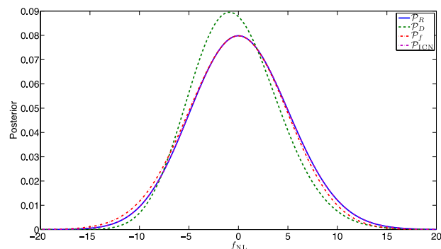
Figure 7. Analytic f_{\text{NL}} -posterior functions for an Euclid like survey combining all k -bins.
