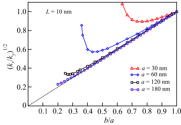
FIG. 6. The energetic ellipticity for L = 10 nm, as defined from the square root of the ratio of force constants, e = \sqrt{k_x/k_y} , versus geometric ellipticity \varepsilon = b/a .
