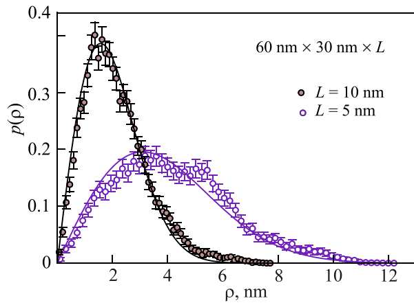
FIG. 9. Vortex core position radial distributions at T=300 K for semi-major axis a=60 nm, \varepsilon=0.5 for two disk thicknesses. Symbols are from Langevin LLG simulations out to dimensionless time \tau=2.5 \times 10^5 . Solid curves are the theoretical expression (73) with \bar{k}=4.299 \times 10^{-4} N/m for L=5.0 nm and \bar{k}=1.676 \times 10^{-3} N/m for L=10 nm, from relaxed vortex calculations. The T=0 gyrotropic periods were \tau_G \approx 2970 for L=5.0 nm and \tau_G \approx 1500 for L=10 nm.
