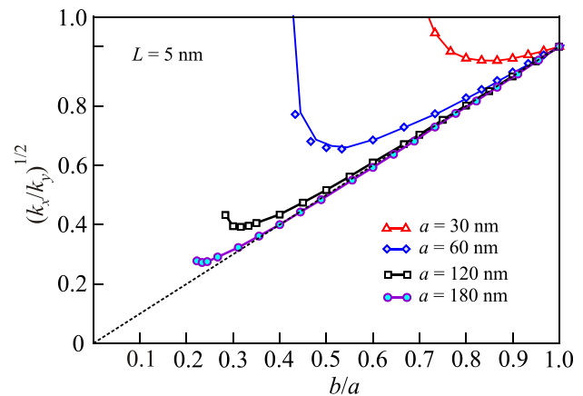
FIG. 5. The energetic ellipticity for L = 5.0 nm, as calculated from the square root of the ratio of forces constants, e = \sqrt{k_x/k_y} versus geometric ellipticity \varepsilon = b/a .
