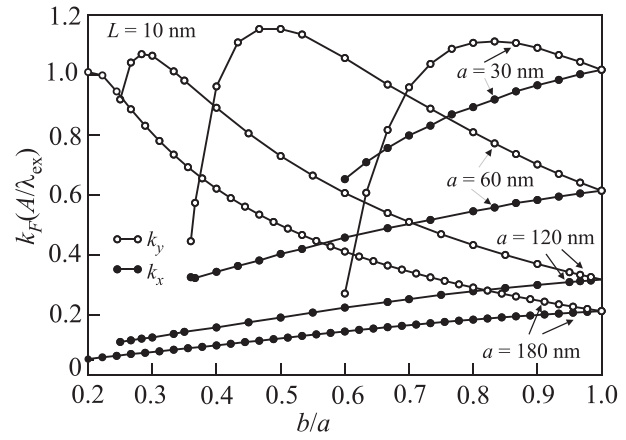
FIG. 3. Vortex force constants versus ellipticity ratio \varepsilon = b/a as in Fig. 1, but for film thickness L=10.0 nm. Note that larger thickness leads to higher force constants, roughly proportional to L^2 .
