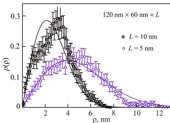
FIG. 10. Vortex core position radial distributions at T=300 K for semi-major axis a=120 nm, \varepsilon=0.5 for two disk thicknesses. Symbols are from Langevin LLG simulations out to dimensionless time \tau=2.5 \times 10^5 . Solid curves are the theoretical expression (73) with \bar{k}=2.667 \times 10^{-4} N/m for L=5.0 nm and \bar{k}=9.174 \times 10^{-4} N/m for L=10 nm, from relaxed vortex calculations. The T=0 gyrotropic periods were \tau_G \approx 4770 for L=5.0 nm and \tau_G \approx 2760 for L=10 nm. The \rho(\tau) used to produce the curve for L=10 nm is displayed in Fig. 11.
