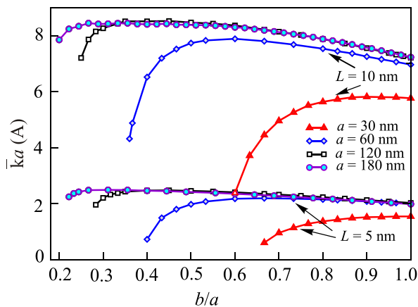
FIG. 4. The geometric mean of force constants, \bar{k} = \sqrt{k_x k_y} , scaled by semi-major axis a , in units of the exchange stiffness A , versus geometric ellipticity \varepsilon = b/a .
