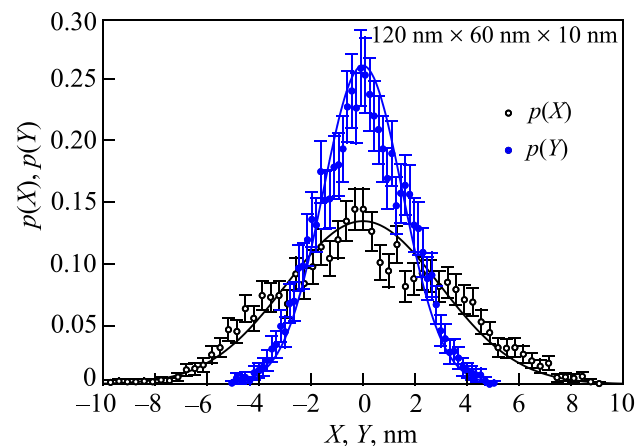
FIG. 12. Vortex core linear distributions along the major axes at T=300 K for semi-major axis a=120 nm, \varepsilon=0.5 , thickness L=10 nm. Symbols are from Langevin LLG simulations to time \tau=2.5 \times 10^5 . Solid curves are from theoretical expression (77) with k_x=4.696 \times 10^{-4} N/m and k_y=1.792 \times 10^{-3} N/m, from relaxed vortex calculations.
