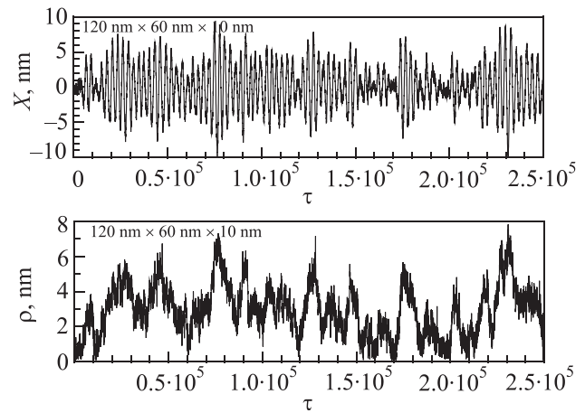
FIG. 11. Vortex core motion for thermalized dynamics at T=300 K for semi-major axis a=120 nm, \varepsilon=0.5 , thickness L=10 nm. Graphs of X(\tau) and Y(\tau) are very similar, but of different amplitudes. The resulting equivalent circular radius \rho(\tau) was used to produce the corresponding probability p(\rho) in Fig. 10.
