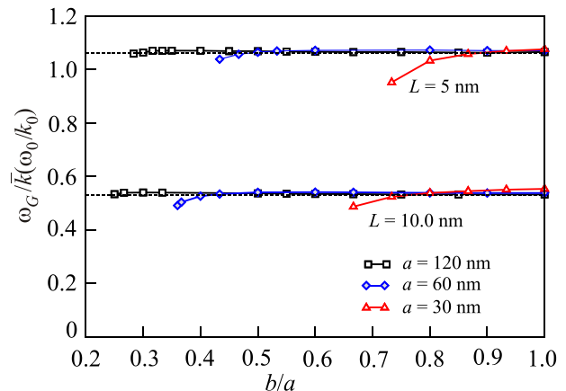
FIG. 8. Vortex gyrotropic angular frequencies from zero-temperature simulations divided by force constants \bar{k} from Lagrange constrained vortex relaxation, as a function of ellipticity \varepsilon = b/a . The frequency unit is \omega_0 \equiv (\mu_0 \gamma M_s)/4\pi , the force constant unit is k_0 \equiv a/\lambda_{\text{ex}} . Dashed lines are the theoretical result (64) based on the Thiele equation dynamics, where \omega_G/\bar{k} \propto \lambda_{\text{ex}}/L .
