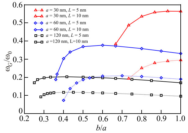
FIG. 7. Vortex gyrotropic angular frequencies calculated from simulations of zero-temperature dynamics, for the indicated nanodisk sizes. The frequency unit is \omega_0 \equiv (\mu_0 \gamma M_s)/4\pi (about 15.1 GHz for Permalloy).
