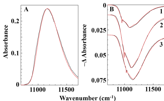
FIG. 4. Experimental data 8 (black curves) from Figure 2 fit with a lognormal J(\omega) (red curves). The parameters obtained from simulations are reported in Table II. Frame (a) is the absorption spectrum and frame (b) shows transient HB spectra with \omega_B = 10\,953 , 10\,992 , and 11\,030 for curves 1–3, respectively.
