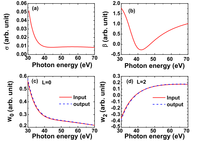
FIG. 2. Retrieval of the radial matrix elements from IR-free photoelectron angular distributions. (a) Input total cross section \sigma_{\text{total}} . (b) Input \beta parameter. (c) Input and retrieved radial matrix element W_0 . (d) The same but for W_2 . The phase difference between the two partial waves vs photon energy from the input and from the retrieval also agree well (not shown).
