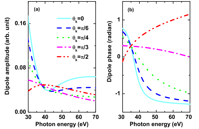
FIG. 1. Angular dependence of single-photon dipole transition amplitude (a) and phase (b), d_0(E, \theta_k) , for the case of ionization from the m_i = 0 initial 3p state of Ar. They are calculated from Eq. (9) where the radial matrix element and phase for the two partial waves L = 0 and 2 are obtained from solving the time-independent Schrödinger equation.
