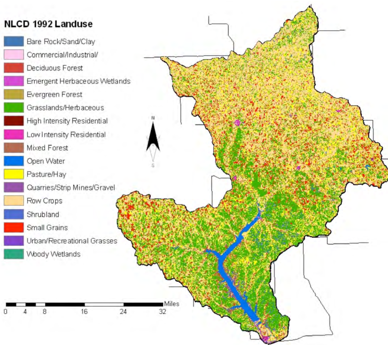
Figure 7. NLCD 1992 land use classification.
