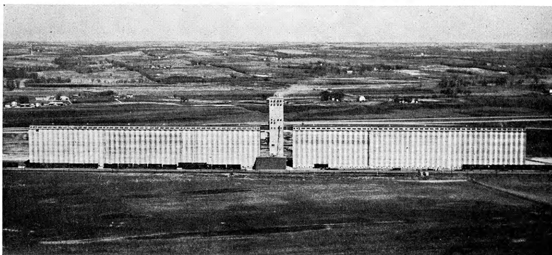
FARMERS UNION WEST TERMINAL ELEVATOR IN TOPEKA
