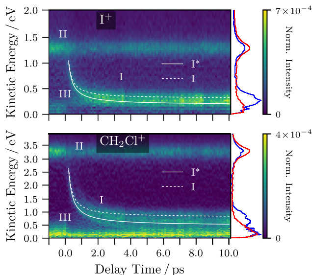
FIG. 6. Kinetic energy distributions as a function of pump-probe delay for the \text{I}^+ (top) and \text{CH}_2\text{Cl}^+ (bottom) ions, obtained from PBASEX Abel inverted ion images. The kinetic energy spectrum for delays of +9.9 ps to +10.1 ps is projected to the right of each panel in blue. The kinetic energy spectrum for delays of -1.0 ps to -0.8 ps, in which the IR probe pulse arrives first, is projected in red. Simulated curves for the \text{I}^*(^2\text{P}_{1/2}) ( \text{I}^* , white solid line) and \text{I}(^2\text{P}_{3/2}) ( \text{I} , white dashed line) dissociation pathways are superimposed over the experimental data. These were modelled by assuming the fragments were instantly accelerated to their final velocities following neutral photodissociation, as described in the main text.
