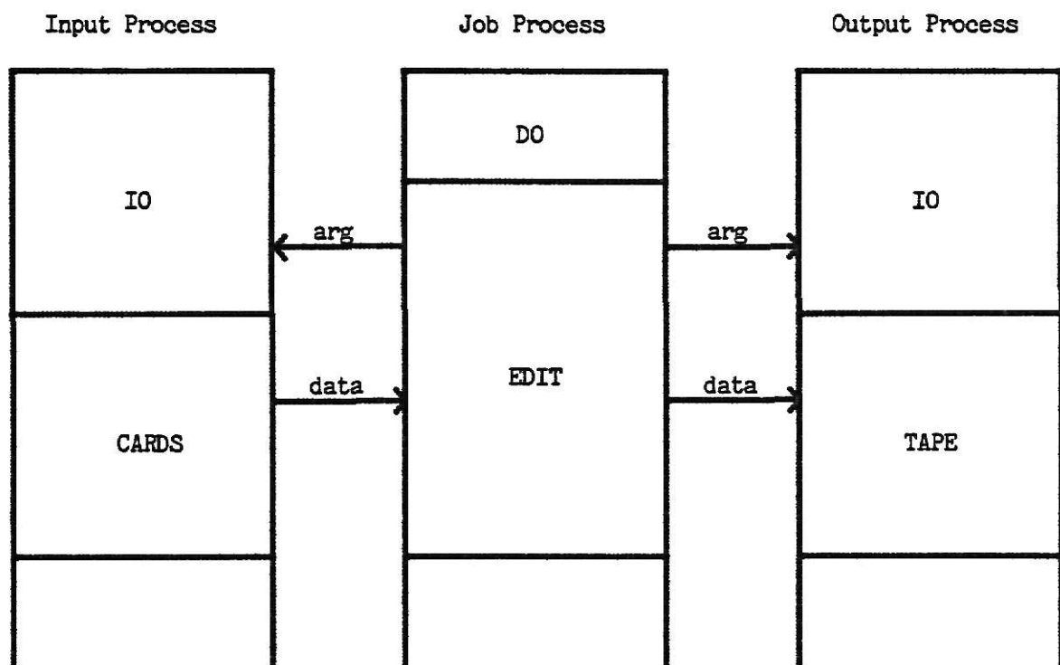
Figure 9. Execution of EDIT(CARDS,TAPE).
