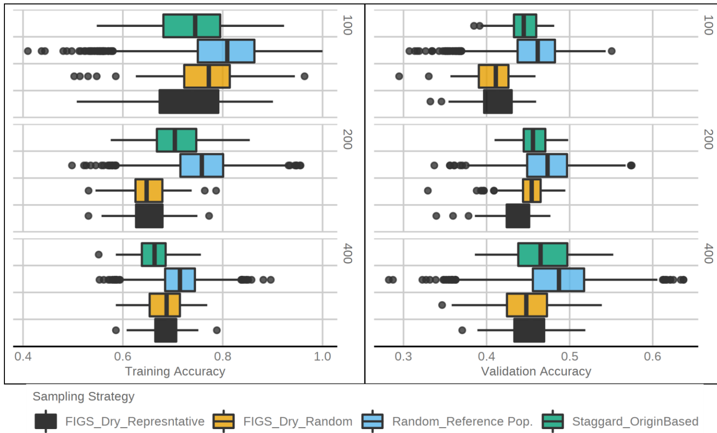
Figure 3-5 Training and validation accuracy of genomic prediction computed using reference populations assembled through different sampling approaches.
