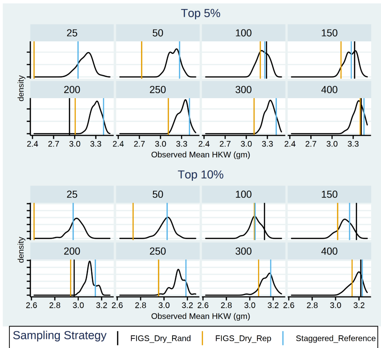
Figure 3-6 Mean HKW of top 5% and 10% lines selected based on GEBVs computed using different sampling strategies.
