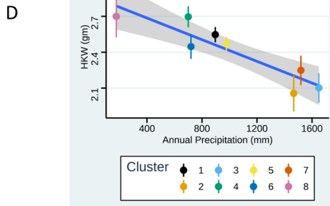
Figure 3-2 FIGS based selection of landraces: (A) Determination of optimum number of clusters (B) Group size and mean precipitation of the clusters. (C) The distribution of the clusters along precipitation gradient and PCs. (D) Relationship of cluster mean HKW and annual precipitation.
