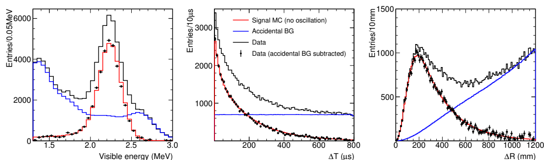
Figure 3. Input variables to ANN: E_{\text{delayed}} (left), \Delta T (centre) and \Delta R (right) for the IBD signal MC (red), accidental background from off-time coincidences (blue) and the on-time data before (black histogram) and after (points) subtraction of the accidental background.
