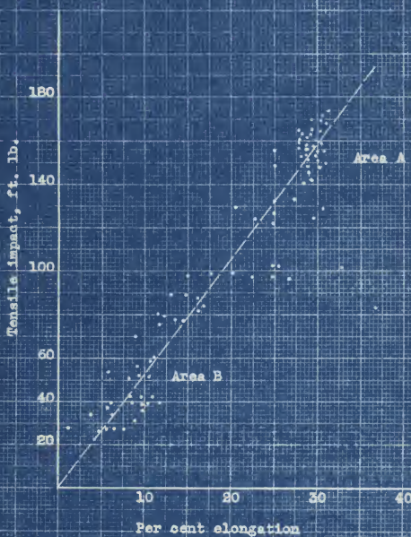
Fig. 4. Showing relationship between parent metal failures (Area A), and weld metal failures (Area B).
