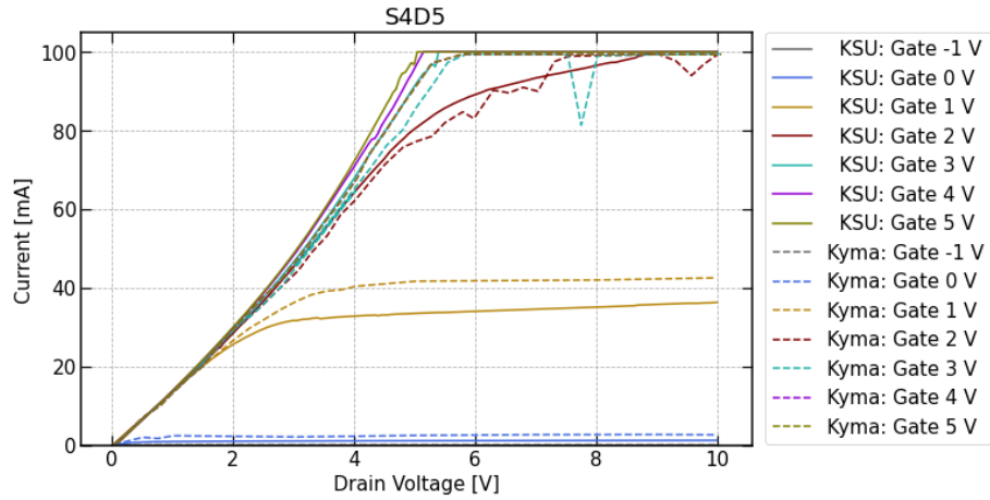
Figure 5.9: Comparison of fabricated GaN FinFET S4D5 measured family of curves.
