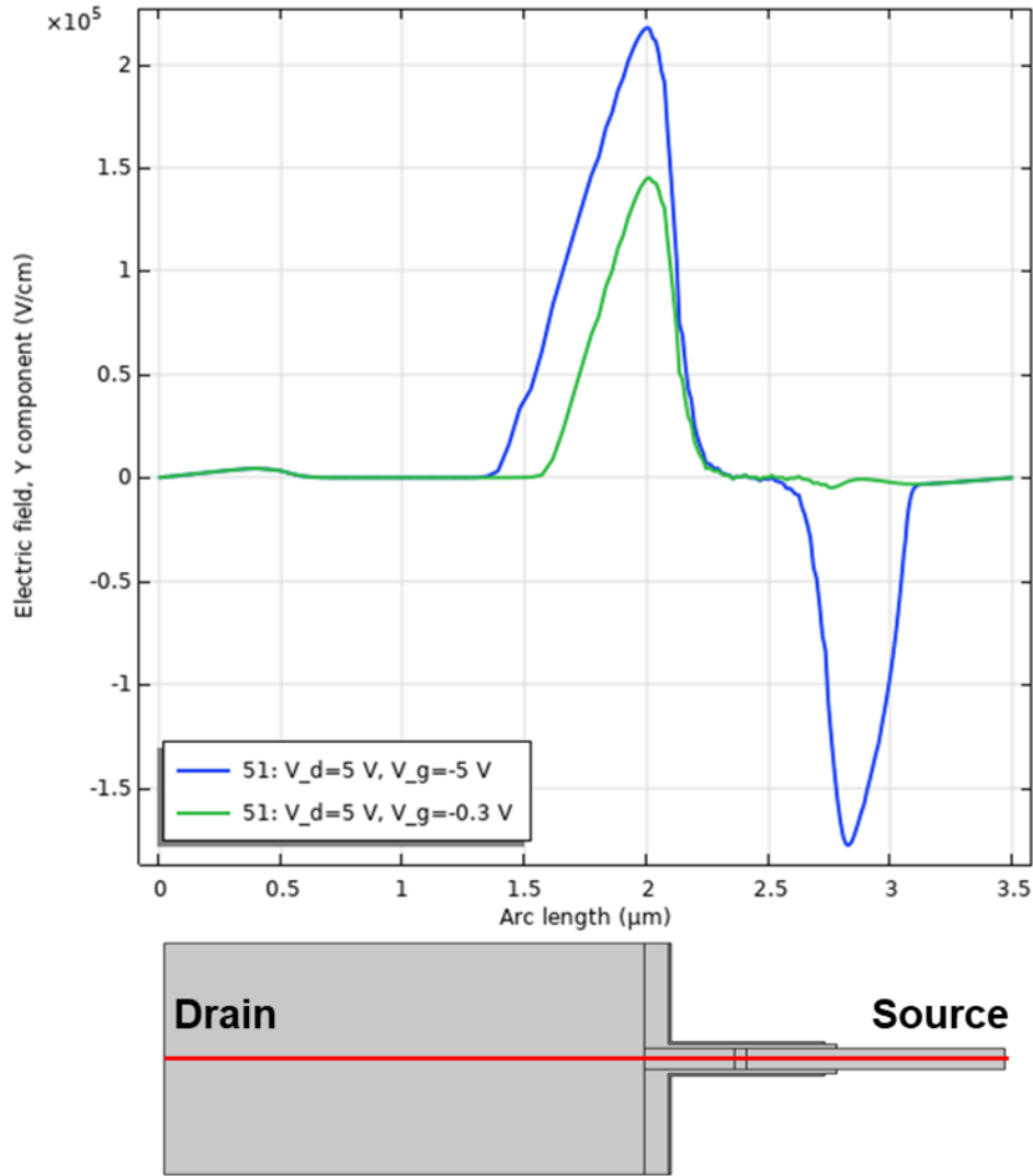
Figure 5.13: Comparison of y -component of electric field down center cutline of GaN Fin-FET simulation for gate bias of -0.3\text{ V} and -5\text{ V} , with a constant drain bias of 5\text{ V} . Arc length of 0\text{ }\mu\text{m} corresponds to bottom (drain) of the device and arc length of 3.5\text{ }\mu\text{m} corresponds to the top (source) of the device.
