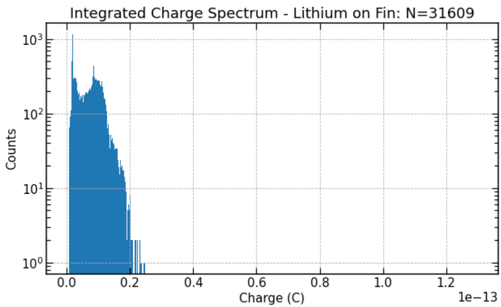
Figure 5.24: Integrated charge spectrum including only lithium ions incident on fin edge. The value of N represents the number of times the particles were incident on the GaN surface– the total number of source thermal neutrons simulated was 5,517,789.
