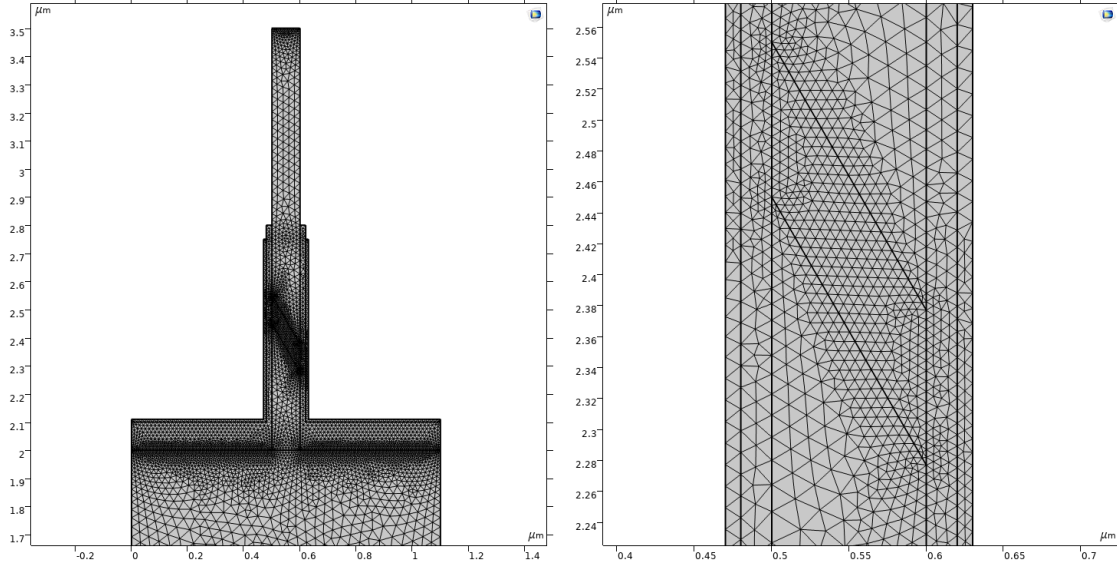
Figure 4.2: The meshing used for time-dependent solutions, zoomed out (left) and focused on the generation domain (right).
