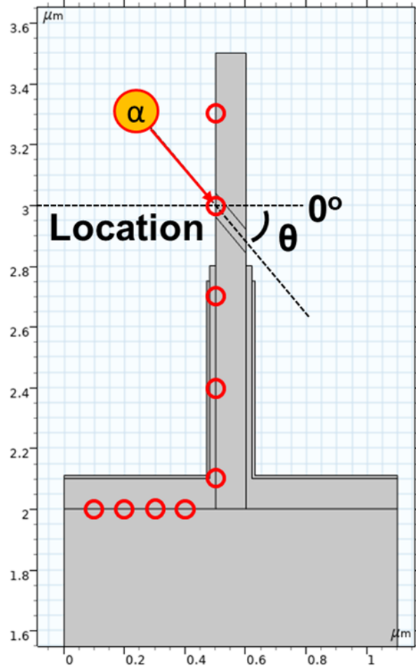
Figure 5.14: Location of where incident particles are simulated in COMSOL. Note the angles given are referenced according the perpendicular of the side of the fin edge.
