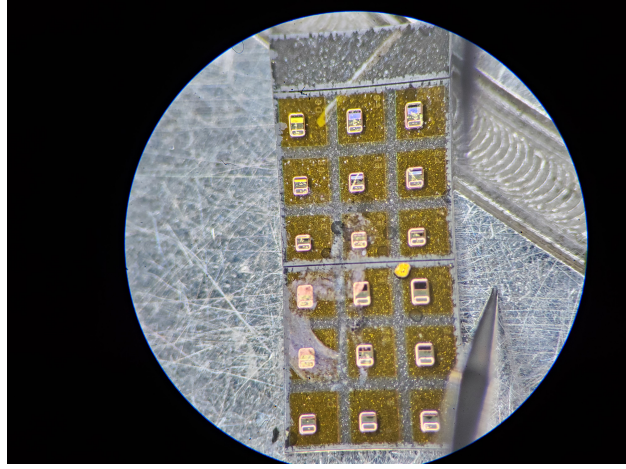
Figure 1.4: Kyma Technologies FinFET devices under probe station microscope.
