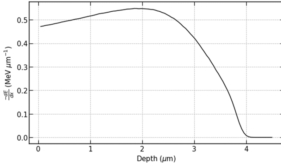
Figure 4.3: Bragg curve for 1777 keV alpha particle traveling through GaN, calculated from SRIM/TRIM.
