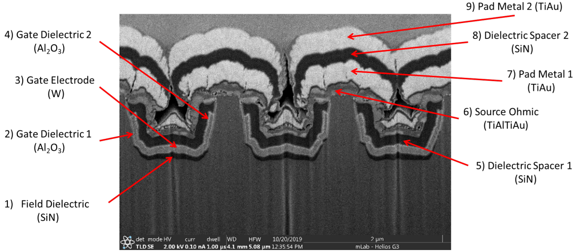
Figure 1.5: Cross-section image of fabricated GaN FinFETs, with material annotations 2 .
