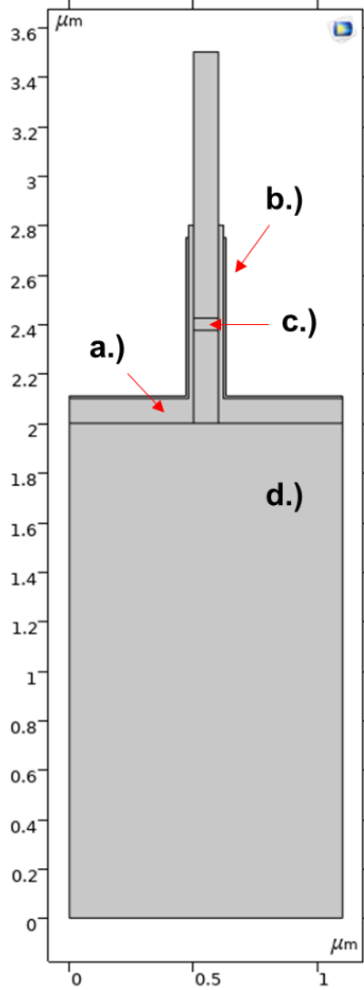
Figure 4.1: COMSOL model of 2D GaN vertical FinFET. This model includes the gate dielectric material (a), conducting semiconductor material layer (b) in order to use metal gate contact physics, the GaN charge generation domain (c), and the remaining GaN domains (d) of the device.
