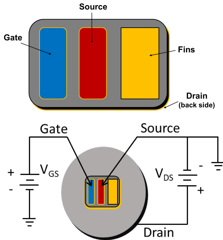
Figure 3.2: Illustration of wiring schematic for testing of fabricated FinFET devices 2 .
