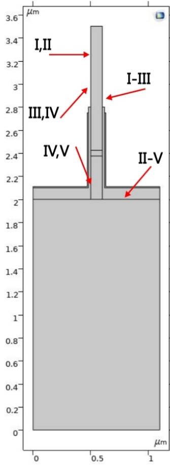
Figure 5.26: Illustration of common alpha particle incident locations and which region of the spectrum they contribute to (see Fig. 5.22), including particles incident on the trench.
