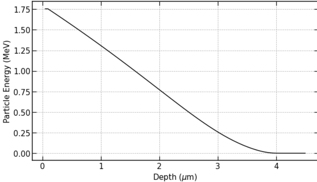
Figure 4.4: Cumulative Bragg curve for 1777 keV alpha particle traveling through GaN, calculated from SRIM/TRIM and numerically calculated using Python.
