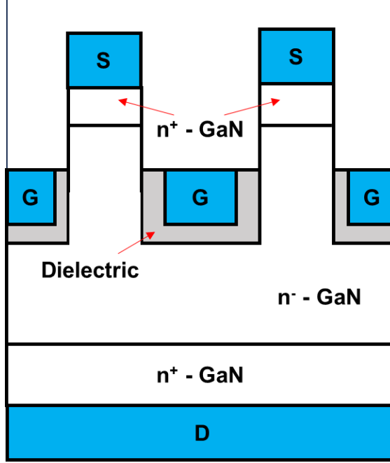
Figure 1.1: Illustration of FinFET device geometry, where S is the source contact, G is the gate contact, and D is the drain contact 1 .
