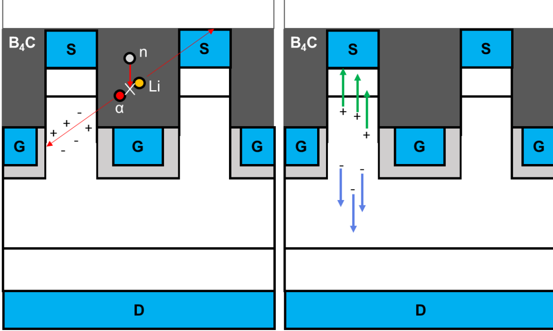
Figure 1.3: Illustration of FinFET device geometry with neutron conversion material B_4C . The neutron will be captured by ^{10}B and emit an alpha and lithium ion in opposite directions, where they will ionize the GaN FinFET and be detected.
