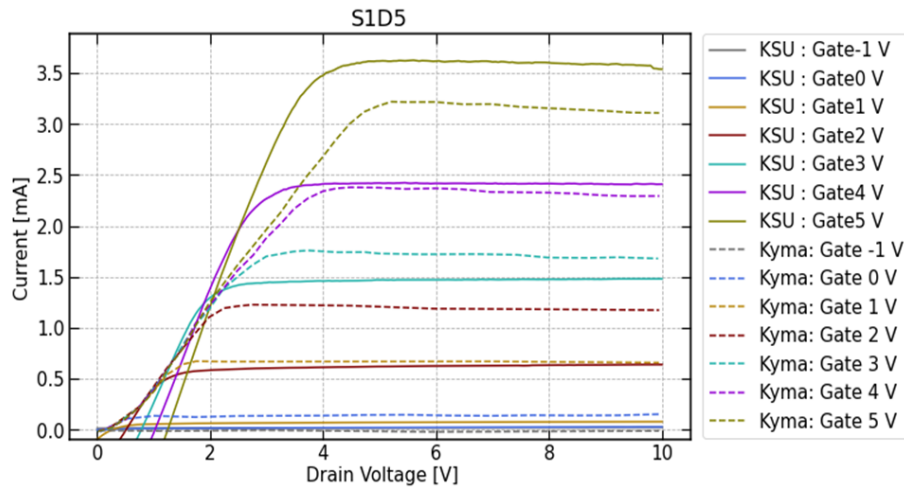
Figure 5.7: Comparison of fabricated GaN FinFET S1D5 measured family of curves.
