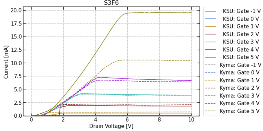
Figure 5.8: Comparison of fabricated GaN FinFET S3F6 measured family of curves.
