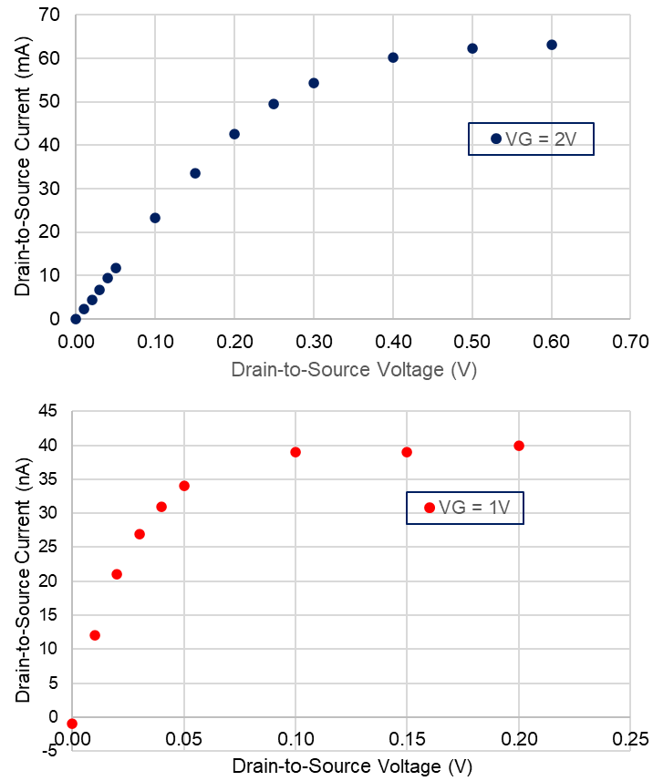
Figure 3.1: Current-voltage curves for MOSFET IRL520N to ensure equipment was working properly.
