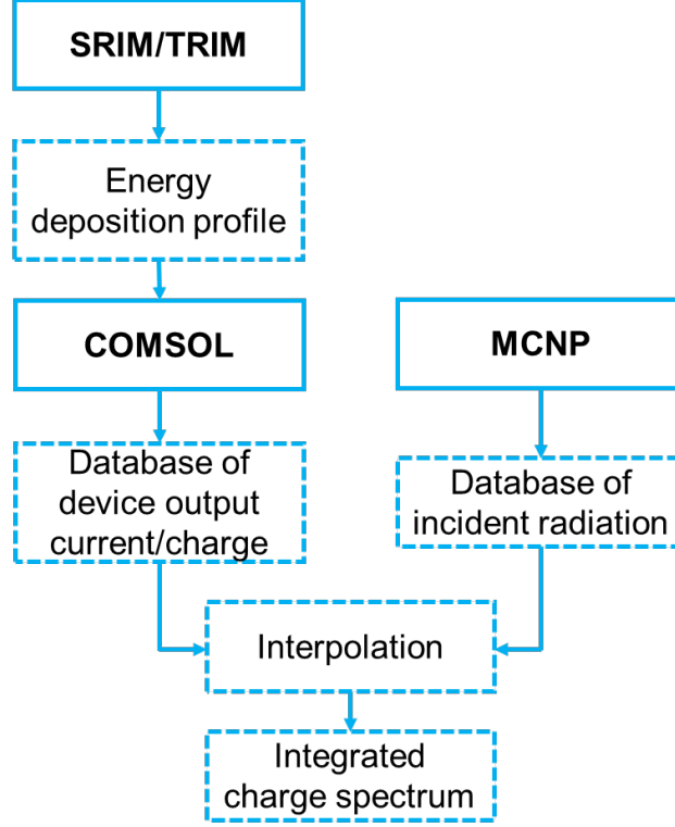
Figure 1.2: Flowchart of simulation framework used to analyze radiation detection device.
