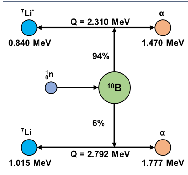
Figure 1.6: Reaction products from n-alpha reaction 3 .
