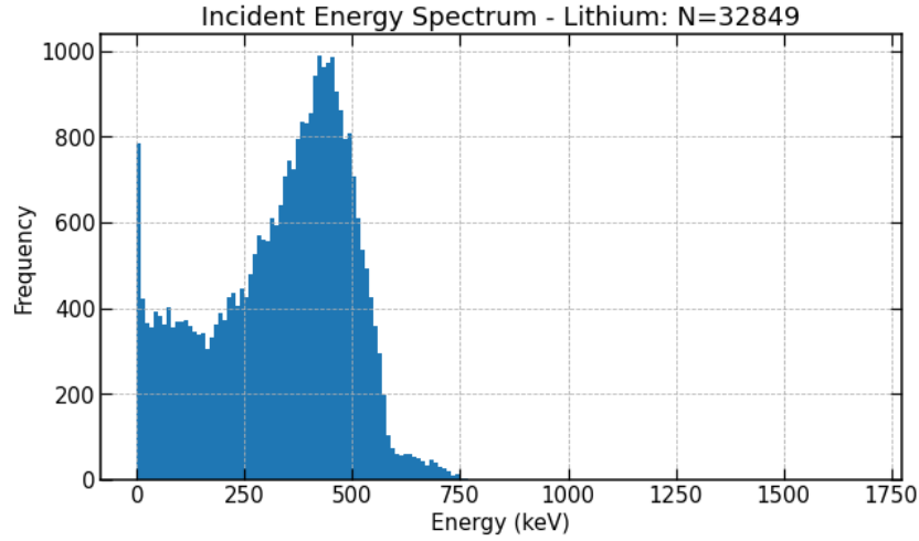
Figure 5.2: Histogram of energy values of lithium ions incident on GaN.
