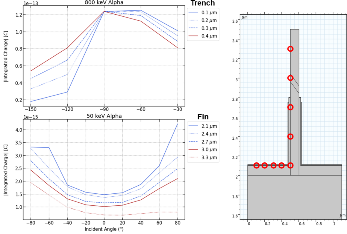
Figure 5.17: Angular interpolated integrated charge values for 50 keV and 800 keV alpha particle incident on the fin edge and trench base respectively.
