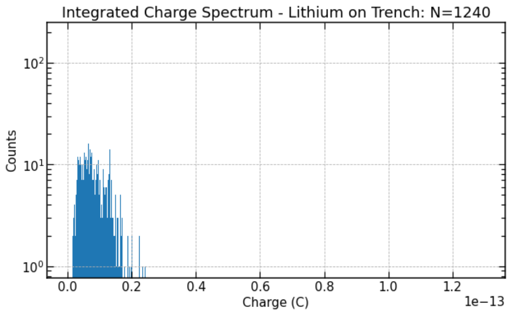
Figure 5.25: Integrated charge spectrum including only lithium ions incident on base of trench. The value of N represents the number of times the particles were incident on the GaN surface– the total number of source thermal neutrons simulated was 5,517,789.
