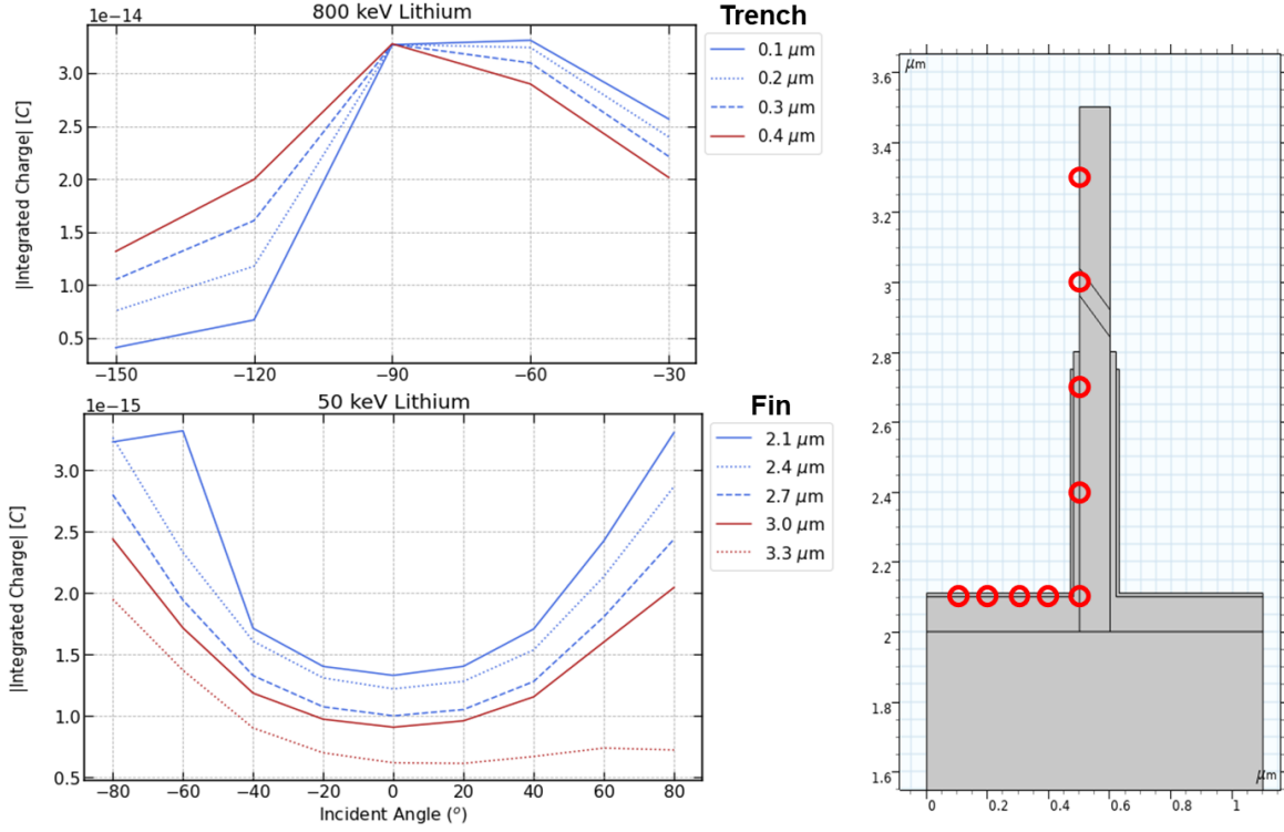
Figure 5.18: Angular interpolated integrated charge values for 50 keV and 800 keV lithium ion incident on the fin edge and trench base respectively.
