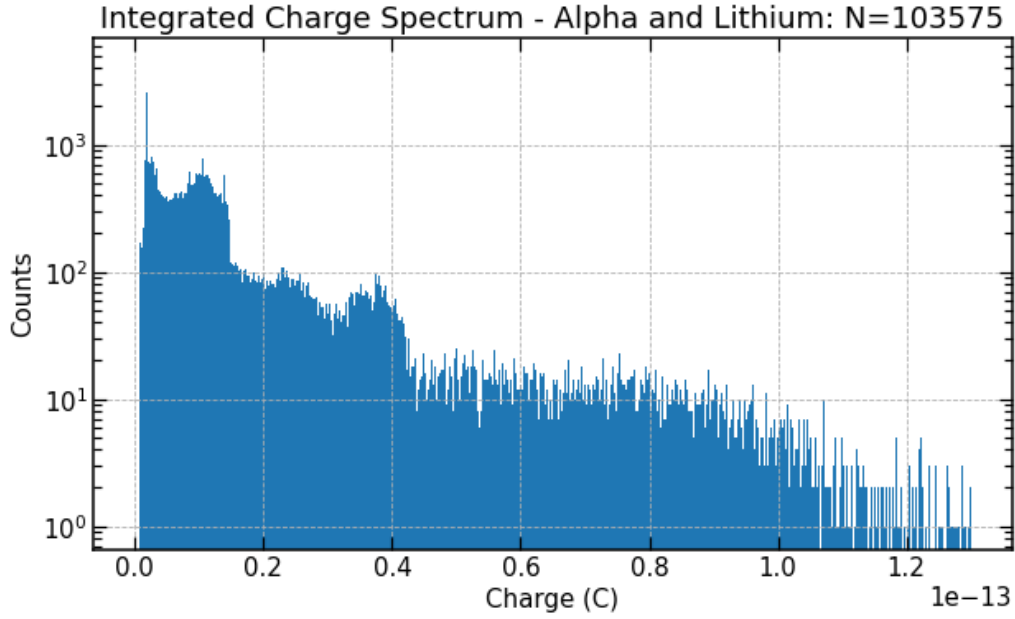
Figure 5.19: Integrated charge spectrum including alpha particles and lithium ions. The value of N represents the number of times the particles were incident on the GaN surface—the total number of source thermal neutrons simulated was 5,517,789.
