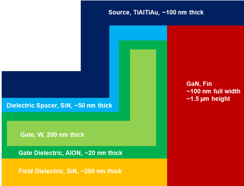
Figure 2.2: Illustration of half of FinFET model materials and dimensions. Not to scale.
