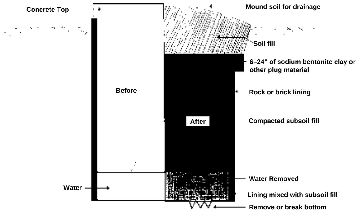
Figure 1. Plugging diagram for cistern, cesspool or septic tank.
