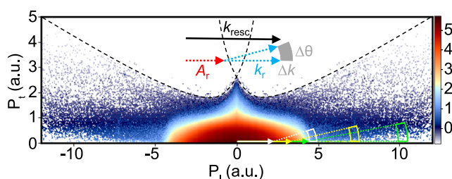
FIG. 1. FT-LIED extraction. Two-dimensional map of the longitudinal, P_{\parallel} , and transverse, P_{\perp} , momenta given in atomic units (a.u.). The return momentum, k_r , at the instance of rescattering is obtained by subtracting the vector potential, A_r , from the detected rescattered momentum, k_{\text{resc}} , given by k_r = k_{\text{resc}} - A_r . The energy-dependent interference signal is extracted at various different vector potential kicks (see white, yellow, and green arrows along P_{\perp} = 0 ) by integrating the area indicated by a block arc. A schematic is drawn at the top of the figure relating k_{\text{resc}} (black arrow), k_r (blue arrows), A_r (red arrow), and the integrated area indicated by the gray shaded block arc corresponding to a small range of rescattering angles and momenta, \Delta\theta and \Delta k , respectively. We use \Delta\theta_r and \Delta k_r values of 10^\circ and 0.2 a.u., respectively. The dotted black lines represent the detection acceptance angle of the reaction microscope. 28
