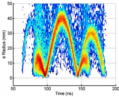
FIG. 10. (Color online) Detected electron radius vs time of flight. The radius is defined as the distance from the center of detector. The nodes are characteristic of the magnetic field and can be used to determine its value
