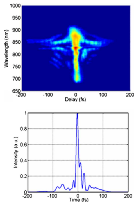
FIG. 16. (Color online) (Top) Sample GRENOUILLE trace of the pulse after spectral broadening in the SPM waveguide and recompression with the chirped mirrors. (bottom) Reconstruction of the temporal profile of the pulse from the GRENOUILLE trace by using a standard FROG algorithm showing a 10–12 fs pulse.
