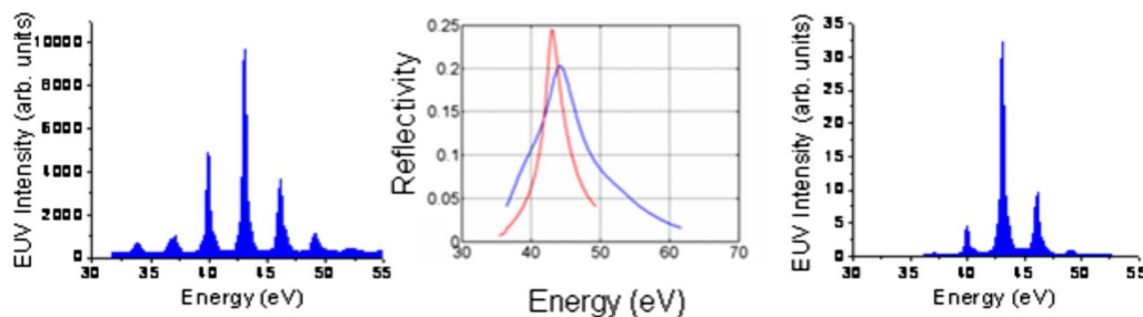
FIG. 3. (Color online) (Left) Sample EUV spectrum obtained with a 30 fs driving laser pulse. The emission consists of a comb of harmonics centered at \sim 43 eV. (Middle) Reflectivity of Mo/Si multilayered mirror as a function of photon energy for a single reflection. The blue curve is a broadband reflection. The red curve is narrow-band reflection. (Right) Sample spectrum of the EUV beam after two reflections from the multilayer narrow-band EUV mirrors used in the experiments described herein.
