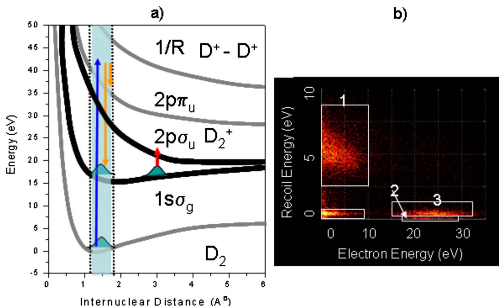
FIG. 13. (Color online) Correlation data for two-color EUV/IR excitation and ionization of the D_2 molecule. (a) The potential energy diagram for D_2 molecule showing ground state, D_2^+ ground and excited states and D_2^{2+} state. The EUV pulse is represented by the long upward blue arrow. The detected electron energy associated with populating a particular state is shown by the downward orange arrows. The IR ionization is represented by the short upward red arrow. (b) The ion-energy/electron-energy correlation map obtained by using the reaction microscope, showing different channels.
