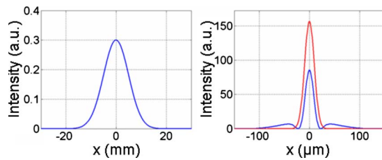
FIG. 5. (Color online) Computed profile of IR beam focused into the sample chamber, after reflection from the beam recombining mirror with a 3 mm hole in the center. (Left) IR beam as a 1/e^2 radius of 10 mm before the 75 cm lens. (Right: red) Focal spot inside the detector using a regular mirror (without a hole in the center). (Right: blue) Focal spot when mirror with a hole is used in the beam bath.
