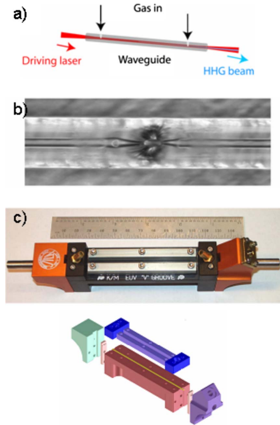
FIG. 2. (Color online) (a) Schematic of the three section EUV waveguide. Two gas inlets allow a constant pressure to be maintained in the center region while the end sections are differentially pumped. (b) Microscope image of laser-created hole in EUV waveguide. The inner capillary is left minimally deformed by the hole. The hourglass shape seen in the picture is due to the lensing effect of the melted outer wall of the capillary. (c) Picture of a HHG waveguide V-groove holder engineered to ensure good mode propagation and low loss. The middle section can be changed to allow different length waveguides to be used.
