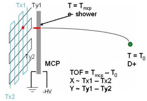
FIG. 11. (Color online) Schematic of the charged fragment detection and momentum calculation. Ionization event occurs at T_0 . The charged particle reaches the MCPs at time T_{MCP} . The MCPs generate an electron shower that is collected by a delay line detector behind it. A current pulse is formed and detected at each end of each wire with times T_{x1} and T_{x2} (for one wire/layer) and with times T_{y1} and T_{y2} (along the other wire/layer). P_z , P_y , and P_x can then be obtained from TOF, T_{y1}-T_{y2} , and T_{x1}-T_{x2} , respectively.
