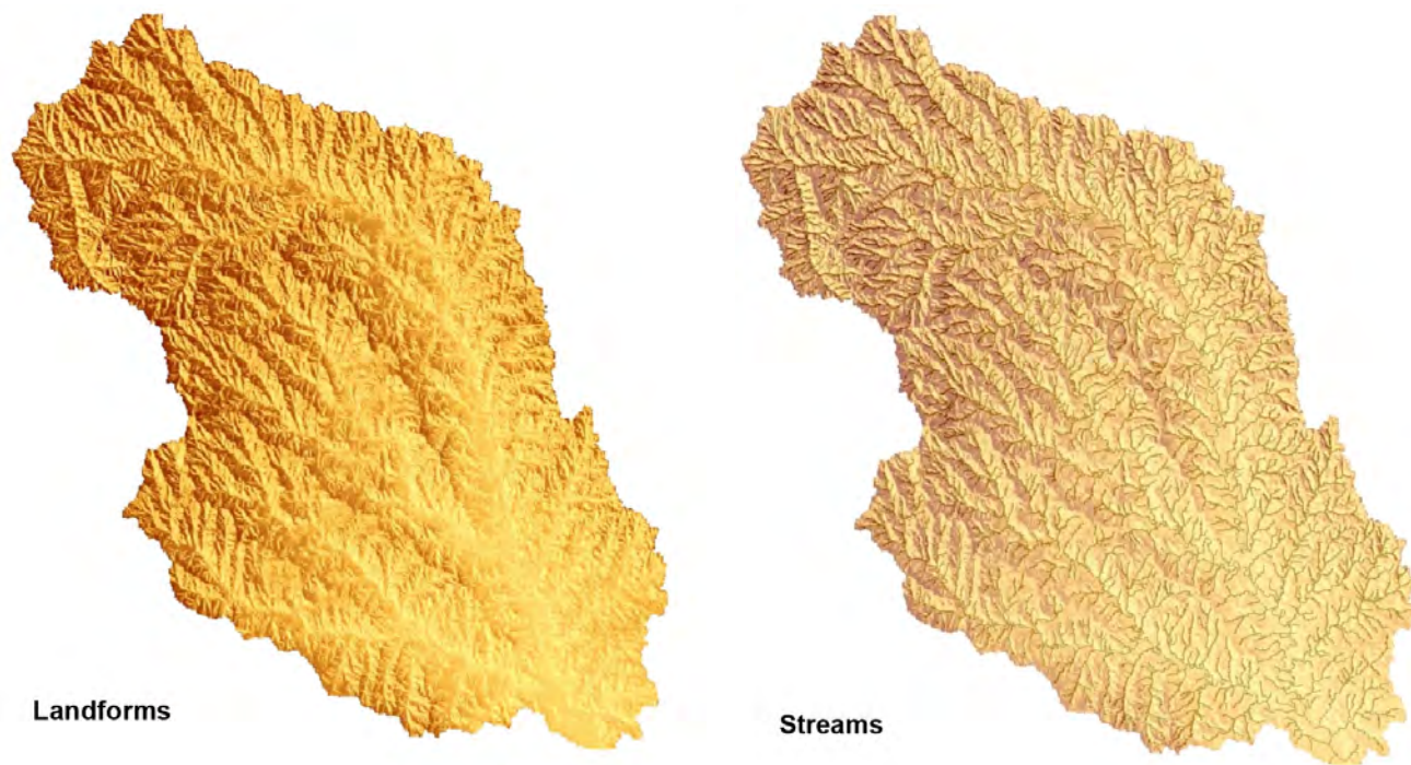
Figure 2. Relief Maps – Toronto Lake Watershed 3
