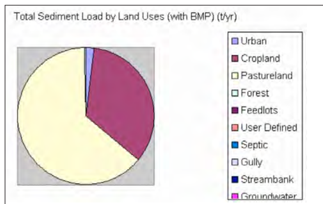
Figure 29. Total Load by Land Uses – Toronto Lake Watershed.
