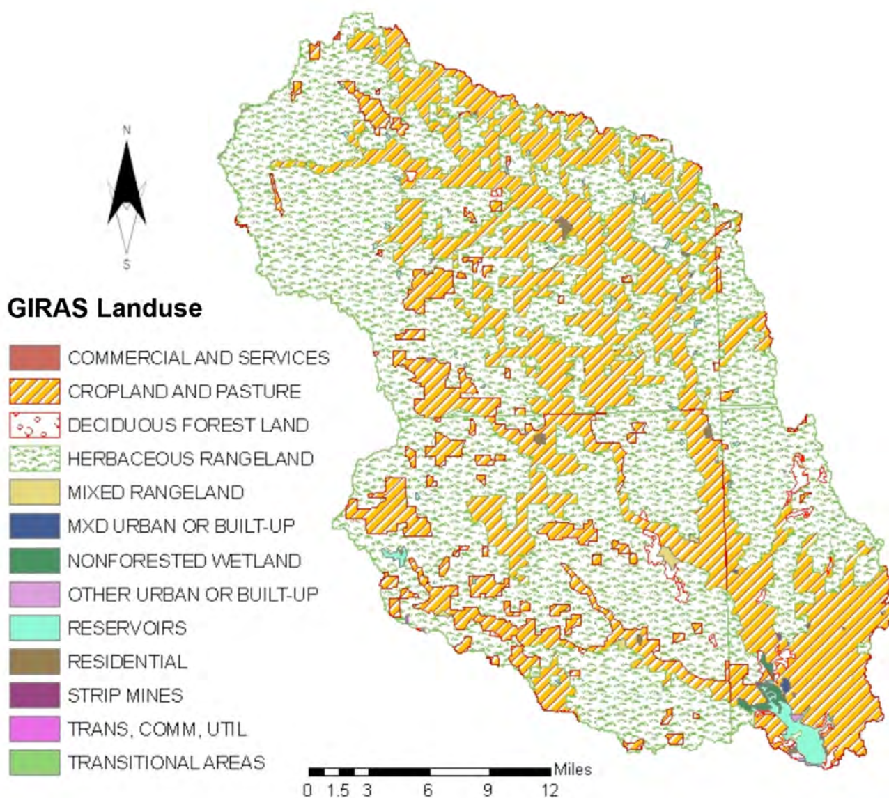
Figure 6. GIRAS 1980s land use classification.
