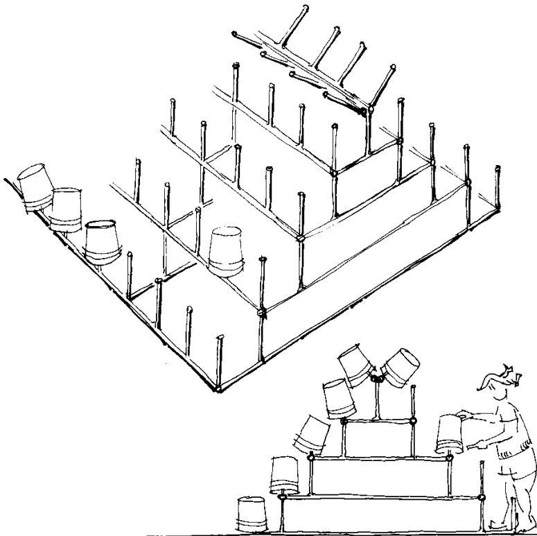
Figure 8. A Welded Pipe Rack for Storing Containers.
