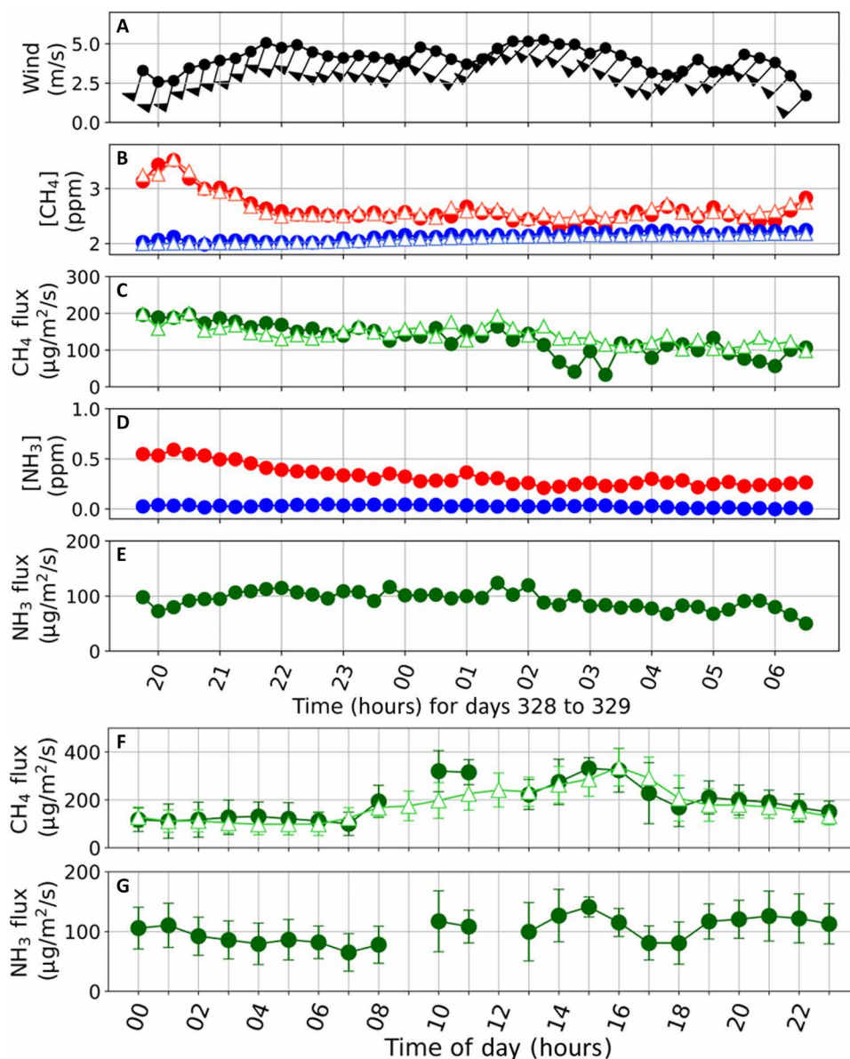
Fig. 4. Time-resolved \text{CH}_4 and \text{NH}_3 flux and averaged hourly diurnal flux cycles. Example dataset covering an 11-hour period showing (A) wind conditions at the measurement site, (B) \text{CH}_4 concentrations (averaged to 15-min time resolution) retrieved from the DCS (solid circles) and CRDS (open triangles) systems for north (red) and south (blue) paths, (C) the corresponding \text{CH}_4 flux retrieved from these DCS and CRDS measurements, (D) \text{NH}_3 concentrations from the DCS system, and (E) the corresponding \text{NH}_3 flux. The wind barbs point to the direction from which the wind is coming. (F) Diurnal cycle of \text{CH}_4 flux determined by DCS (solid circles) and CRDS (open triangles) when cattle were at the site (October 2019 to December 2019). Error bars are calculated by taking the SD of all 15-min averages included in each time bin. The increase in \text{CH}_4 flux between hours 8 and 16 is due to increased enteric fermentation after cattle feeding. (G) Diurnal cycle of \text{NH}_3 flux determined by DCS.
